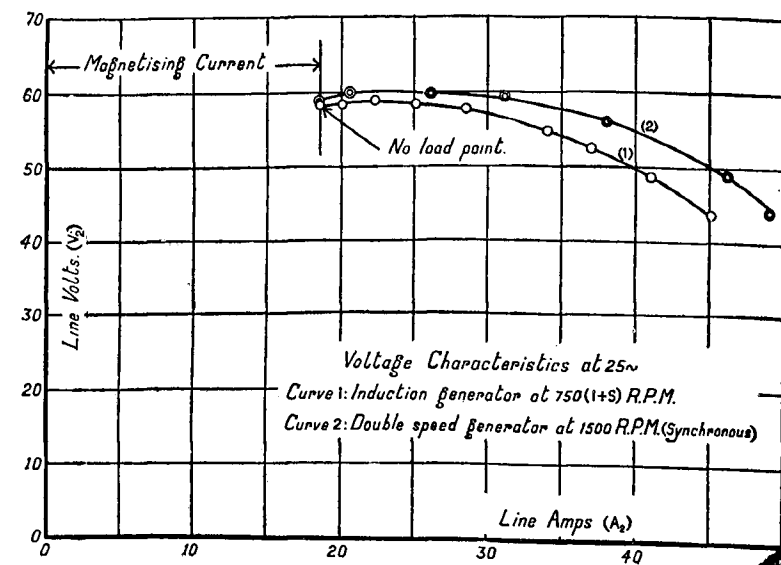
Fig 7. Terminal Voltage Characteristics
