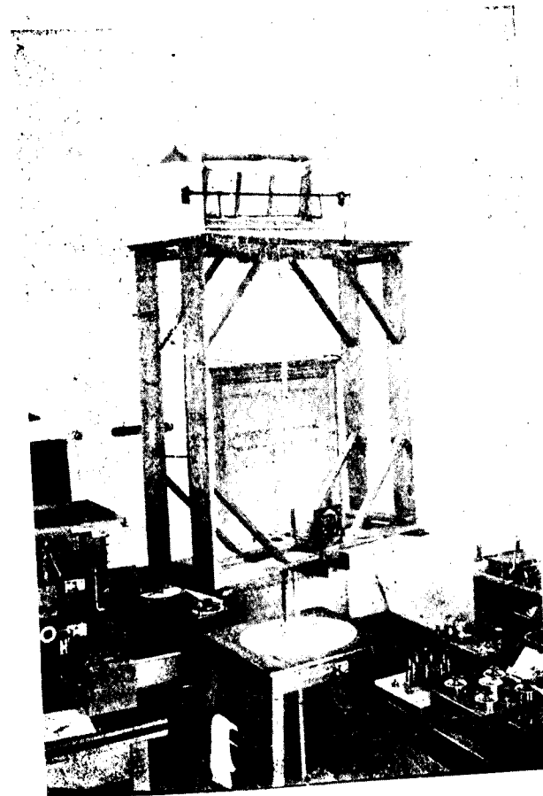
FIG. 3. COIL RECEIVER
