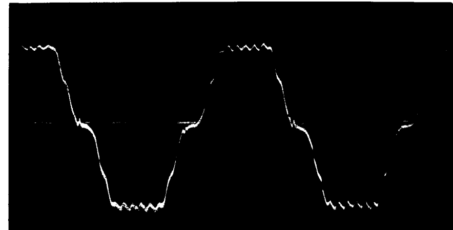
Plate 3. Current throughout coil a, machine running as generator on no load, 50 ohms in oscillograph circuit.
