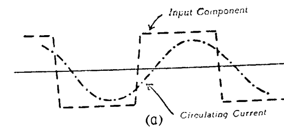
Fig. 9. Variation of Armature Current with Load.
