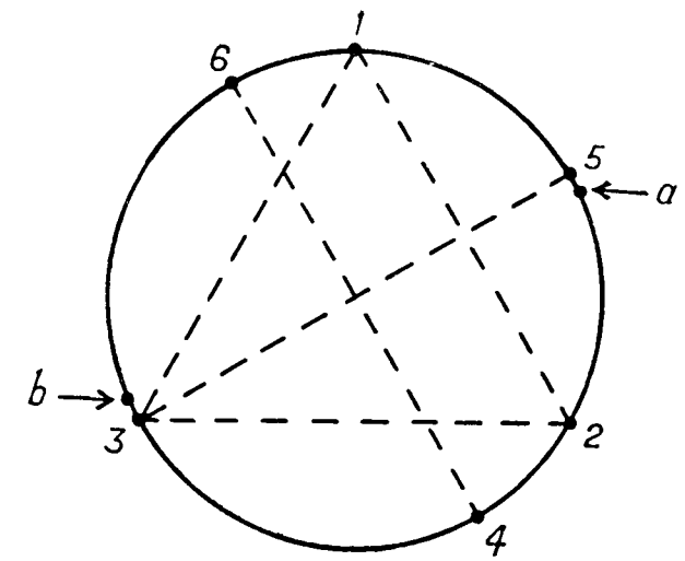
Fig. 1. Armature Diagram.
