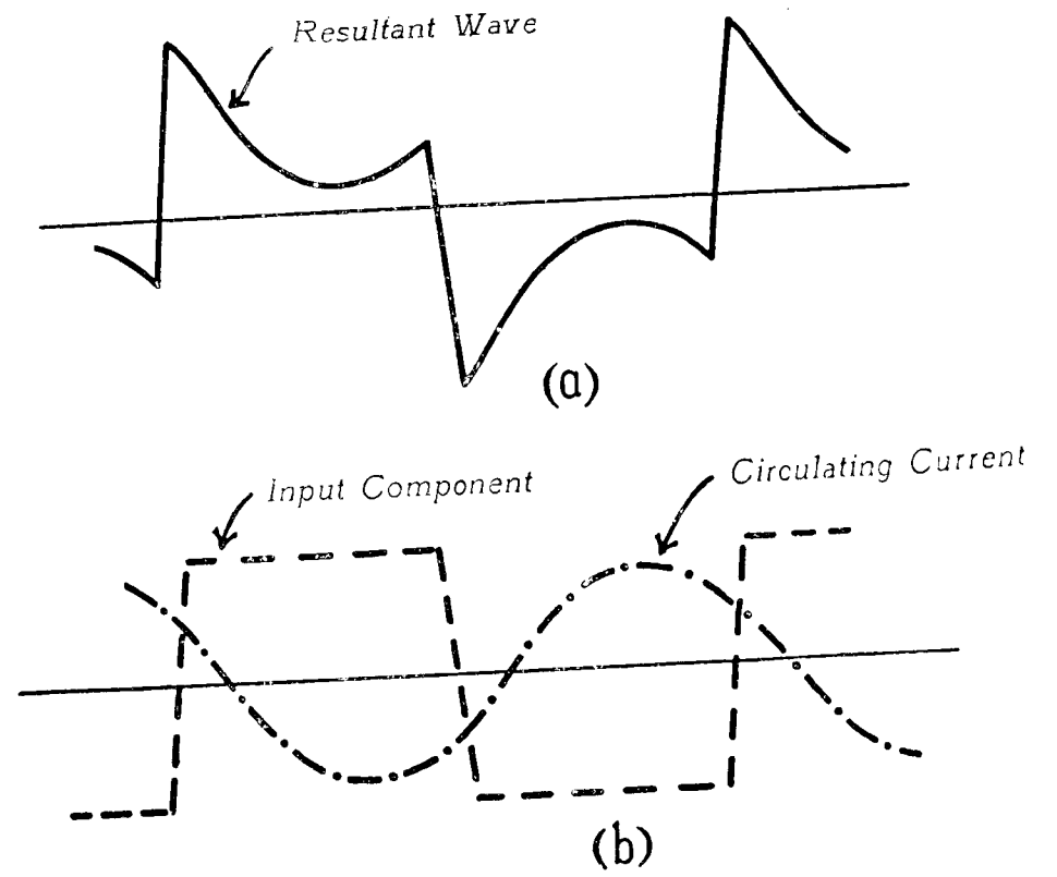
Fig. 3. Armature Current Wave and its Components.
