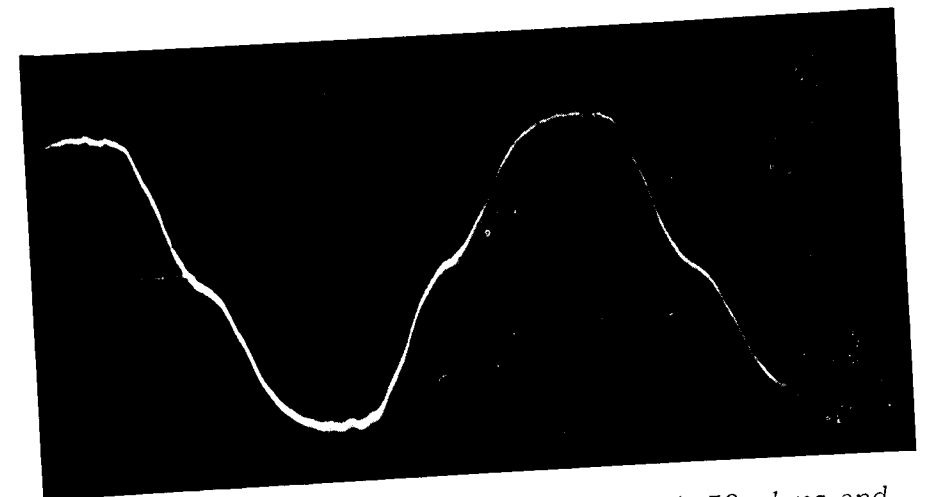
Plate 10. Current through search coil with 50 ohms and 0.1 henry, machine running as motor on load.
