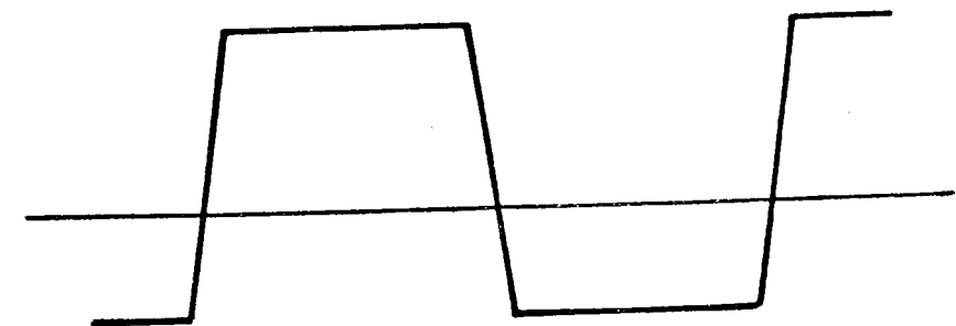
Fig. 4. Wave of Current due to unequal Flux under different Poles.
