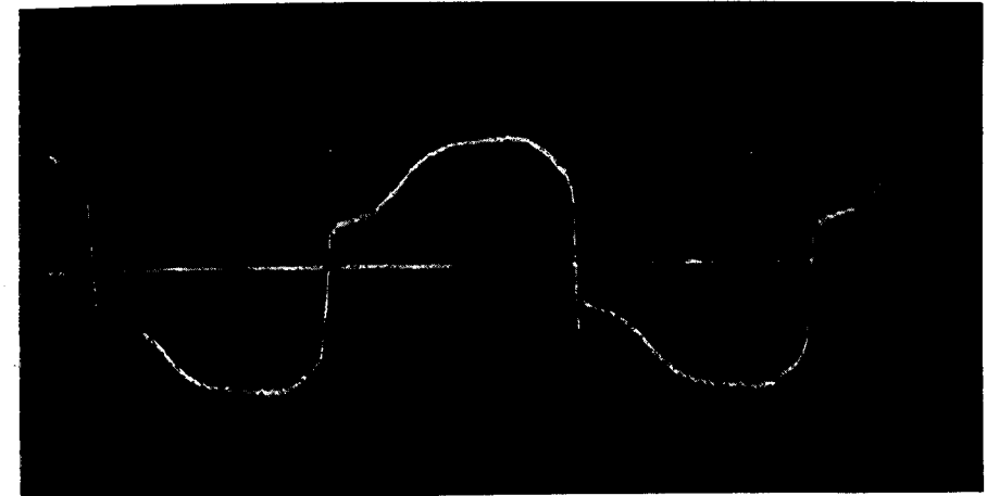
Plate 7. Current through coil b, machine running as motor on no load.
