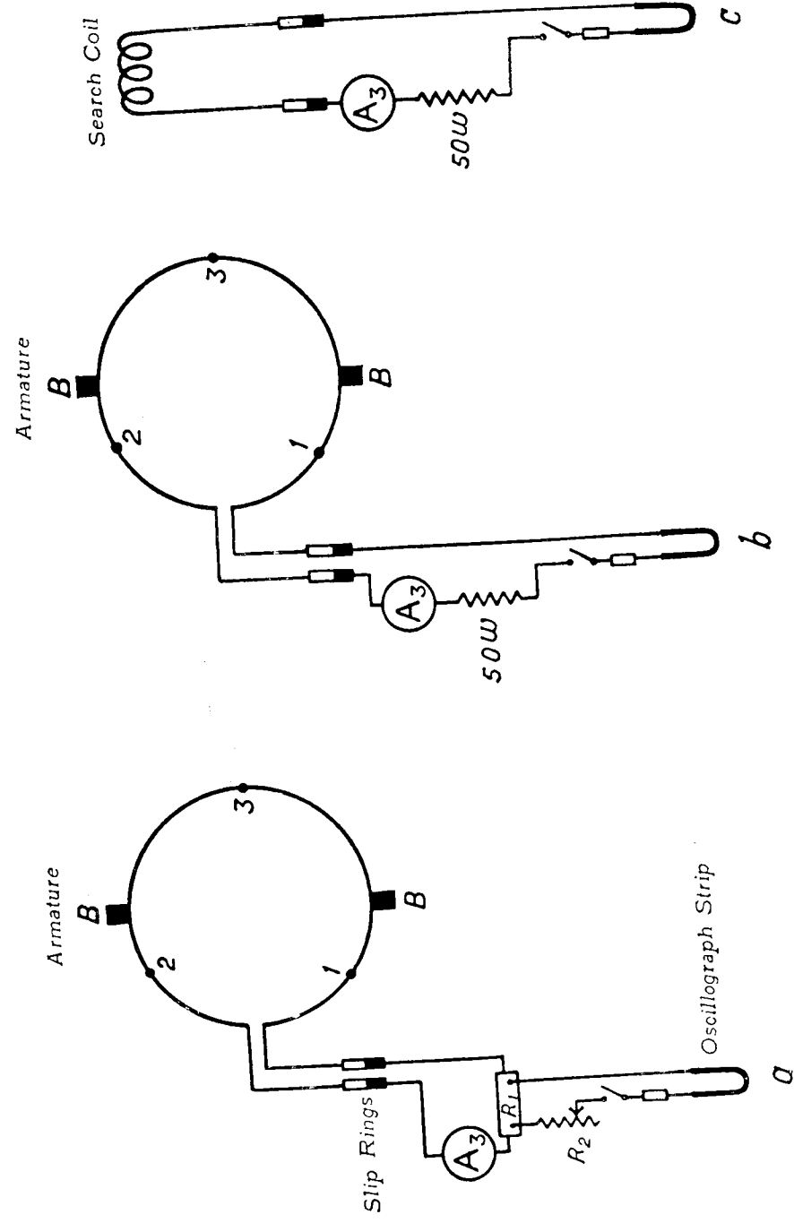
Fig. 6. Oscillograph Circuits.
