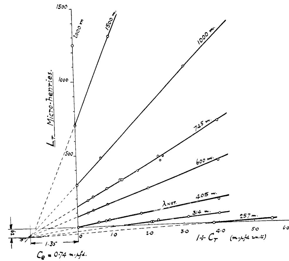
Fig. 2. Tuning Characteristics of Small Aerial with Counterpoise.
