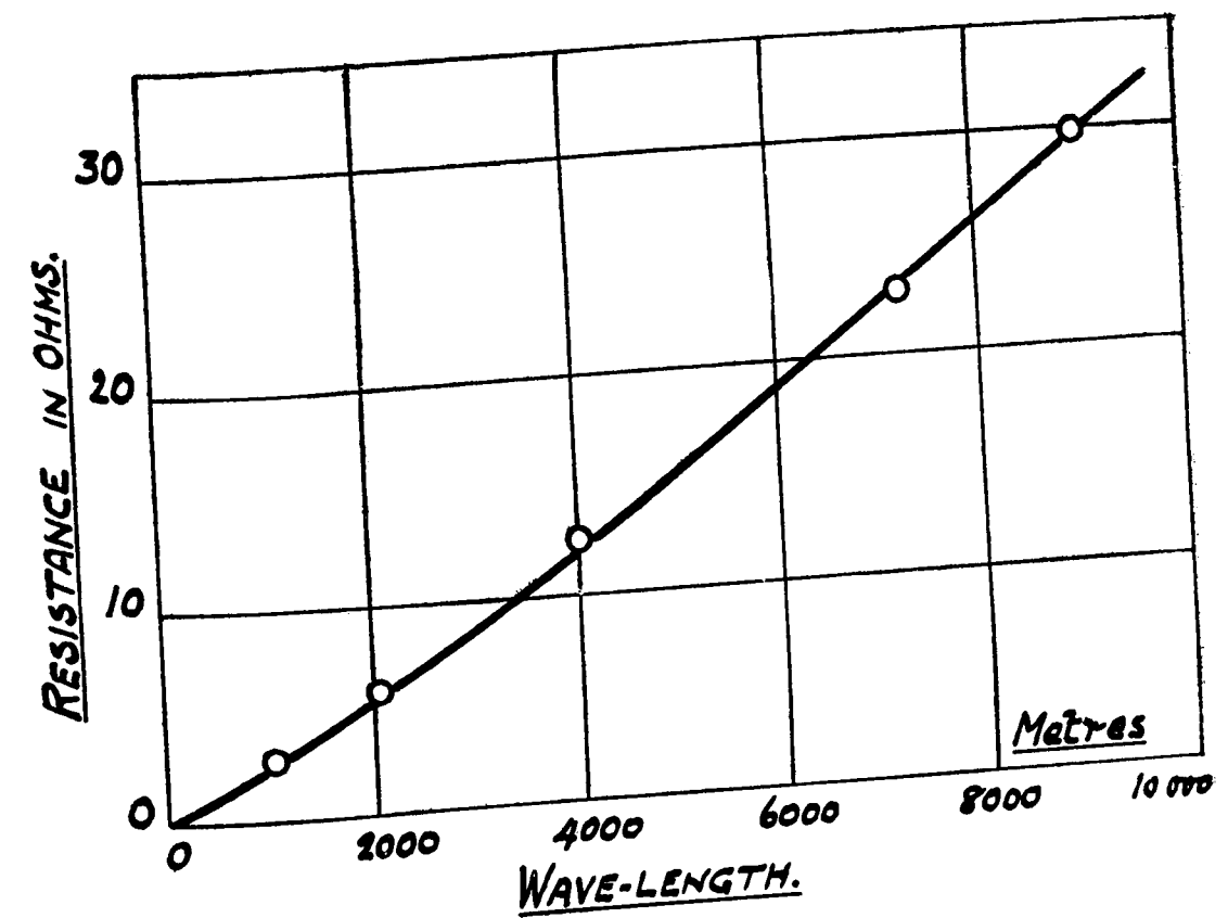
Fig. 9. Variation of Dielectric Resistance with wavelength. 0.002 \mu fd. mica and moulded plate condenser.
