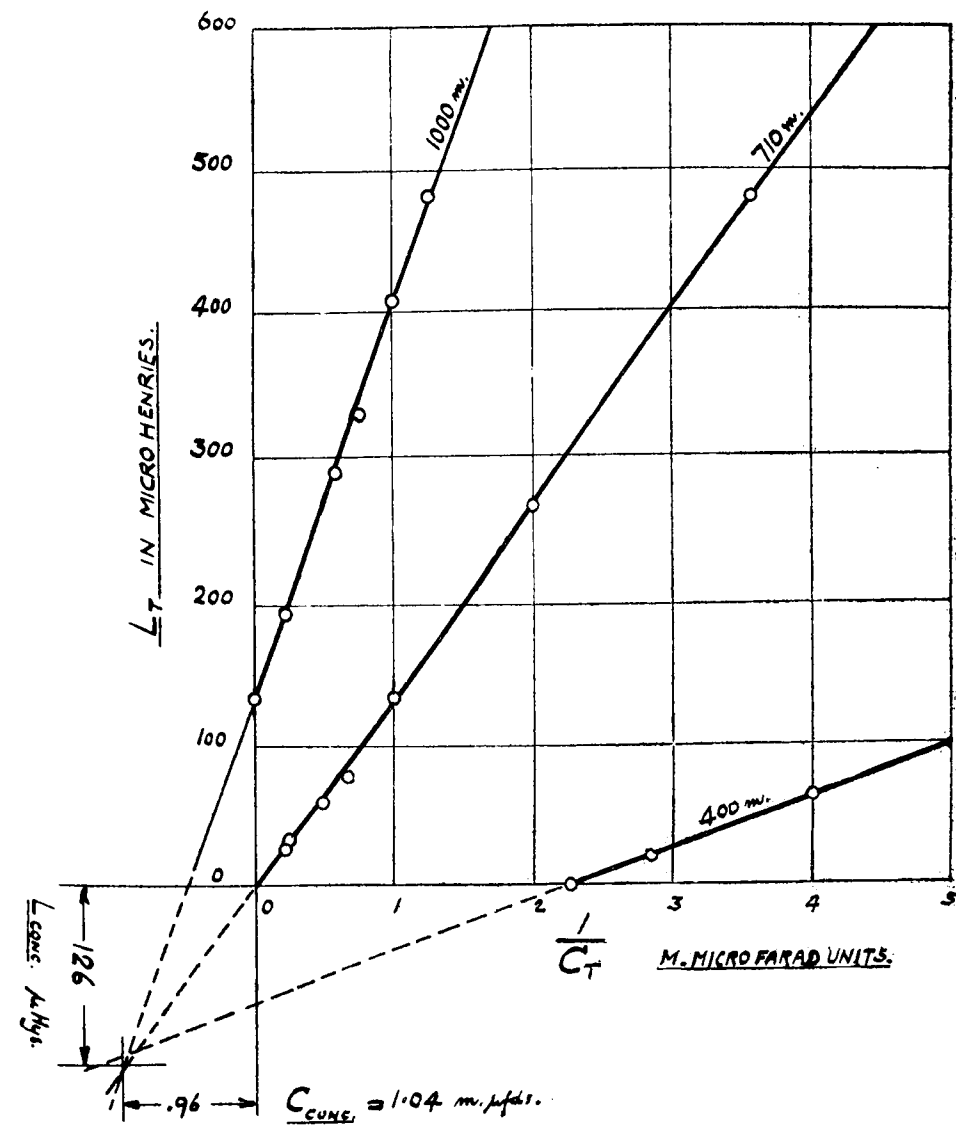
Fig. 5. Experiment with Concentrated Circuit Constants.
