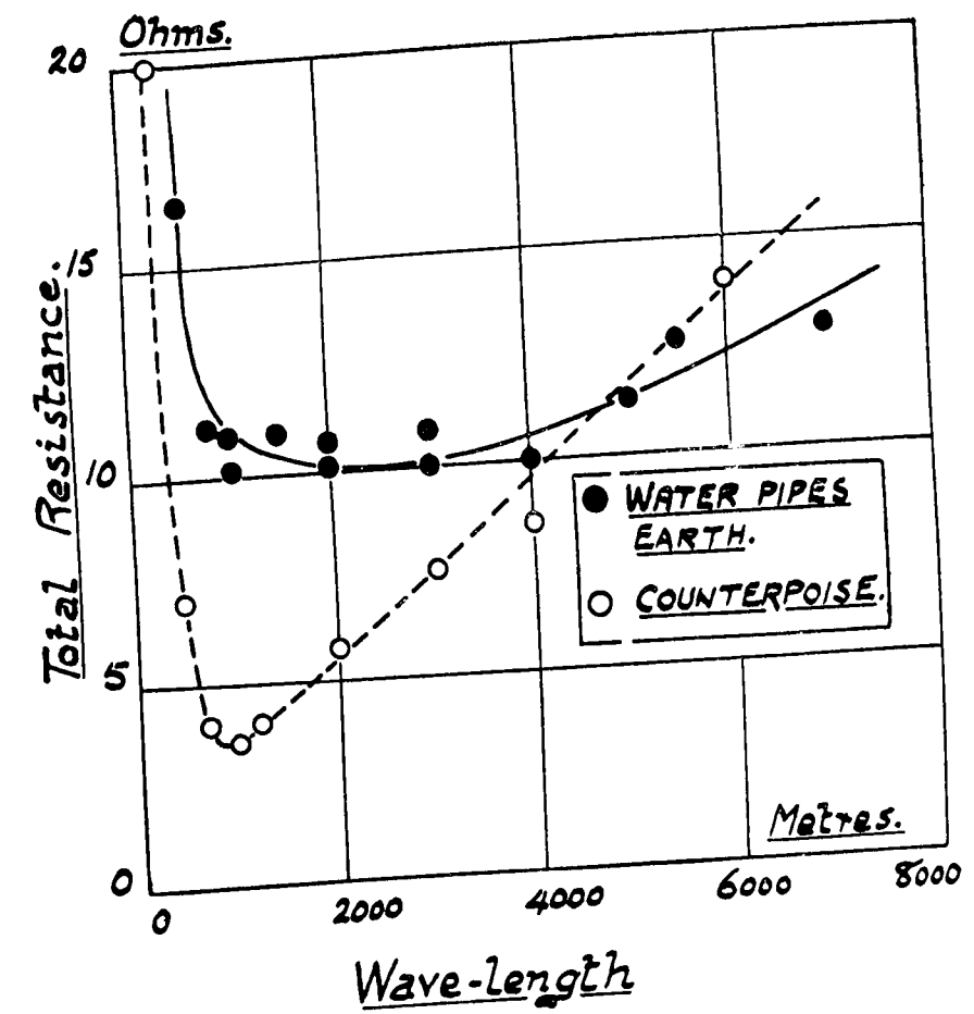
Fig. 8. Aerial Resistance, Inverted L. Two 90 ft. Steel Masts 200 ft. apart. Indian Institute of Science, Bangalore.
