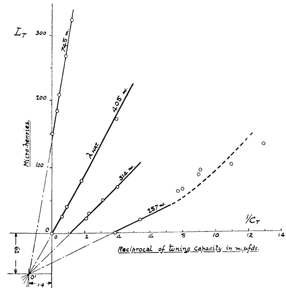
Fig. 3. Tuning Characteristics below Fundamental Wavelength.
