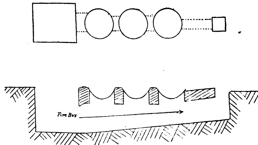
Fig. 1. Ordinary Burmese furnace (without fire-bars). Scale, \frac{1}{2} inch = 1 foot roughly.
