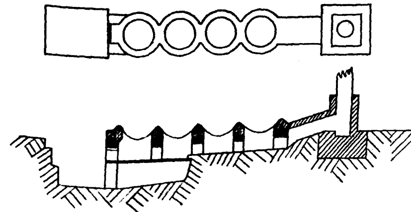
Fig. 2. Improved Burmese furnace with fire-bars. Scale, \frac{1}{8} inch = 1 foot roughly.
