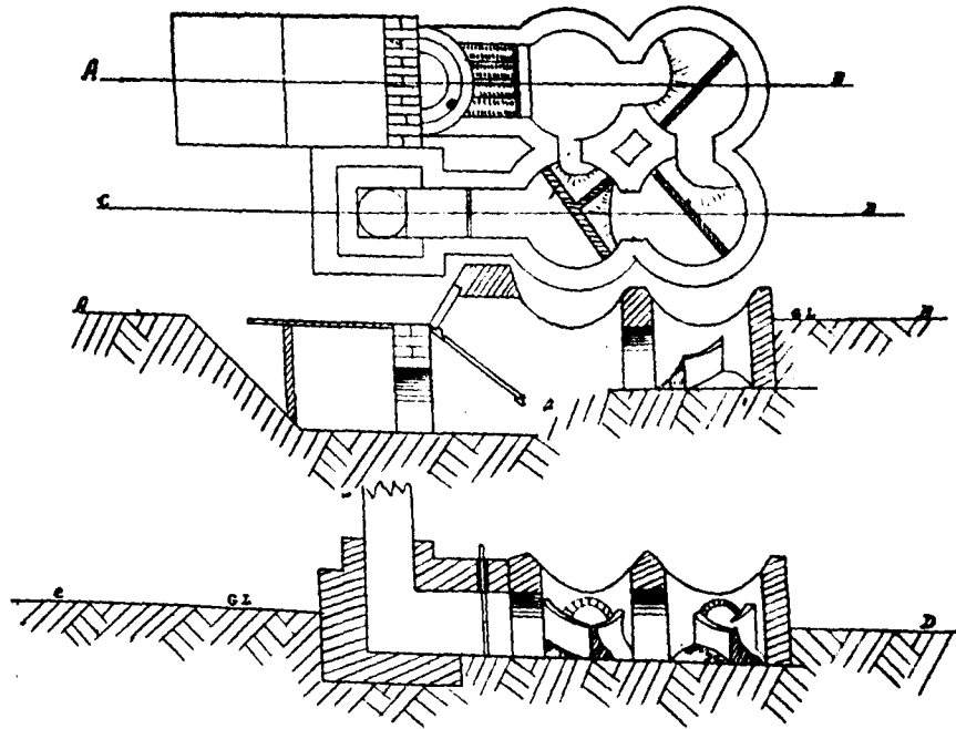
FIG. 6. Return type furnace for megass burning designed by the Agricultural Department Scale, 1/4 inch = 1 foot roughly.
