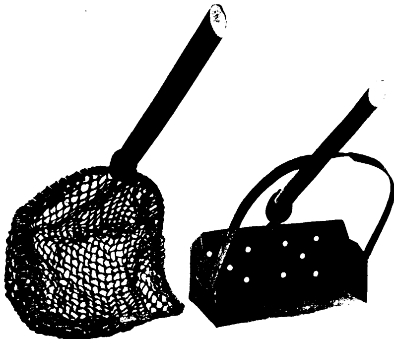
(A) Net Pattern—5½ lb. —A good tool for removing duckweed and semi-buoyant "slub" from dykes—a trifle too heavily built.
