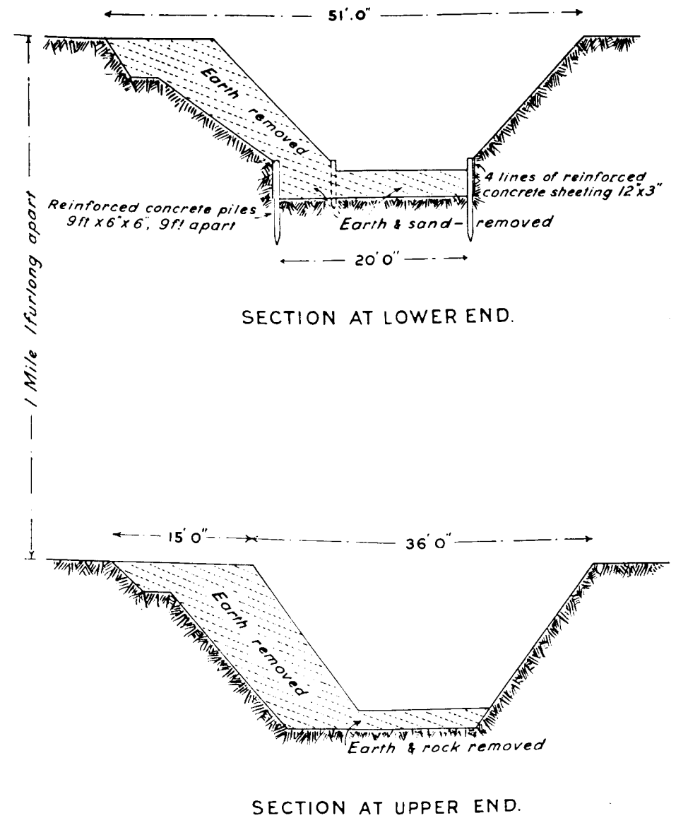
FIG. 9.—Sections of the White House Drain, BURNT FEN SCHEME (Area No. 1).
