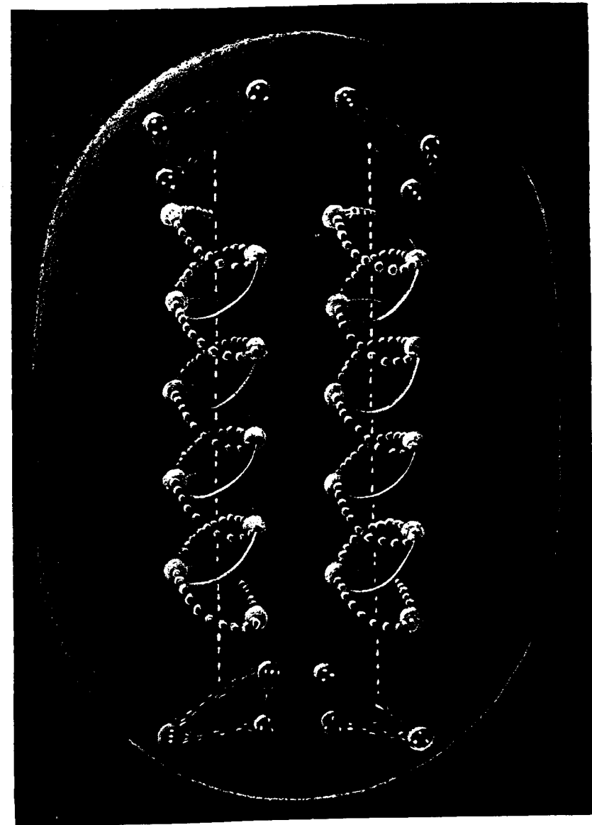
FIG. 15. HYDROGEN PEROXIDE H_2O_2
