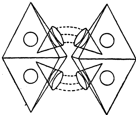
FIG. 17. TWO CARBON ATOMS LINKED TO EACH OTHER C=C
