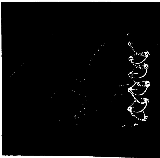
FIG. 16. METHYL ALCOHOL CH_3OH
