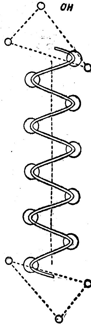
FIG. 14. HYDROXYL ION, OH
