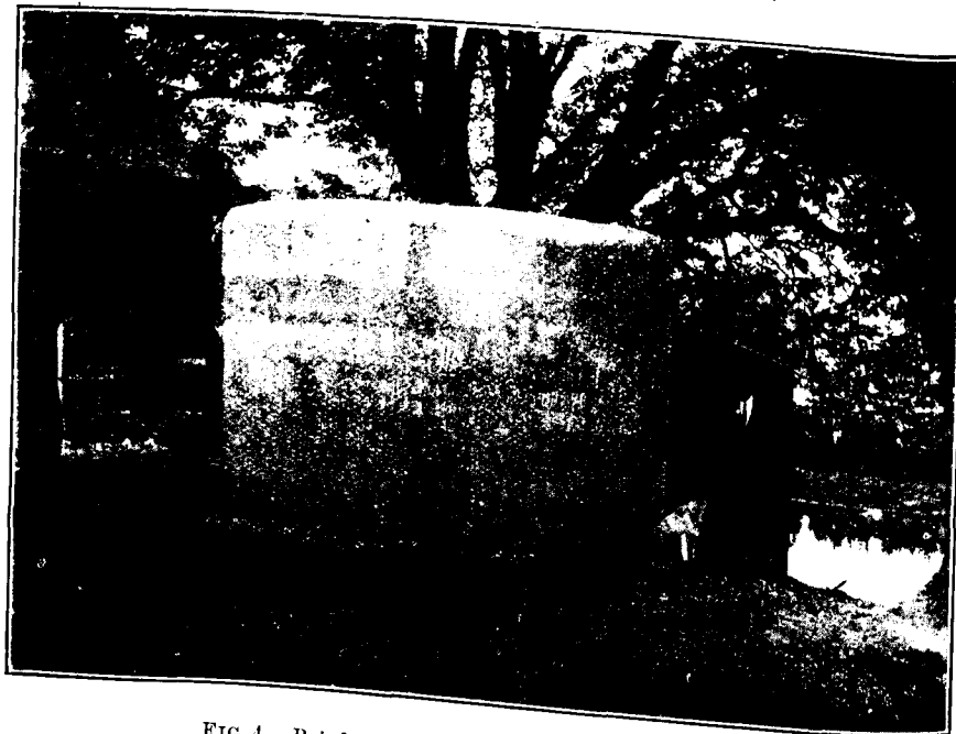
FIG. 4.—Reinforced Concrete Water Tank at Brundon.
