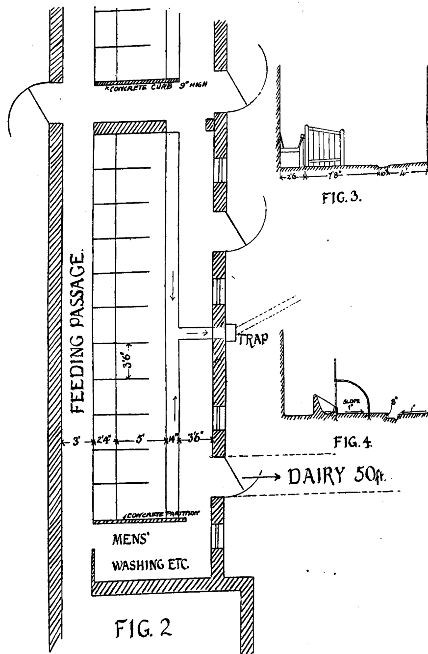
FIG. 2.—Plan of re-constructed Shed. " 3.—Section of Cowshed before re-construction. " 4.— " " after " "
