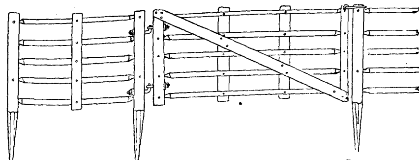
FIG. 3.—Standard 6 ft. by 3 ft. Hurdle and Gate with 5 Cross Bars.
