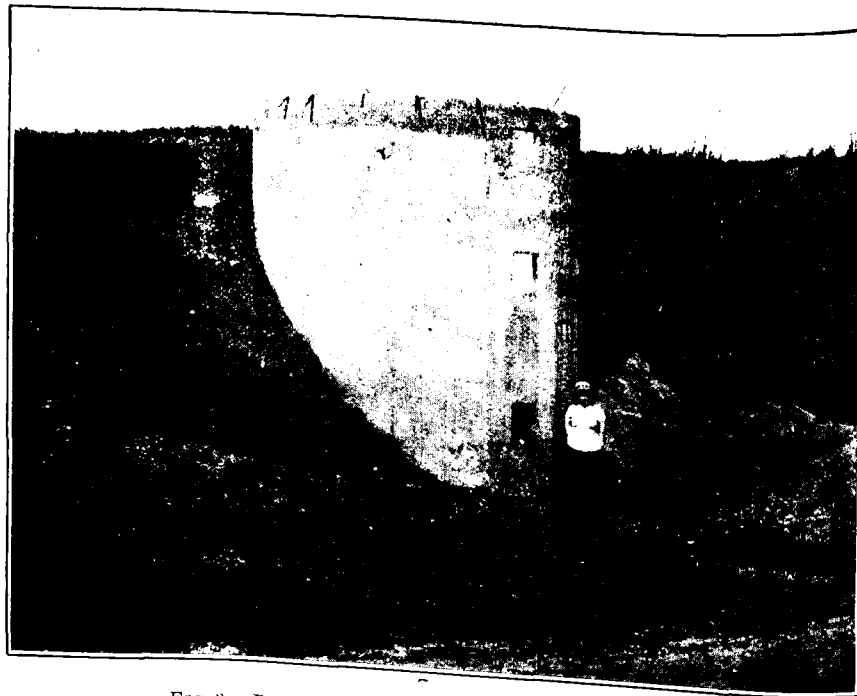
FIG. 3.—Reinforced Concrete Pit Grain Silo at Brundon.
