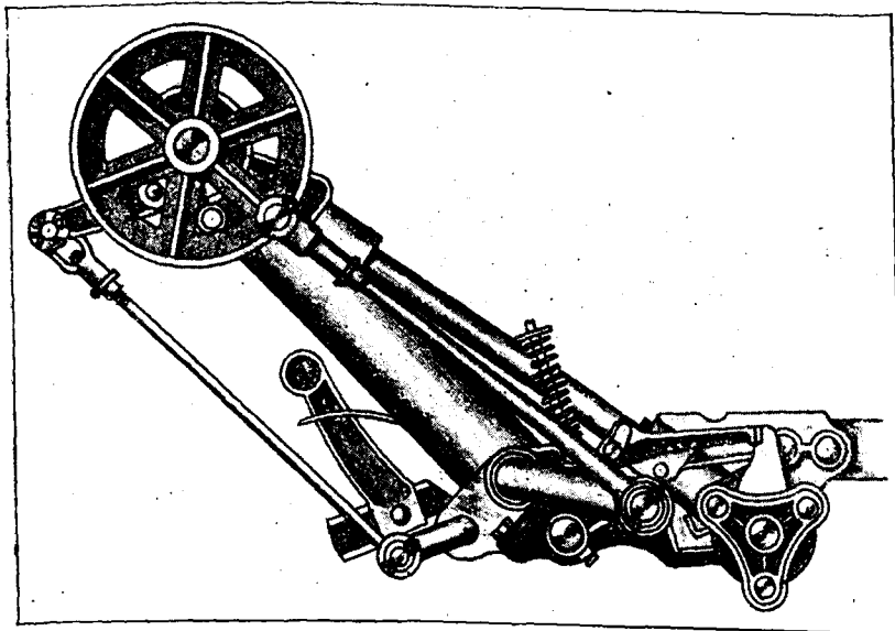
FIG. 7.—Binder Head showing Adjustable Connecting Rods for Needle Shaft (right), and Stop Arm holding Dog (right corner).
