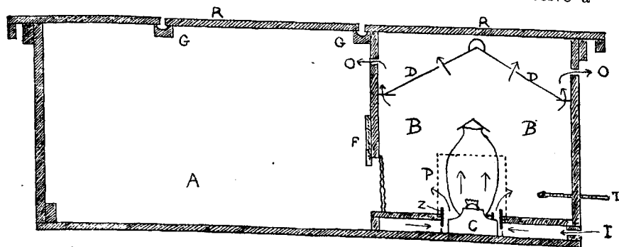
FIG. 2.—Vertical Section of Lamp Brooder. Length 6 ft.; breadth 2 ft. 1\frac{1}{4} in.; height 1 ft. 11 in. front, 1 ft. 7 in. back. (R) Roof in sections, hinged behind, and covered with bituminous felt. (A) Outer chamber, (B) inner chamber, (C) hurricane lamp, (D) cone of iron sheeting, (I) fresh air inlets, (F) sliding trap door, (G) back to front roof supports with groove to carry off water, (O) foul air outlets, (P) perforated zinc collar, (Z) zinc collar.
