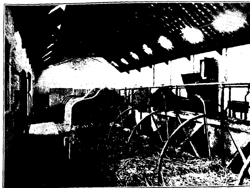
FIG. 1.—Cowshed for 30 Cows, with Bull Pen and Calf Stalls.
