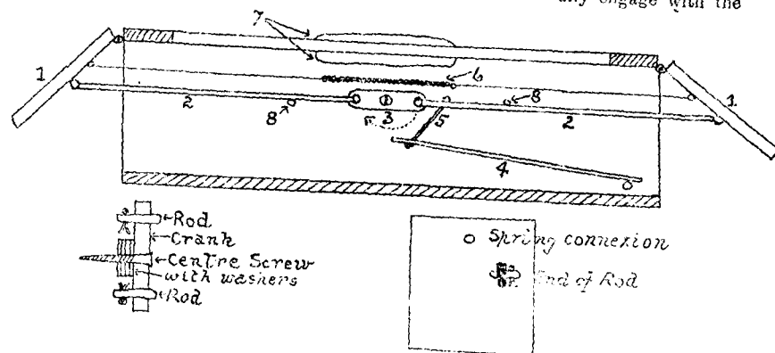
Fig. 3.—'Straight through' Box Trap (Longitudinal Section). 1. Trap Doors. 2. Thick Wire Rods which actuate doors. 3. Crank, free to rotate on its centre screw. As shown it is at dead centre, and both doors are prepped open. As the crank turns in direction of arrow both doors close. 4. Spring Plate. 5. Cord connection between spring plate and crank. 6. Door Spring. 7. Strong Spring in lid for bait and handle. 8. Stops.
