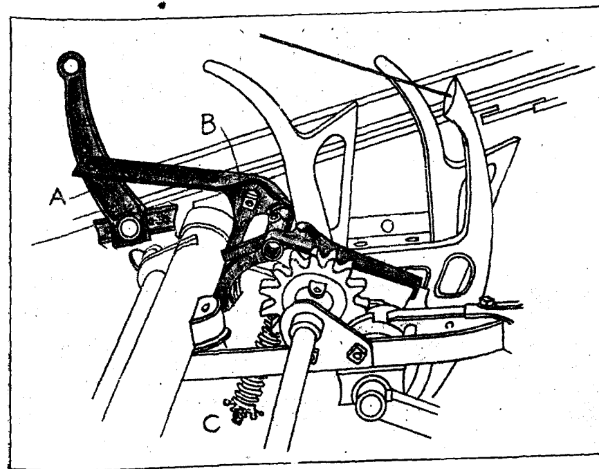
FIG. 8.—Shafting Mechanism.—A, Compression Arm ; B, Trip Lever ; C, Trip Spring.
