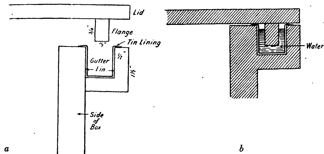
FIG. 14. Details showing construction of the fumigating-box.
