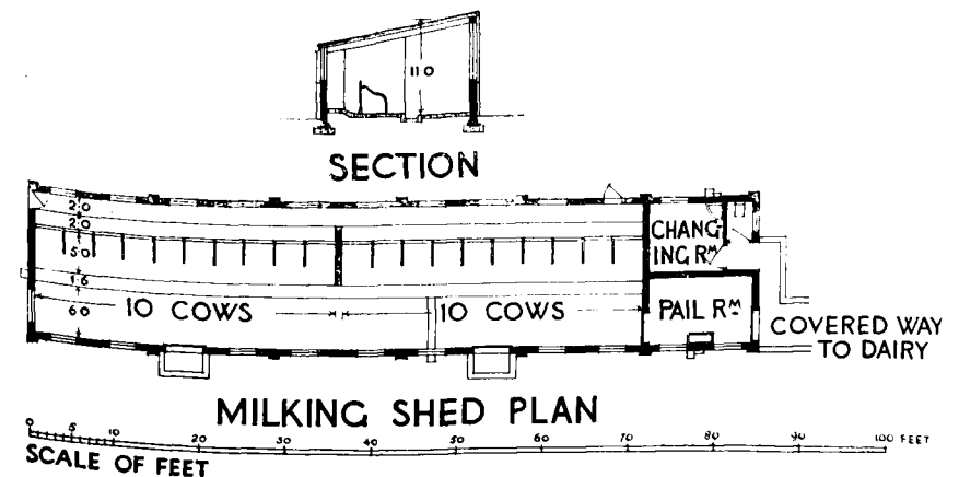
FIG. 2.—Plan and Section of Milking Shed.
