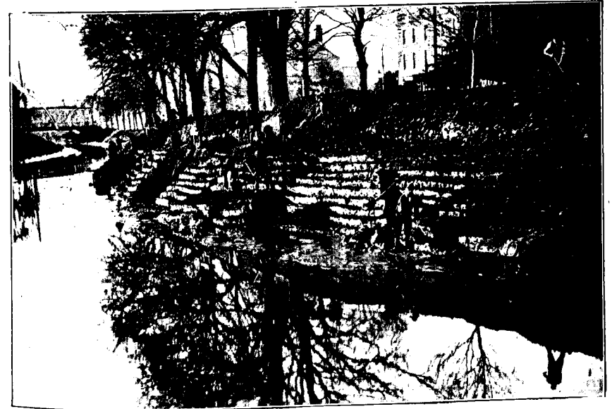
FIG. 7.—River Welland at Spalding : Digging out Cesses and widening the Waterway.
