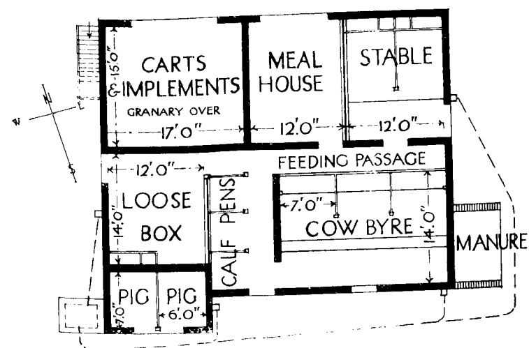
FIG. 3.—Plan of Farm Buildings.
