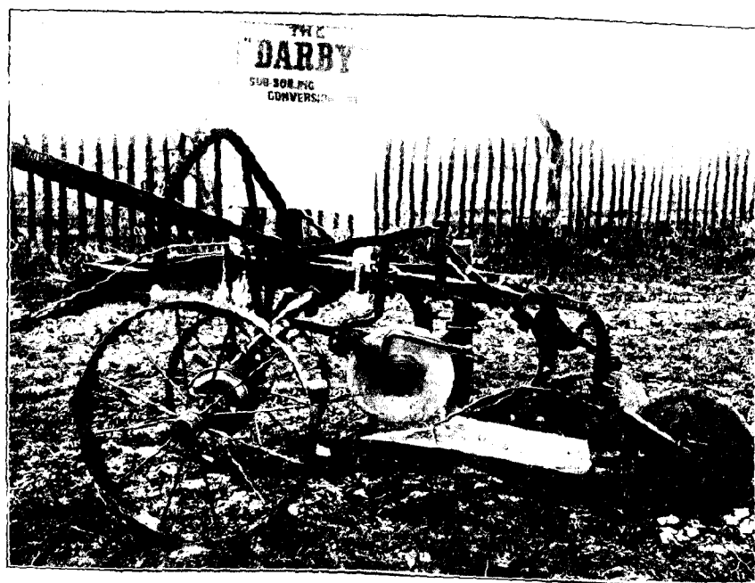
FIG. 4.—Darby Sub-Soiling Conversion Set.
