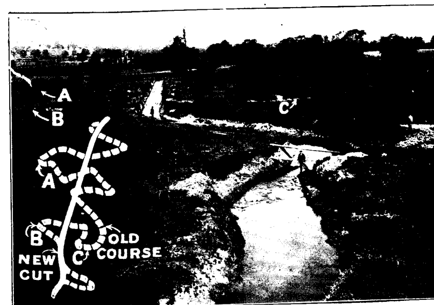
FIG. 1.—The River Anker, Warwickshire: A typical case of river straightening.
