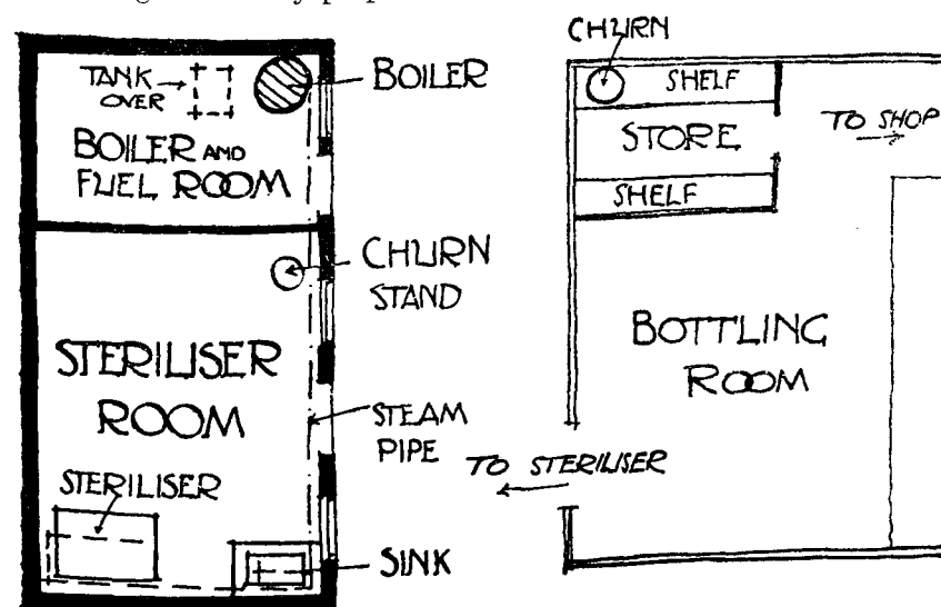
FIG. 1.—Old Stable adapted for Sterilizing Plant.
