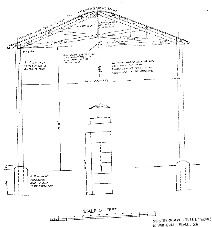
FIG. 1.—Design for Timber Dutch Barn.
