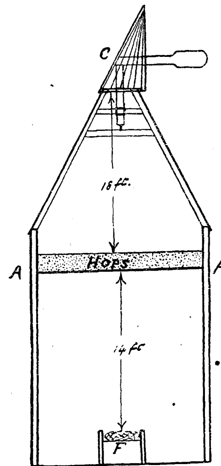
FIG. 1.—Hop Oast. F, fireplace; AA, drying floor; C, cowl.
