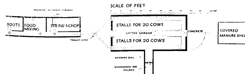
FIG. 1.—Ground Plan of Farm Building.
