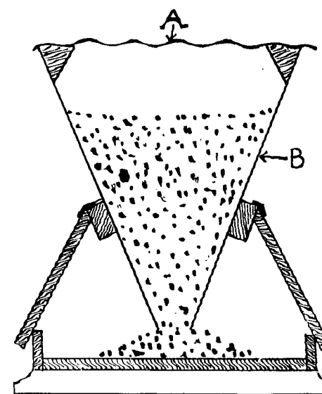
FIG. 2.—Cross Section of Feeder shown in Fig. 3.
