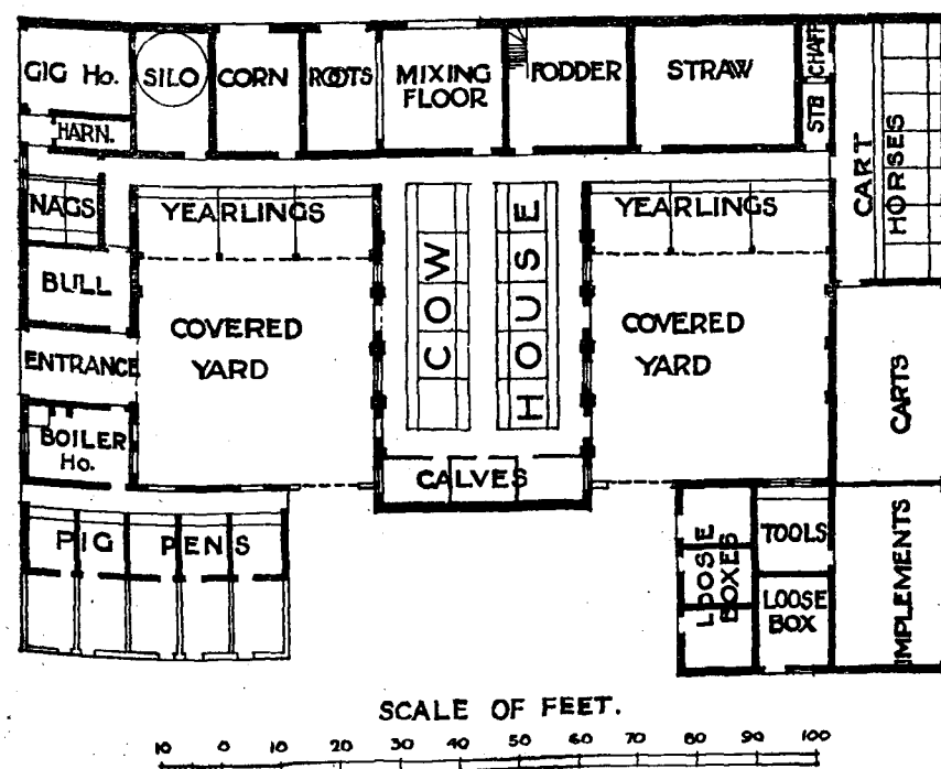
FIG. 2.—Original plan of Farm Buildings, Seale-Hayne Agricultural College.
