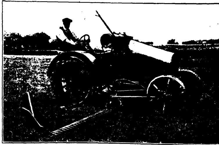
FIG. 4.—The International Tractor Mowing Attachment.
