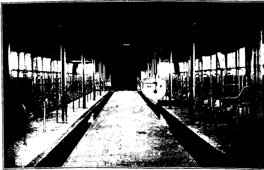
FIG. 3.—Interior of Cow-byre, showing Overhead Trolley system for removing manure.
