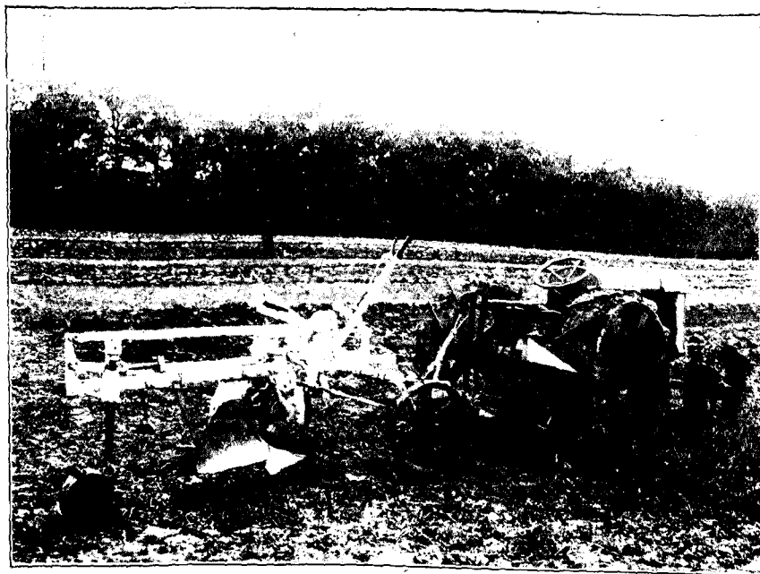
FIG. 3.—Celliers' Sub-Soiler for attachment to Tractor.
