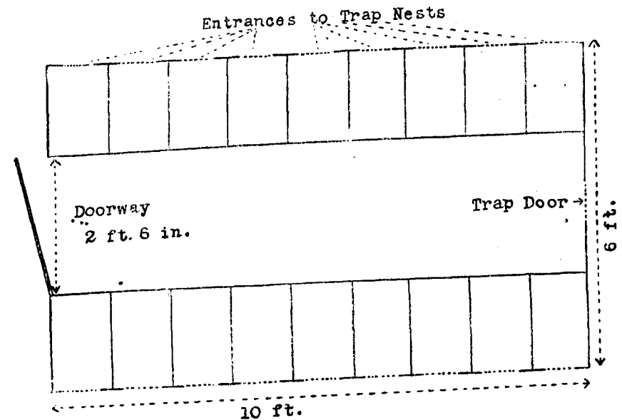
FIG. 1.—Plan of Duck House designed for Recording with Trap Nests.
