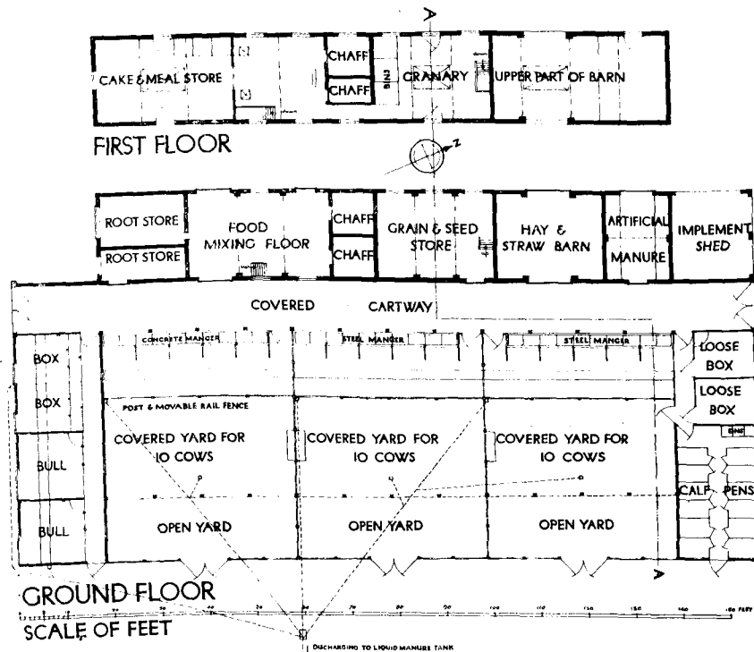
FIG. 3.—Plan of Main Farm Buildings.
