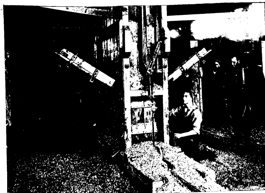
FIG. 2.—Baling Press, showing Hops pressed ready to close the bale.
