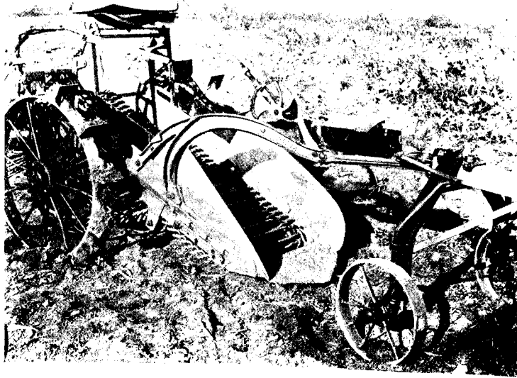
FIG. 3.—Potato Digger (Elevator Class).
