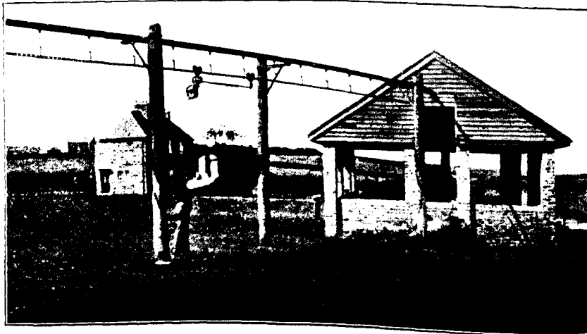
FIG. 4.—Covered Manure Shed with Overhead Trolley system from Cow-byre.
