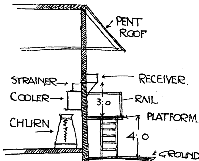
FIG. 4.—Beansheaf Farm: Section through Cooling Room.
