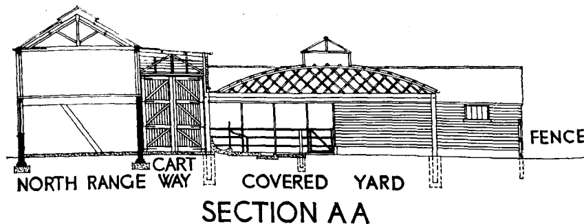
FIG. 4.—Section through line A A on Fig. 3.
