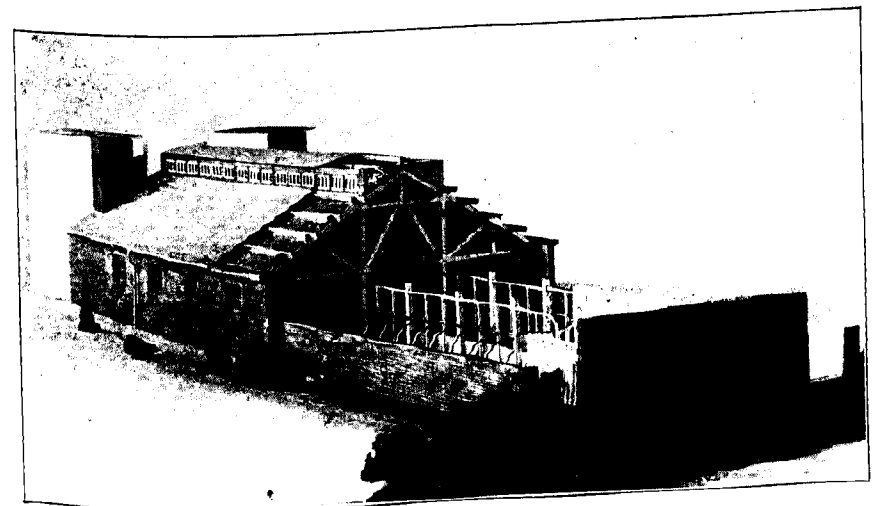
View of Model. (Part of Roof removed to show interior.) FIG. 3. —Suggested development of Hucknall Cow-house for 40-50 cows, with head to head arrangement (Scheme A).
