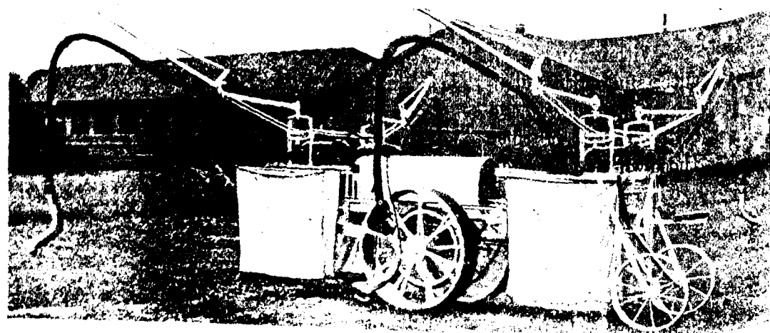
Close-up view of the Stuckenberg cotton picker and the tractor that carries it.
