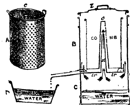
FIG. 3.—Gerster Wax Extractor.
