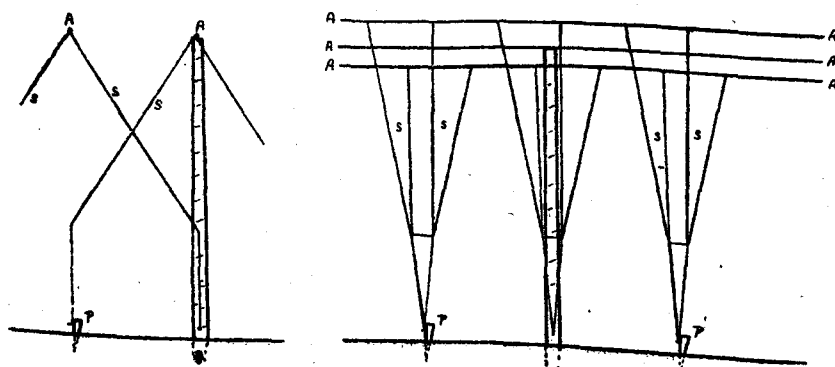
Cross Butcher System of Training Hops. AA, string wires; SS, strings; PP, pegs.
