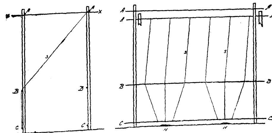
Butcher System of Training Hops.
