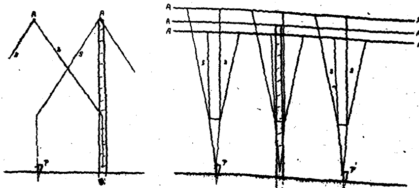
Cross Butcher System of Training Hops. AA, string wires; SS, strings; PP, pegs. FIG. 6.—End view.
