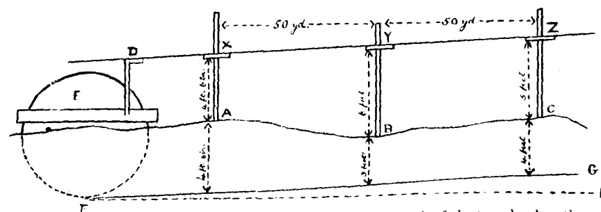
FIG. 4.—Diagram showing the method of adjusting the depth of the trench when the machine passes over uneven land.
