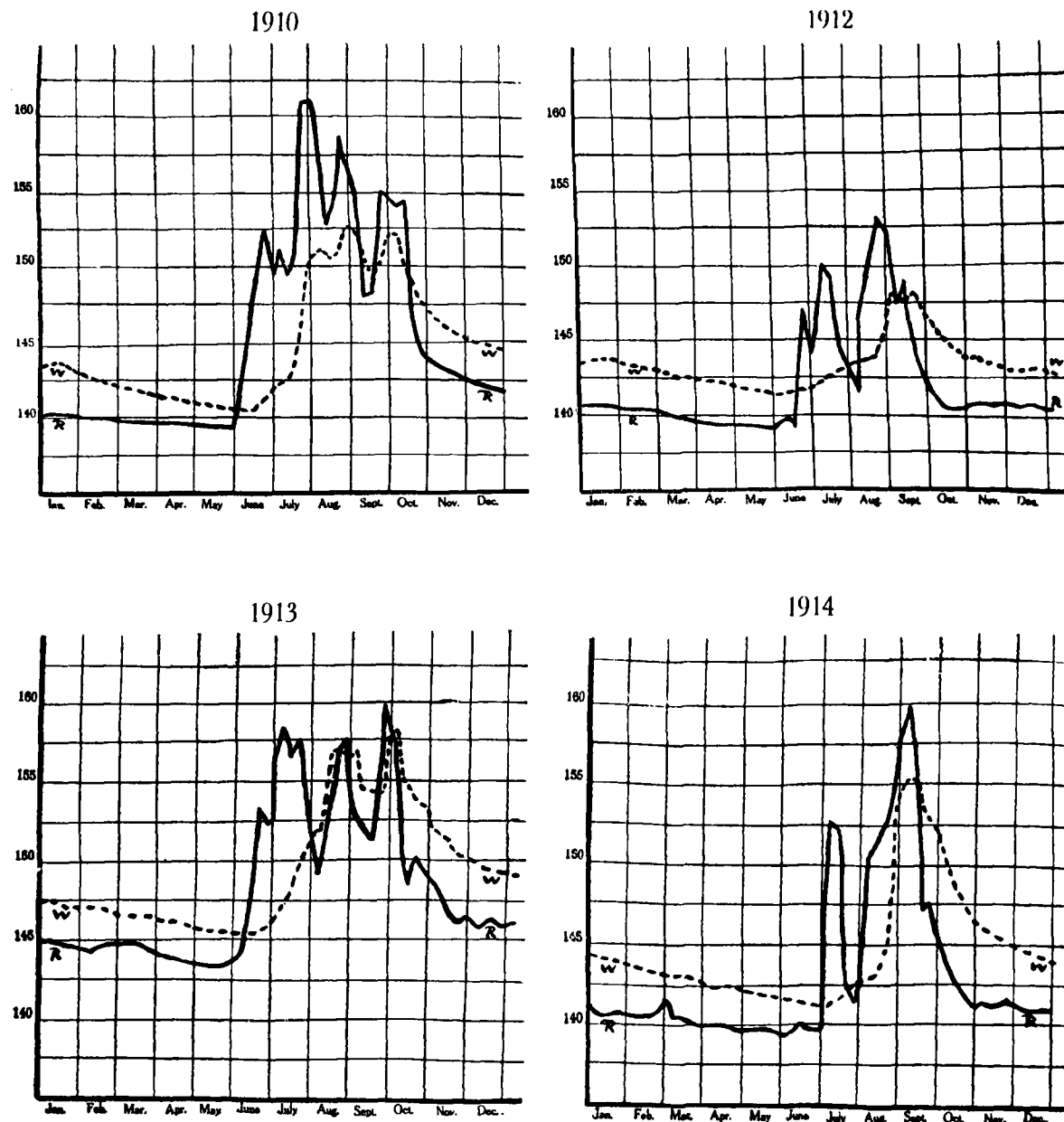
CHANGES IN THE RIVER AND WELL LEVELS AT PUSA.
