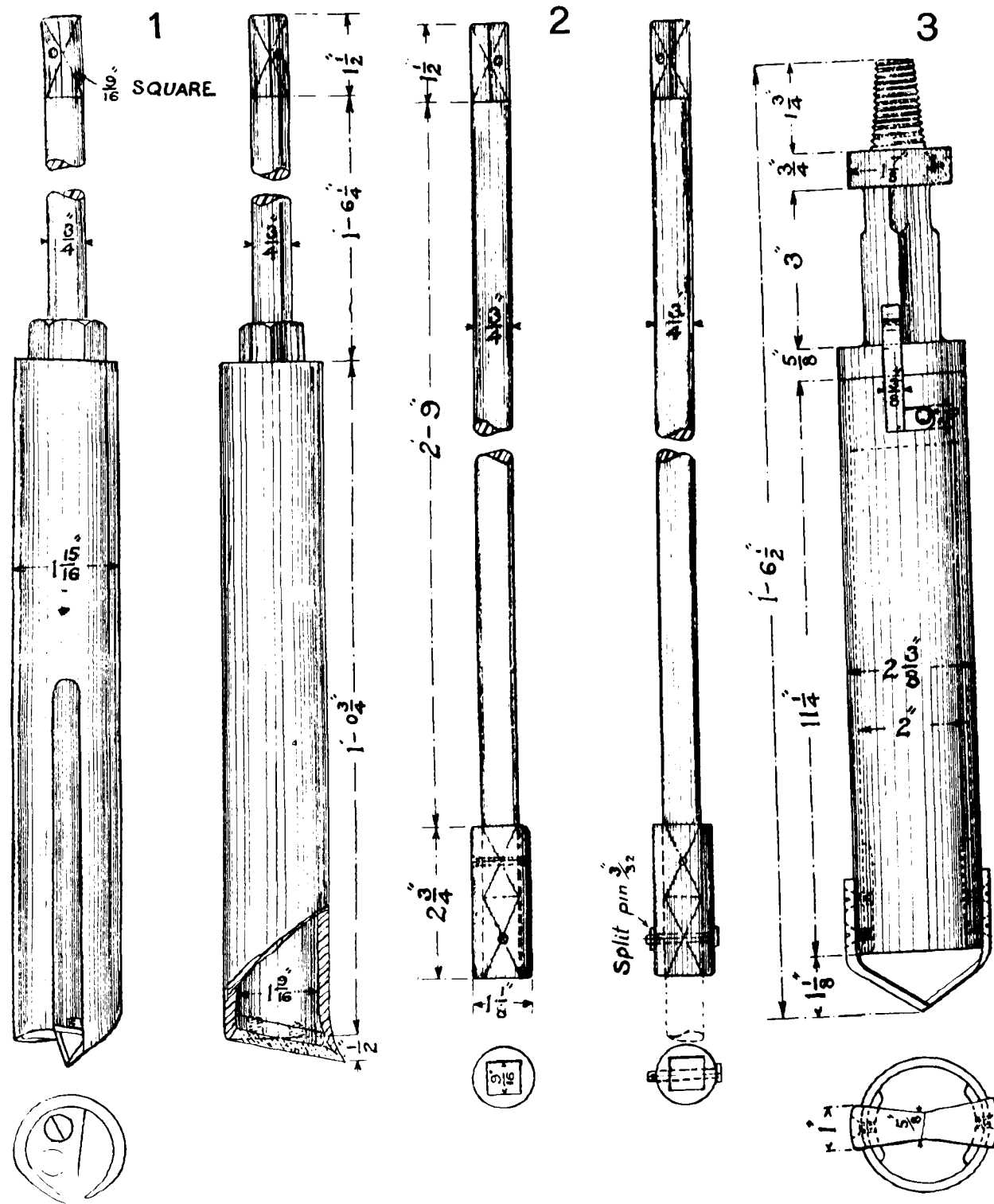
A NEW SOIL SAMPLER
