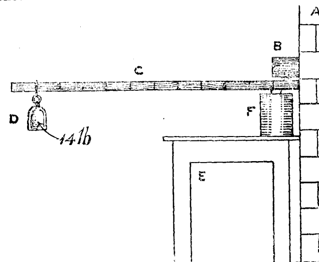
A—Wall; B—Block of wood fixed on wall; C—Wooden lever, 6 ft. long and 2 in. by 2 in. section; D—Weight; E—Kitchen table; F—Cheese mould containing cheese.
