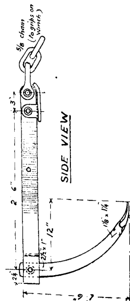
FIG. 4.—Side View of Anchor.
