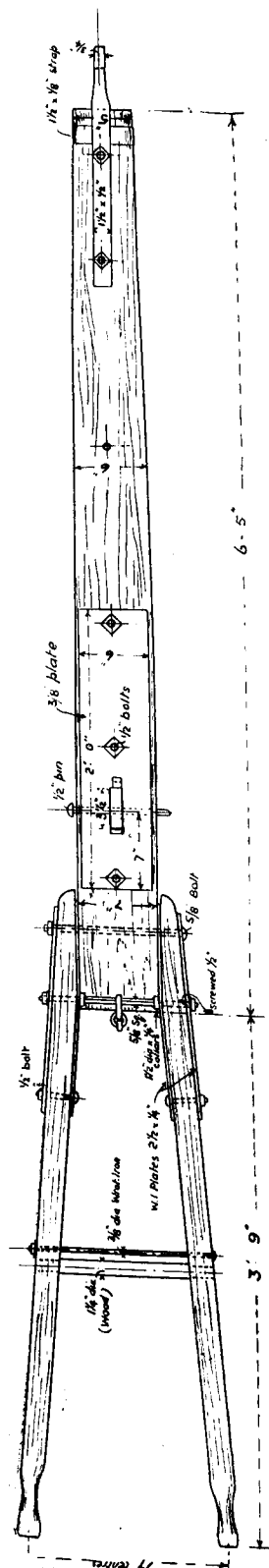
FIG. 2.—Details of Mole Plough (scale \frac{1}{4} in. to 1 foot). Horizontal section.
