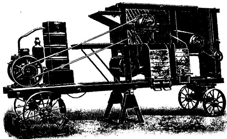
Small Thresher and 5 B.H.P. Engine, mounted on a Telescopic Platform, with 18-in. Drum. Very suitable for small holders.
