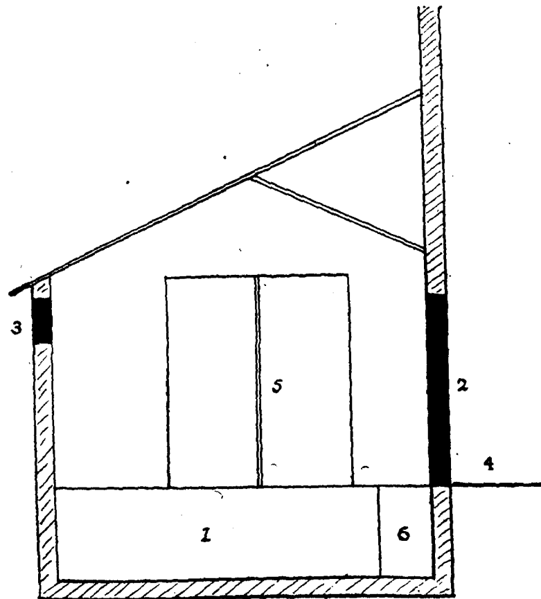
FIG. 5.—Solid Manure Pit adjoining Cattle House.
