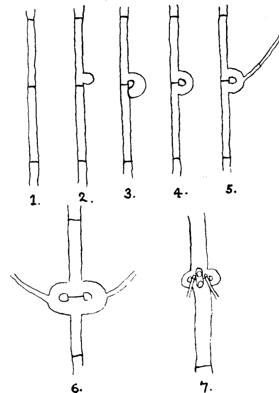
Diagrams of highly magnified hyphæ of fungi causing dry rot. (In these diagrams the relative dimensions of the constituents are not necessarily natural).
