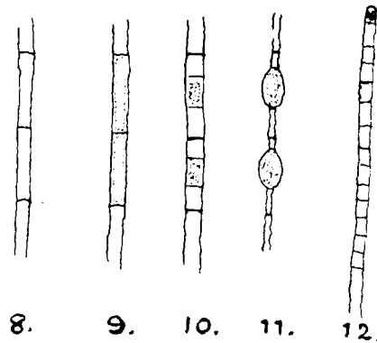
Diagrams of highly magnified hyphæ of fungi causing dry rot. (In these diagrams the relative dimensions of the constituents are not necessarily natural).
