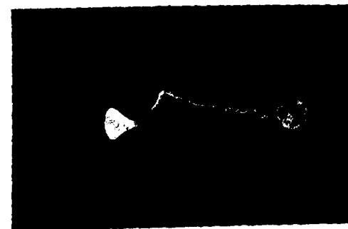
FIG. 4.—STALK DISEASE. A single " Sclerotinia ," which, after lying dormant during winter, has produced a spore-bearing cup or apothecium (nat. size).
