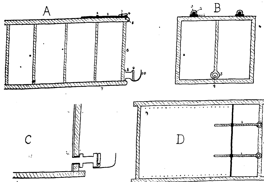
FIG. 4.—Kist (Large Size) for Liquid Manure.
