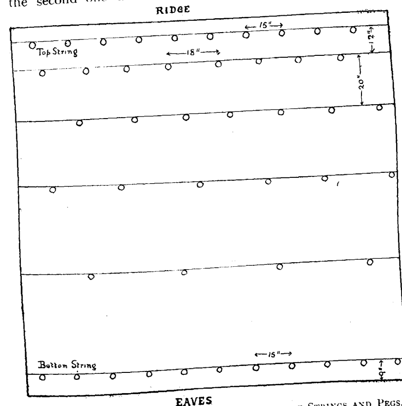
DIAGRAM OF SECTION OF ROOF SHOWING POSITION OF STRINGS AND PEGS.
