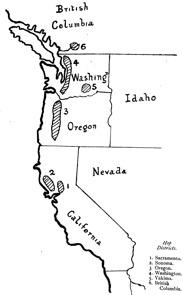
MAP SHOWING THE POSITION OF THE CHIEF HOP-GROWING DISTRICTS OF THE PACIFIC COAST OF AMERICA.
