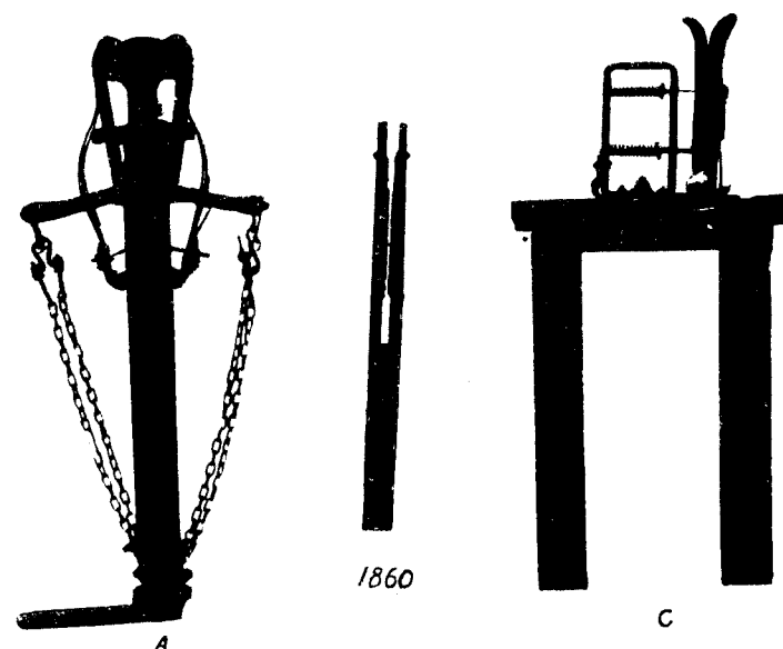
A, machine worked by foot; will peel two rods at one time; C, machine adapted for peeling two-year-olds or sticks. The illustration in the centre is of an actual machine used fifty years ago.
