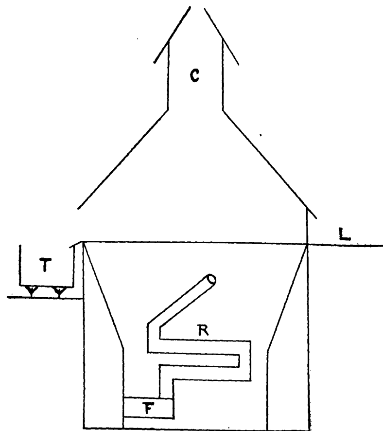
DIAGRAM OF HOP KILN.
