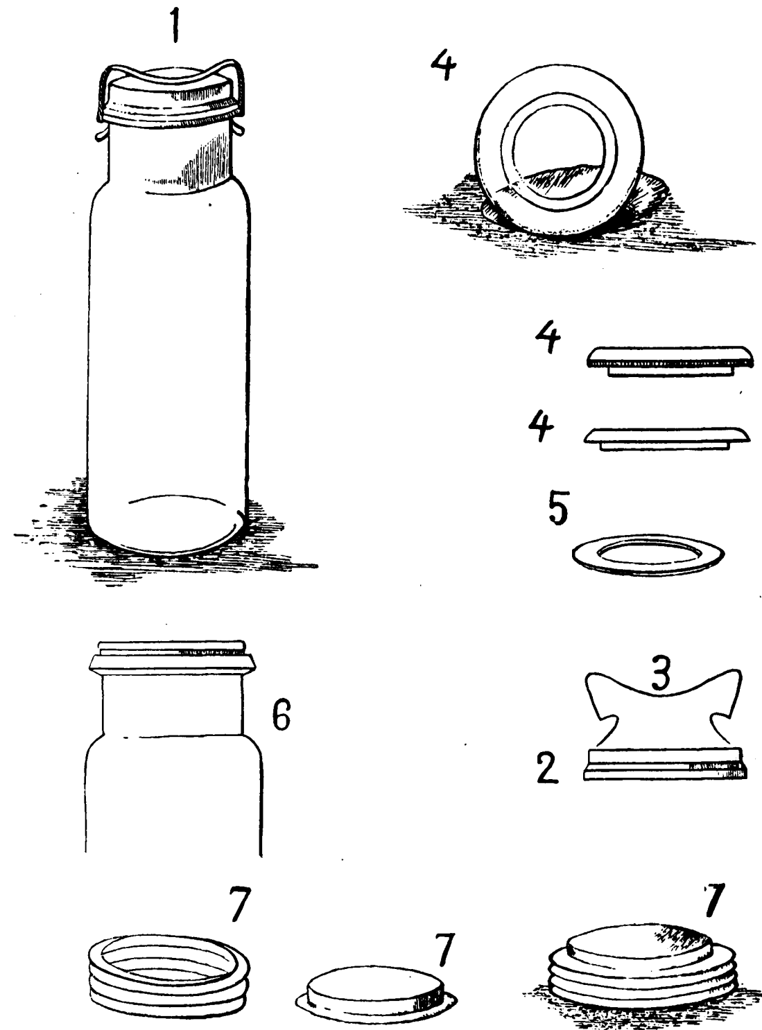
1.—GLASS BOTTLE WITH METAL CAP AND SPRING FIXED. 2.—METAL CAP. 3.—SPRING. 4.—GLASS COVER OR CAP. 5.—RUBBER RING. 6.—TOP OF BOTTLE WITHOUT CAP. 7.—SCREW AND CAP FOR SCREW-TOP BOTTLES.
