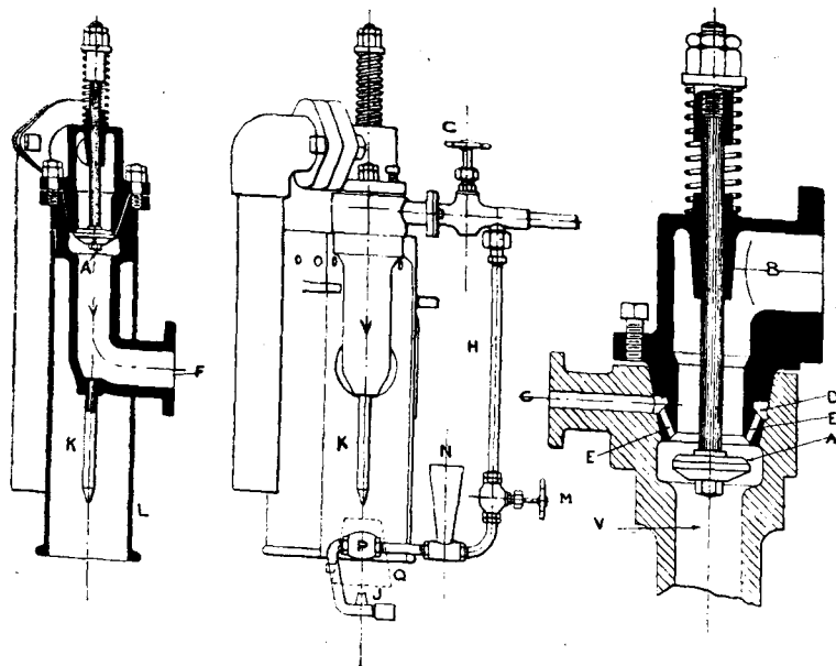
FIGS. 13, 14, 15.—THE CAMPBELL OIL ENGINE.—VAPOURISER AND IGNITION APPARATUS.
