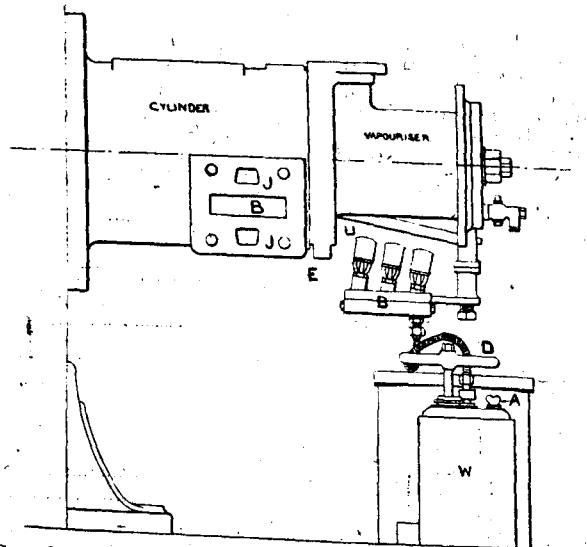
FIG. 8.—STARTING LAMP OF CLAYTON & SHUTTLEWORTH OIL ENGINE.
