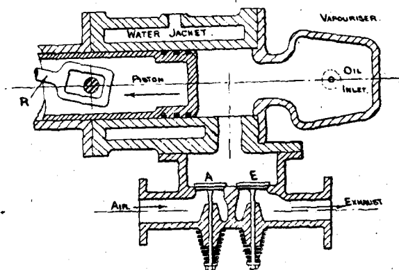
FIG. 1.—DIAGRAM OF HORNSBY-ACKROYD ENGINE.
