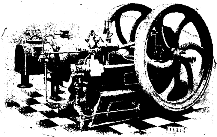
FIG. 2.—HORNSBY-ACKROYD OIL ENGINE (30 H.P.).
