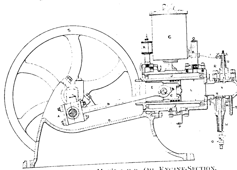
FIG. 11.—BROWN & MAY'S 3 H.P. OIL ENGINE-SECTION.
