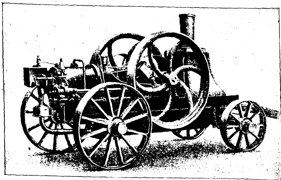
FIG. 18.—THE KYNOCH-FORWARD PORTABLE OIL ENGINE, (7 h.p.)
