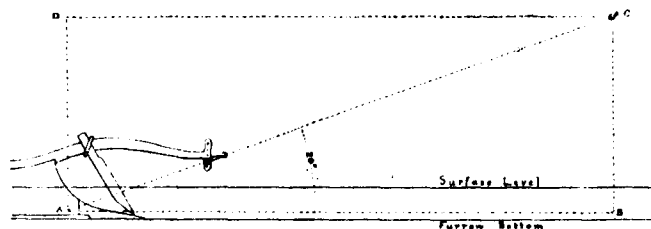
FIG. 1.— Draught of the Plough.
