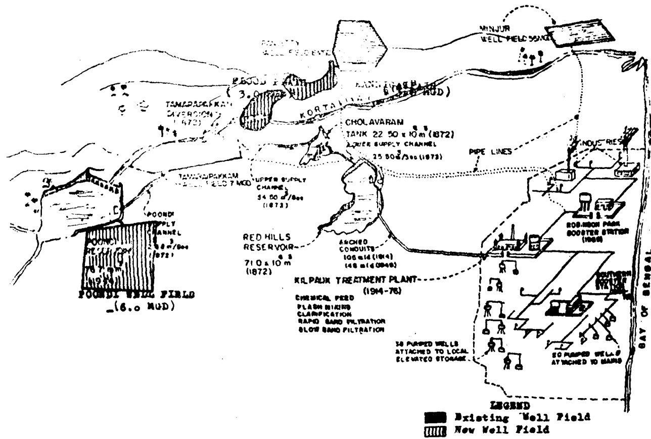
EXISTING WATER SUPPLY SYSTEM / SCHEMATIC /
