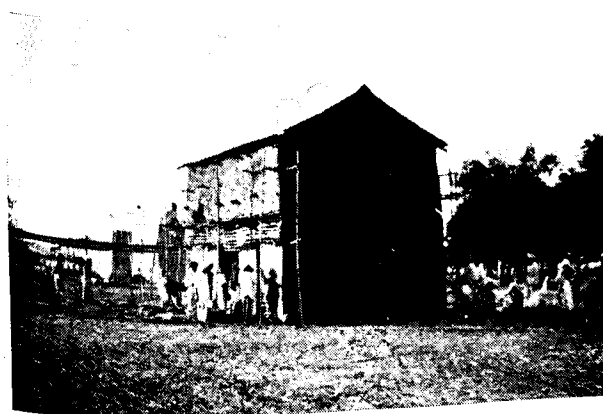
FLUE-CURING BARN
