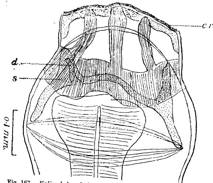
Fig. 167.— Kalicephalus fimbriatus . Anterior end of female; lateral view. c.r., corona radiata; d., duct of dorsal oesophageal gland; s., wall of buccal capsule (optical section). (After Baylis and Daubney.)
