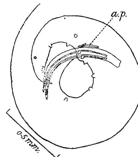
Fig. 82.— Spironoura testudinis . Posterior end of male; lateral view a.p., accessory piece. (After Baylis and Daubney.)
