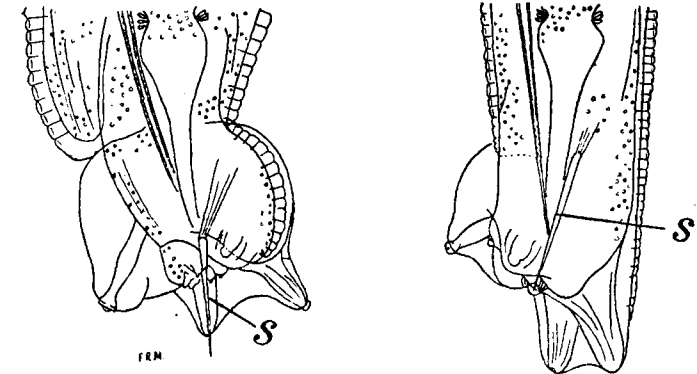
Fig. 101.— Oxyuris equi . Anterior end of female; dorsal view. (From Baylis, after Yorke and Mapleston.)
