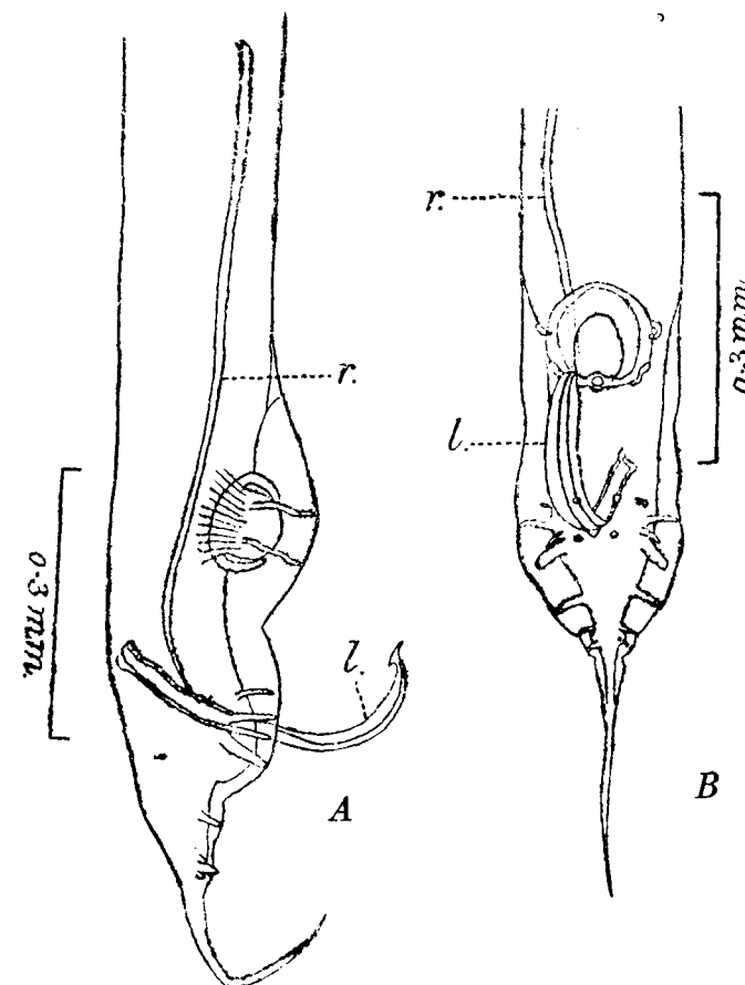
Fig. 59.— Pseudaspidotera pavonis . A, posterior end of male, lateral view; B, the same, ventral view. l. , left spicule; r. , right spicule. (After Baylis and Daubney.)
