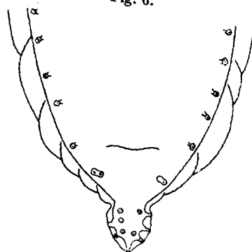
Fig. 5.— Ascaris vitulorum . Part of oesophagus and intestine. i. , intestine; m. , muscular portion of oesophagus; v. , ventriculus. (After Baylis and Daubney.) Fig. 6.— Ascaris vitulorum . Posterior end of male; ventral view. (After Boulenger.)
