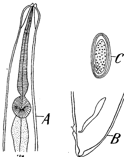
Fig. 103.— Enterobius vermicularis . A, anterior end, ventral view; B, posterior end of male, lateral view; C, egg. (From Baylis, after Yorke and Maplestone.)
