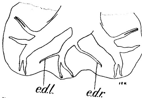
Fig. 152.— Bunostomum trigonocephalum . Anterior end; lateral view. (From Baylis, after Ransom.) Fig. 153.— Bunostomum trigonocephalum . Bursa of male; dorsal view. e.d.l. , left externo-dorsal ray; e.d.r. , right externo-dorsal ray. (From Baylis, after Ransom.)
