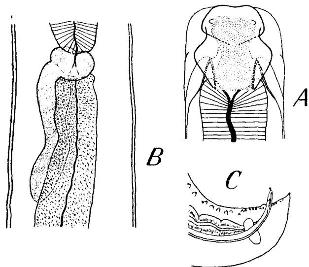
Fig. 22.— Raphidascaris diadonis . A, head, dorsal view; B, portion of oesophagus and intestine, showing ventriculus and appendix; C, posterior end of male, lateral view. (After Thwaite.)
