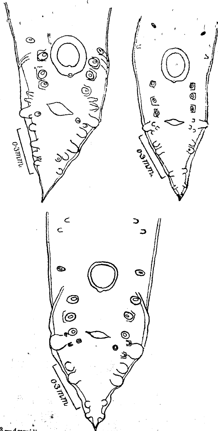
Fig. 63.— Ascaridia columbae . Posterior ends of three males; ventral view, showing variations in papillæ. (After Baylis and Daubney.)
