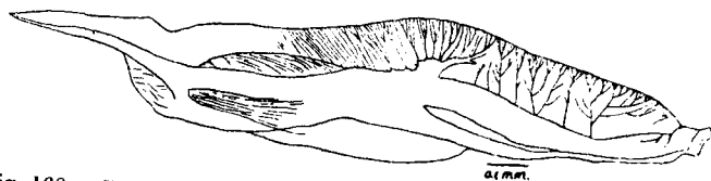
Fig. 160.— Grammocephalus varedatus . A, anterior end, lateral view; B, bursa of male, lateral view. (After Lane.) Fig. 161.— Grammocephalus varedatus . Right spicule; dorsal view. (After Lane.)
