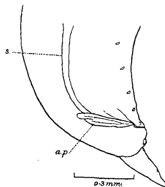
Fig. 27.— Porrocæcum reticulatum . Posterior end of male; lateral view. a.p., accessory piece; s., right spicule. (After Baylis and Daubney.)
