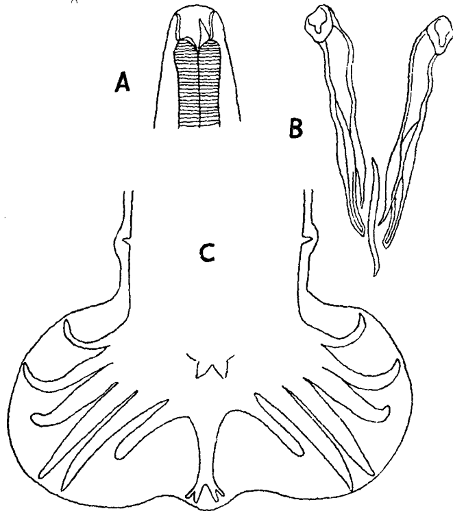
Fig. 168.— Amidostomum skrjabini . A, anterior end, lateral view; B, spicules and accessory piece, ventral view; C, bursa of male, ventral view. (After Boulenger, in 'Parasitology'.)
