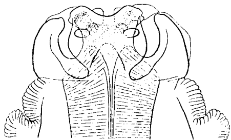
Fig. 32.— Contracæcum spiculigerum . Head of female; dorsal view. (Original.)
