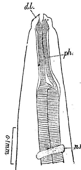
Fig. 67.— Strongyluris chamæleonis . Anterior end of female; lateral view. dl. , dorsal lip; n.r. , nerve-ring; ph. , pharynx. (After Baylis and Daubney.)
