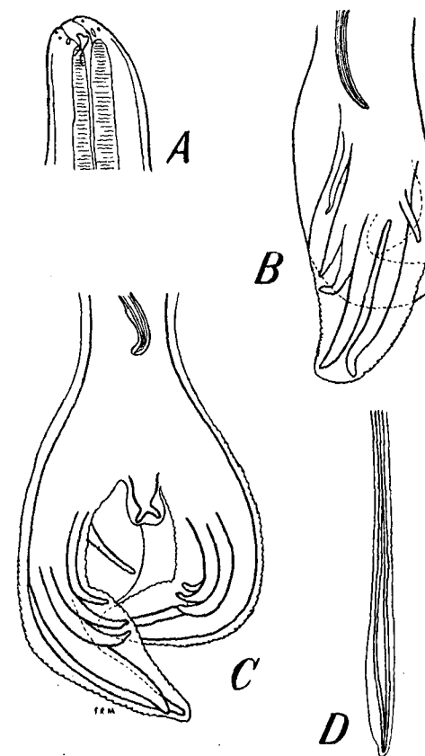
Fig. 180.— Mecistocirrus digitatus . A, anterior end, lateral view; B, bursa of male, lateral view; C, bursa, dorsal view; D, tip of spicules. (From Baylis, after Yorke and Maplestone.)
