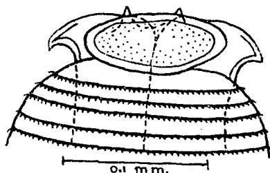
Fig. 51.—( Goezia gavialidis . Head; dorsal view. (After Maplestone.)
