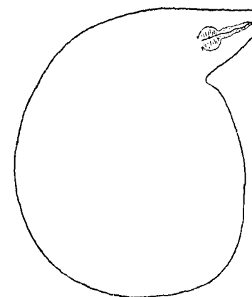
Fig. 113.— Heterodera marioni . Outline of female. (After Marcinowski.)
