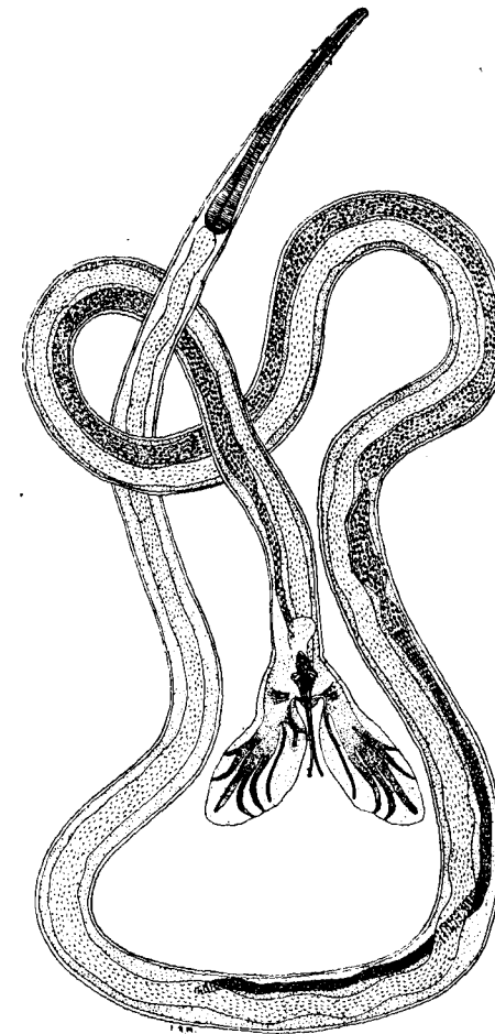
Fig. 175.— Hæmonchus contortus . Male. (From Baylis, after Neveu-Lemaire.)
