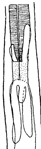
Fig. 47.— Polycæcum gangeticum . Portion of œsophagus and intestine, showing ventriculus and appendages. (After Maplestone.) Fig. 48.— Typhlophoros lamellaris . Anterior end; ventral view. (After Maplestone.)
