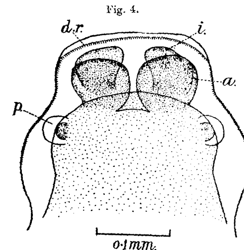
Fig. 4.— Ascaris vitulorum . Dorsal lip, viewed from exterior. a. , anterior lobe of pulp; d.r. , dentigerous ridge; i. , internal process of anterior lobe; p. , papilla. (After Baylis and Daubney.)
