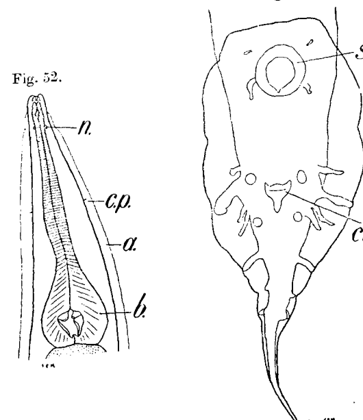
Fig. 52.— Heterakis gallinæ . Anterior end; dorsal view. a. , cervical ala; b. , oesophageal bulb; cp. , cervical papilla; n. , nerve ring. (From Baylis, after Yorke and Maplestone.)
