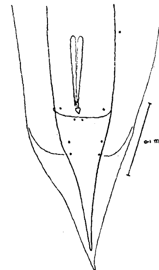
Fig. 107.— Syphaciella indica . Posterior end of male; ventral view. (After Maplestone.)
