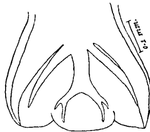
Fig. 141.— Œsophagostomum tridentatum . Bursa of male; dorsal view. (After Maplestone.)
