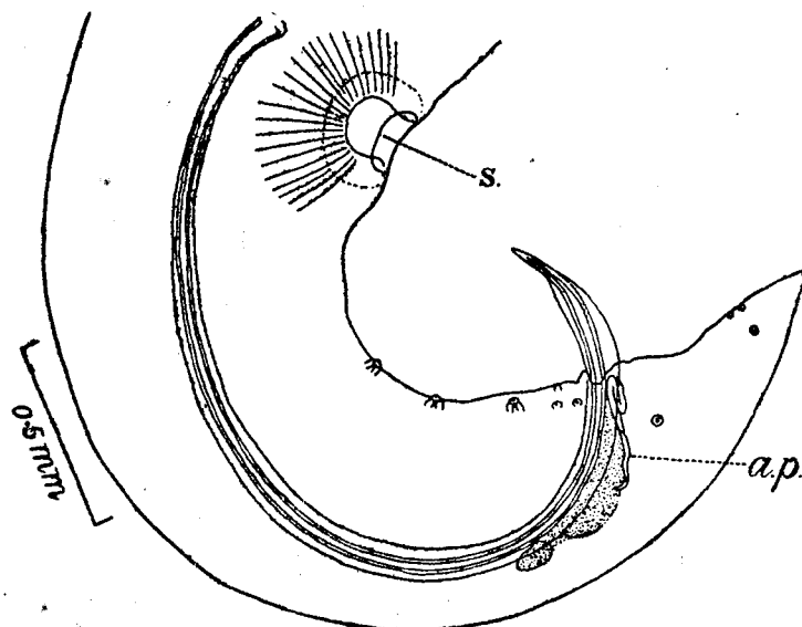
Fig. 94.— Zanclophorus kempii . Posterior end of male; lateral view. a.p., accessory piece; s., sucker. (After Baylis and Daubney.)
