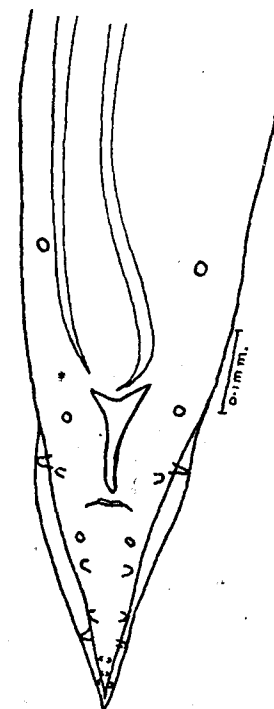
Fig. 76.— Subulura turnicis . Posterior end of male; ventral view. (After Maplestone.)
