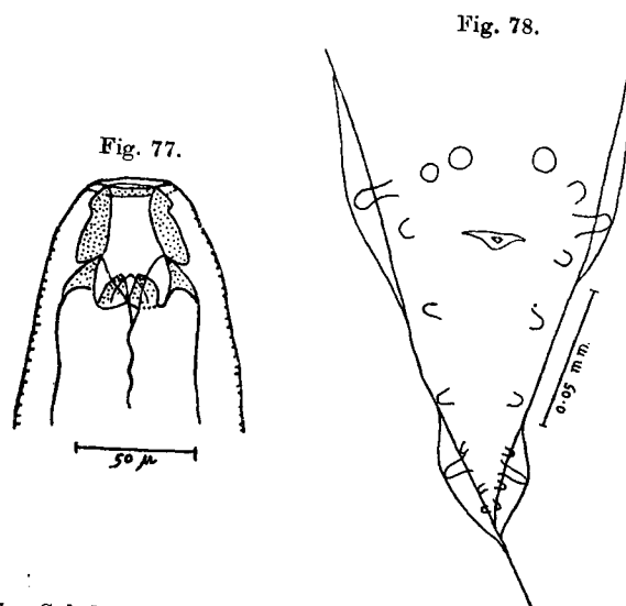
Fig. 77.— Subulura multipapillata . Head. (After Chandler.) Fig. 78.— Subulura multipapillata . Posterior end of male; ventral view. (After Maplestone.)
