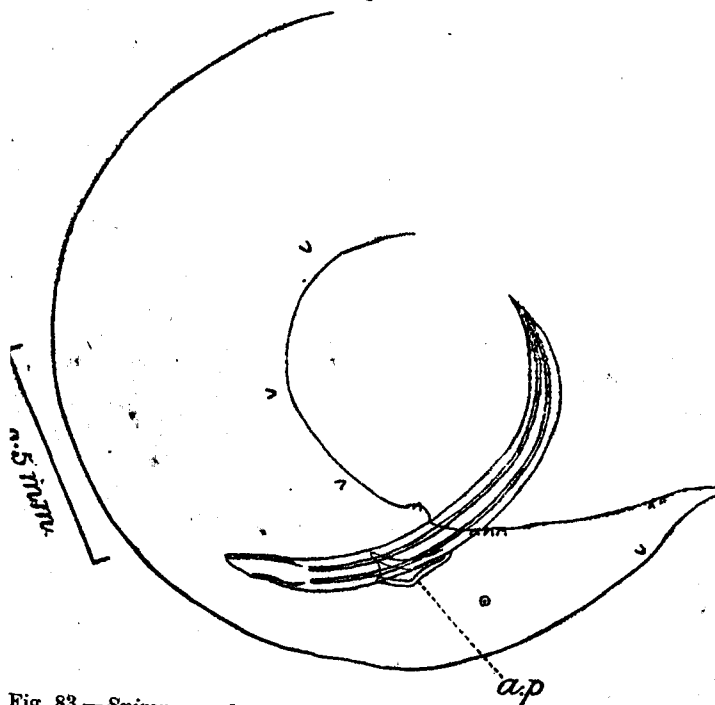
Fig. 83.— Spironoura barbi . Posterior end of male; lateral view. m. , ventral muscles; s. , sucker-like organ. (After Baylis and Daubney.)
