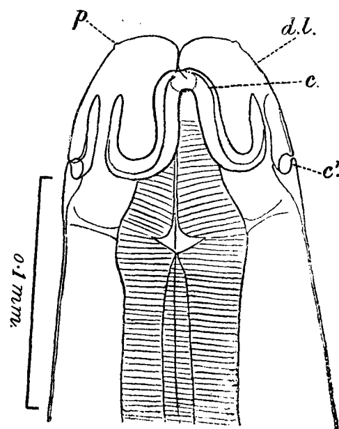
Fig. 58.— Pseudaspidotera pavonis . Anterior end of female; lateral view. c. , c' , cordons; d.l. , dorsal lip; p. , papilla. (After Baylis and Daubney.)
