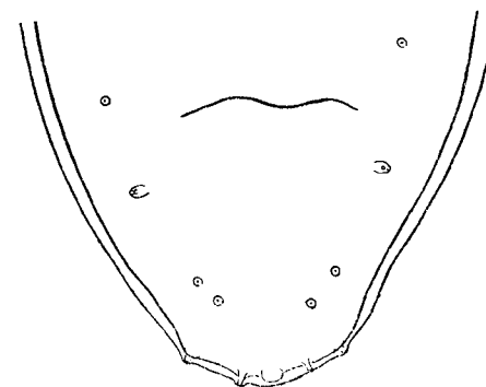
Fig. 13.— Polydelphis brachycheilos . Dorsal lip of female, viewed from exterior. (Original.) Fig. 14.— Polydelphis brachycheilos . Posterior end of male; ventral view. (Original.)
