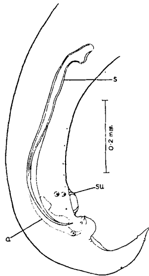
Fig. 72.— Spinicauda cophotis . Posterior end of male; lateral view. a., thickening representing accessory piece; s., right spicule; su., sucker. (After Baylis.)
