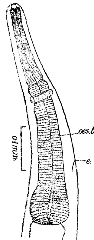
Fig. 109.— Monhysterides piscicola . Anterior end of female ; lateral view. e., excretory pore ; œs.b., œsophageal bulb. (After Baylis and Daubney.)
