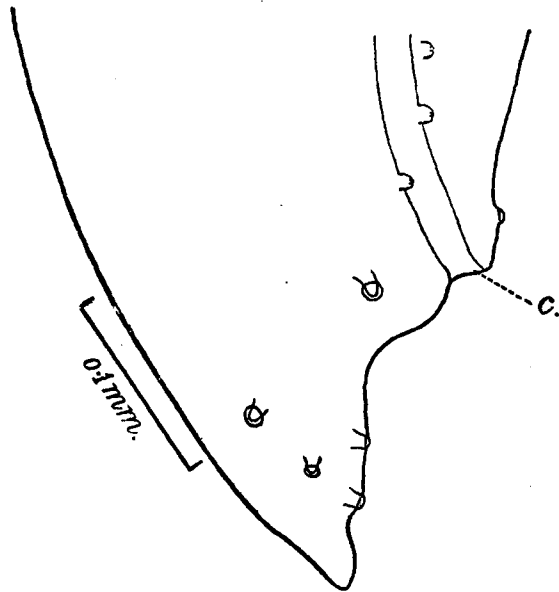
Fig. 49.— Amplicæcum varani . Head of female; dorsal view. d.r. , dentigerous ridge; g. , interlabial groove; i. , interlabium; p. , papilla. (After Baylis and Daubney.) Fig. 50.— Amplicæcum varani . Posterior end of male; lateral view. c. , cloacal aperture. (After Baylis and Daubney.)
