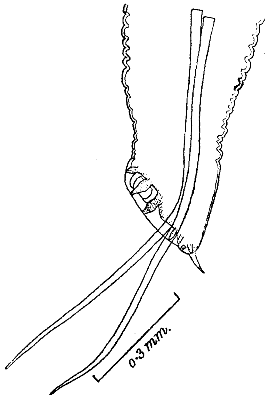
Fig. 68.— Strongyluris chamæleonis . Posterior end of male; lateral view. (After Baylis and Daubney.)
