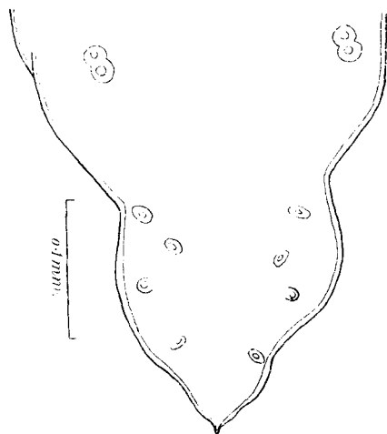
Fig. 25.— Porrocæcum angusticolle . Posterior end of male; ventral view. (After Baylis and Daubney.)
