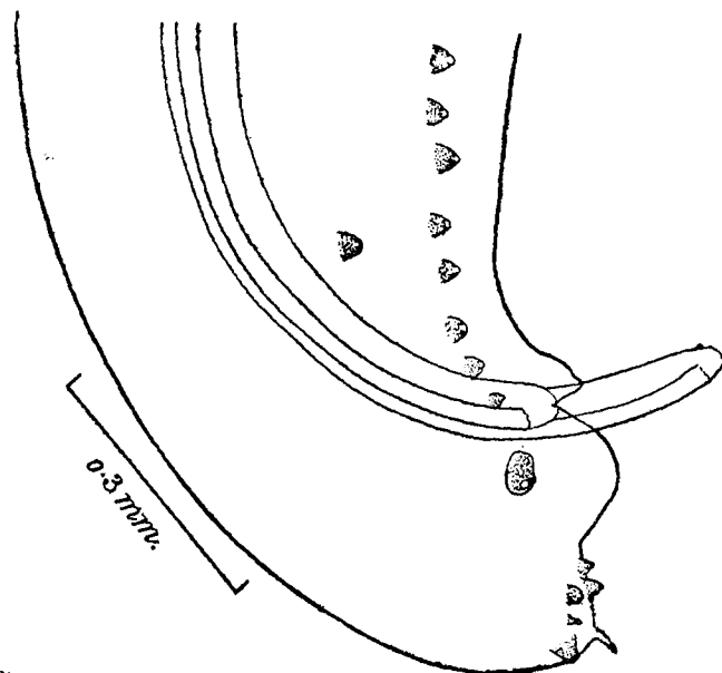
Fig. 16.— Polydelphis sewelli . Posterior end of male; lateral view. (After Baylis and Daubney.)
