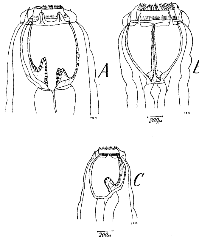
Fig. 116.—Anterior ends of three species of Strongylus . A, S. equinus , lateral view; B, S. edentatus , dorsal view; C, S. vulgaris , lateral view. (From Baylis, after Theiler.)
