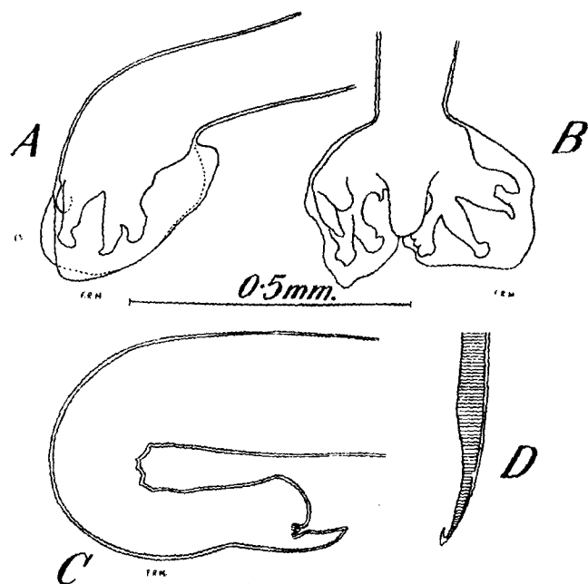
Fig. 181.— Metastrongylus elongatus . A, bursa of male, lateral view; B, bursa, ventral view; C, posterior end of female, lateral view; D, tip of spicule. (The scale refers to the figures above it.) (From Baylis, after Geddes.)
