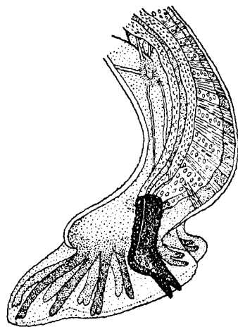
Fig. 182.— Dictyocaulus filaria . Posterior end of male; lateral view. (From Baylis, after Neveu-Lemaire.)
