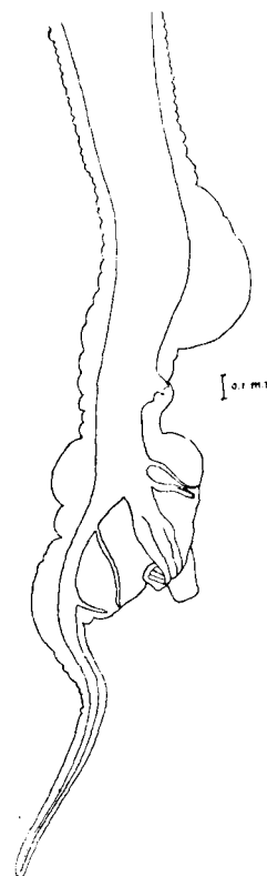
Fig. 131.— Khalilia pileata . Bursa of male; lateral view. (After Lane.)
