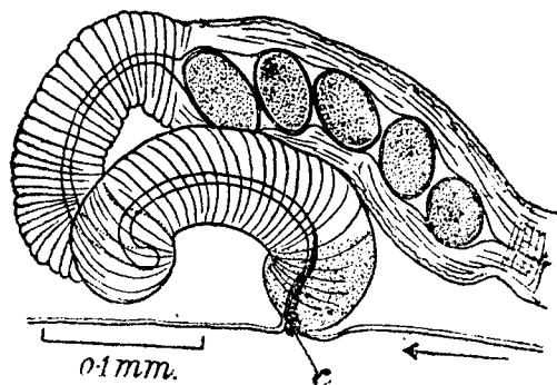
Fig. 60.— Pseudaspidodera pavonis . Vulva and vagina; lateral view. c., plug of cement in vulva. The arrow points in the direction of the head. (After Baylis and Daubney.)
