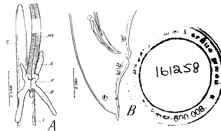
Fig. 46.— Multicæcum agile . A, portion of the alimentary canal, showing the posterior part of the œsophagus (œs.), the intestine (i.) with its cæcum (c.), and the ventriculus (v.) with its anterior (a.) and posterior (p.) appendices; B, posterior end of male, lateral view. (After Baylis, in 'Parasitology'.)
