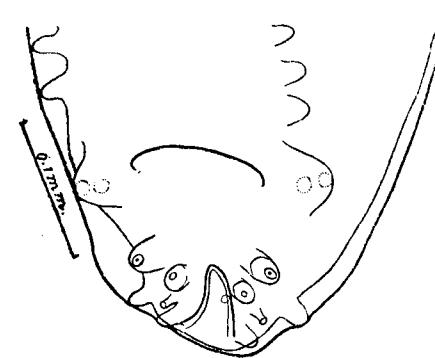
Fig. 8.— Ophidascaris naiæ . Dorsal lip of female, viewed from exterior. (After Baylis and Daubney.)
