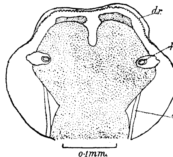
Fig. 24.— Porrocaecum angusticolle . Dorsal lip of female, viewed from exterior. c. , cuticular ridge; d.r. , dentigerous ridge; p. , papilla. (After Baylis and Daubney.)
