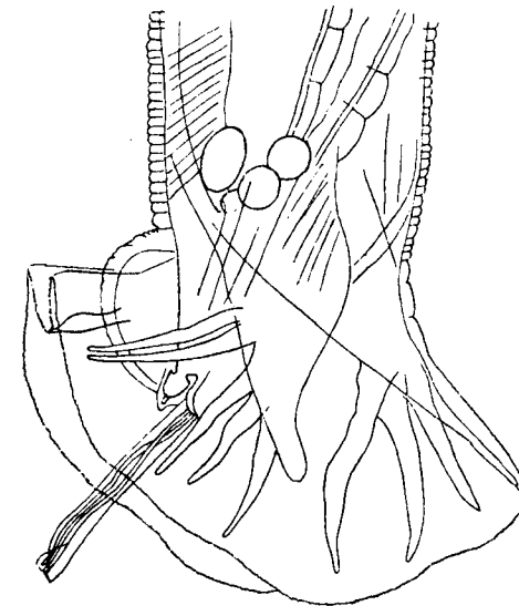
Fig. 120.— Æsophagodontus robustus . Anterior end. (After Theiler.) Fig. 121.— Æsophagodontus robustus . Bursa of male; lateral view. (After Boulenger, in 'Parasitology'.)
