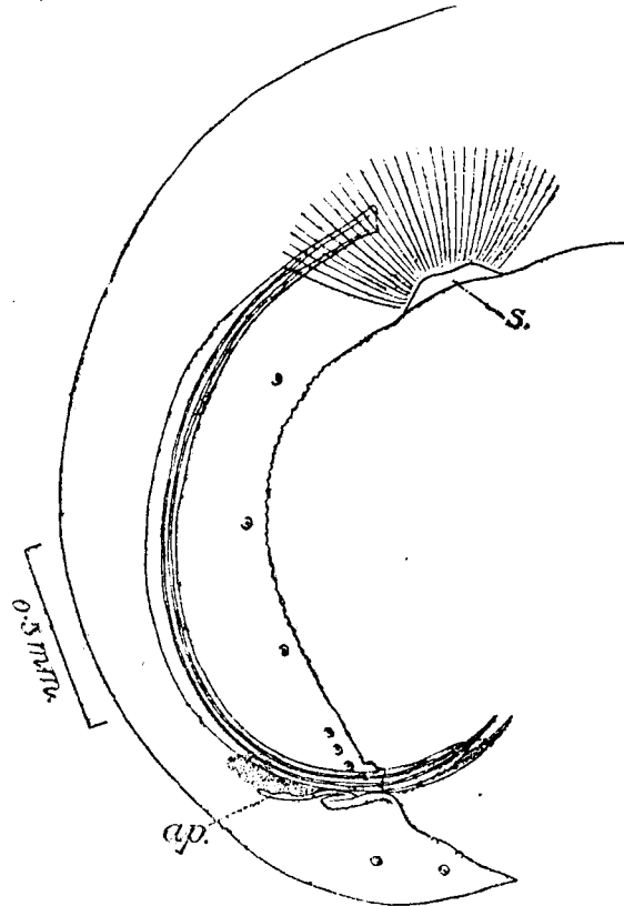
Fig. 92.— Zanclophorus annandalei . Posterior end of male; lateral view. a.p., accessory piece; s., sucker. (After Baylis and Daubney.)
