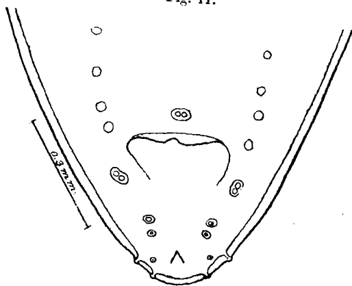
Fig. 10.— Polydelphis anoura . Dorsal lip of male, viewed from exterior. (After Baylis and Daubney.)
