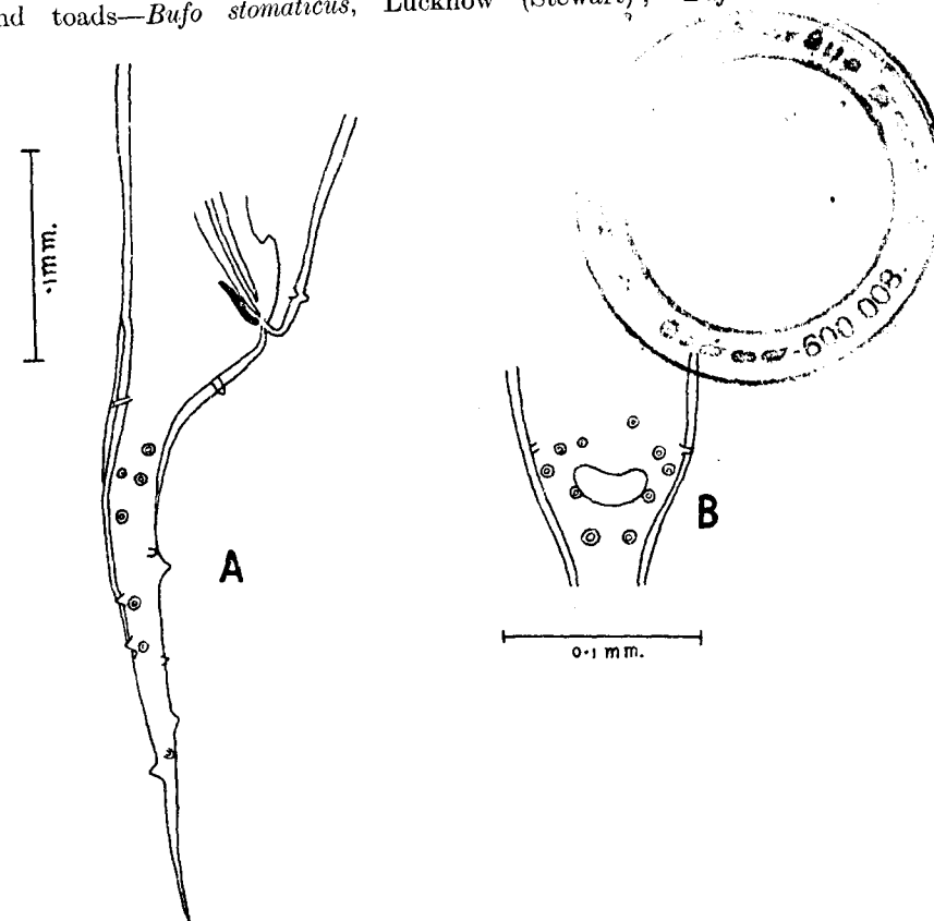
Fig. 106.— Oxysomatium macintoshii . A, posterior end of male, lateral view; B, cloacal region of male, ventral view. (After Karve.)
