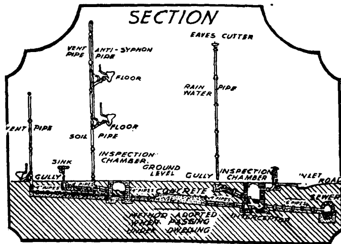
DIAGRAM OF HOUSE DRAINAGE ARRANGEMENTS.
