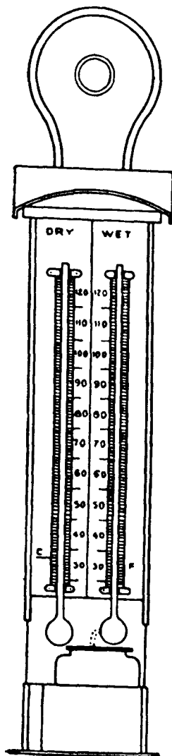
THE WET AND DRY BULB HYGROMETER.
