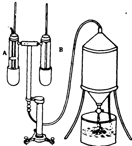
REGNAULT'S HYGROMETER.
