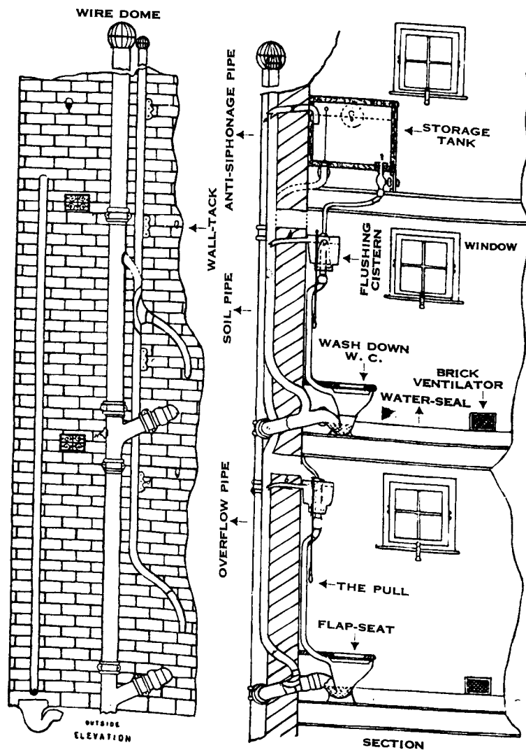
SANITARY FITTINGS
