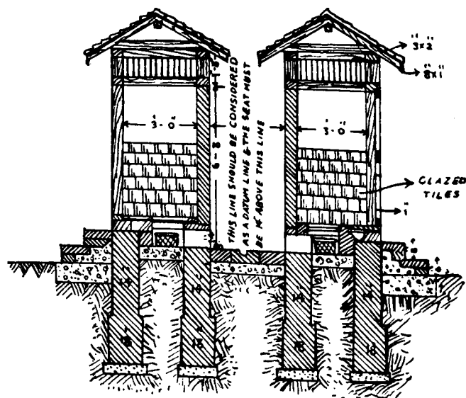
BASKET SYSTEM PRIVY—CROSS SECTION.
