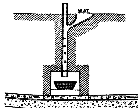
OLD FORM OF BASKET PRIVY.
