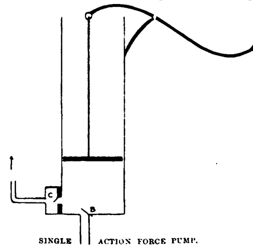
SINGLE ACTION FORCE PUMP.
