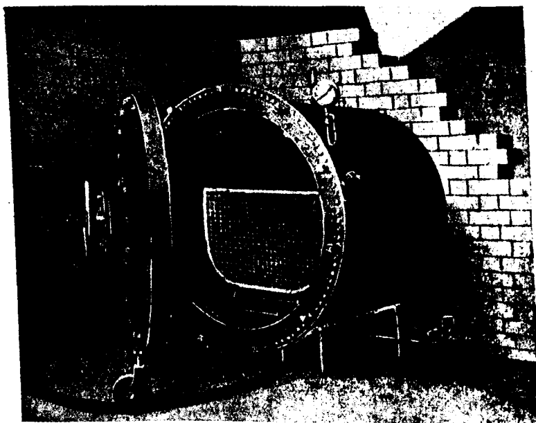
NEW TYPE THRESH CURRENT STEAM DISINFECTOR.
