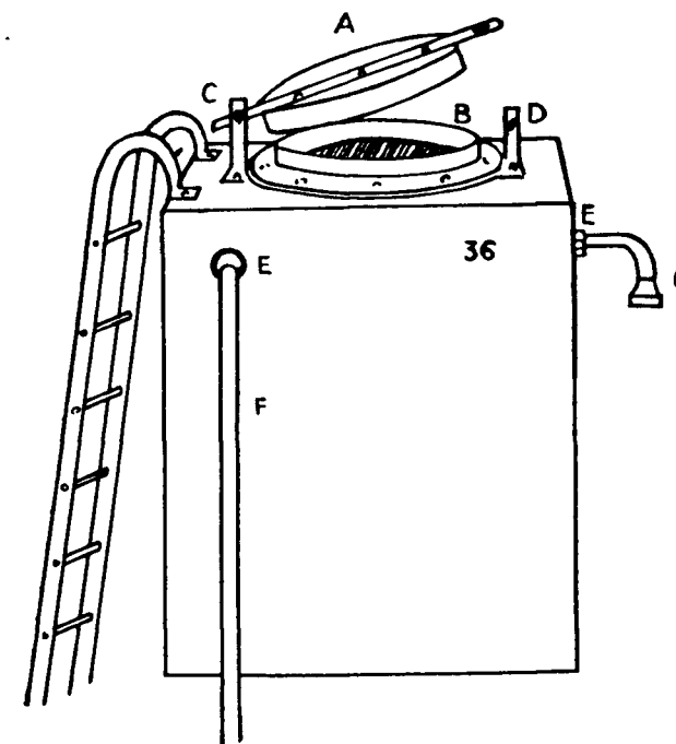
DOMESTIC CISTERN.
