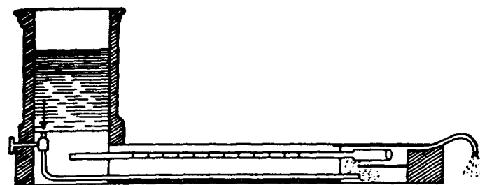
DINE'S HYGROMETER.
