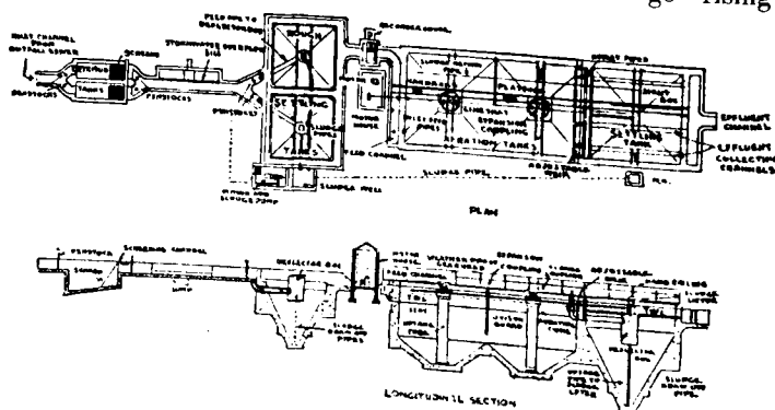
SIMPLEX PATENT SURFACE AERATION PLANT.
