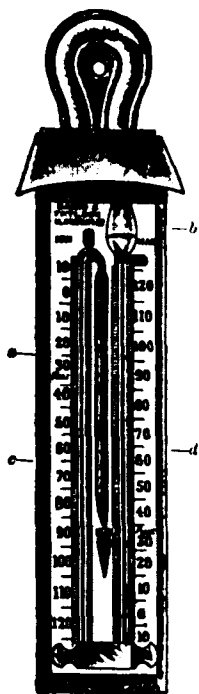
SIX'S THERMOMETER.
