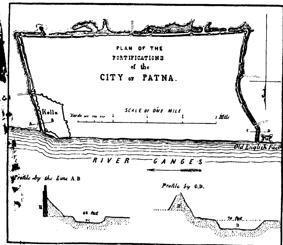
Plan of the fortifications of the City of Patna.
