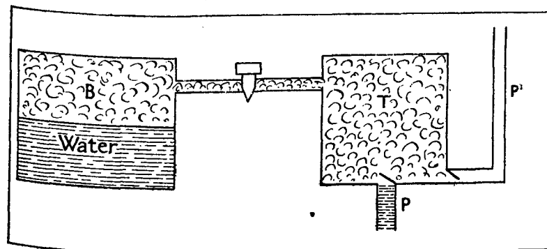
DIAGRAM OF SAVERY'S ENGINE.
