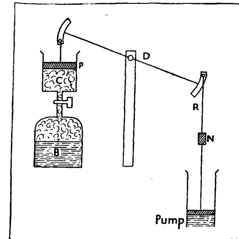
DIAGRAM OF NEWCOMEN'S ENGINE.
