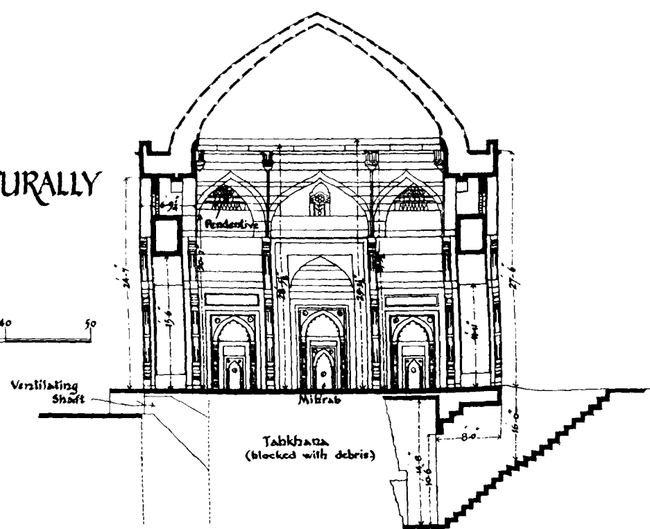
Cross Section Looking From East.
