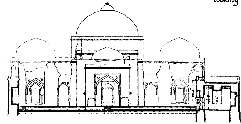
Cross Section through Line A.B.
