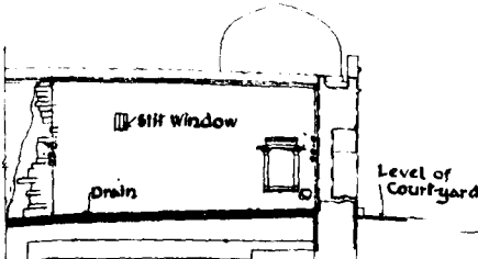
Elevation of East Block Looking from North
