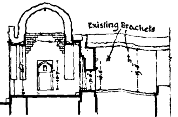
Longitudinal Section through East Block.
