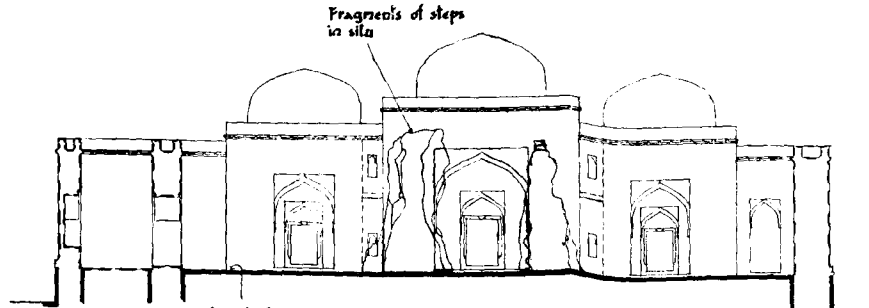
South Elevation of Front Gates to Madrasa. Looking from Courtyard.
