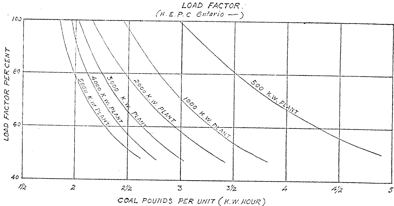
Fig. 22. COAL CONSUMPTION PER UNIT ACCORDING TO PLANT SIZE &
