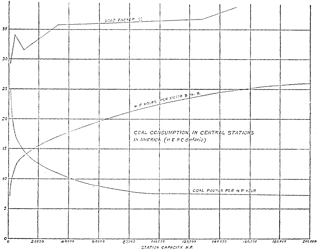
Fig. 21. Coal consumption in Central Stations.
