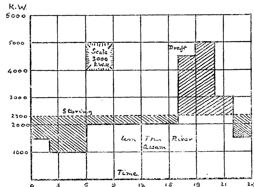
Fig. 19. Regulating Storage.
