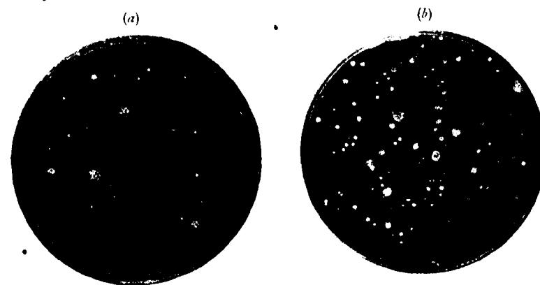
Fig. 14. Agar plates exposed for 30 minutes in a school (a) under ordinary working conditions; (b) after the children had marched out of school.
