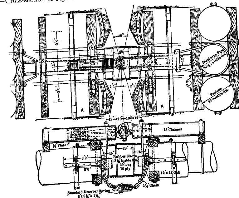
FIG. 51a.—Joints of Pipe Line.
