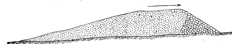
FIG. 74.—Cross-section of Gravel Spur-dikes as Built in 1882.
