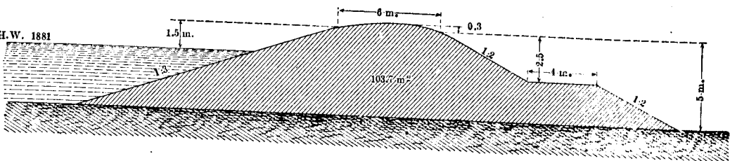
Section below Csongrad in 1888.
