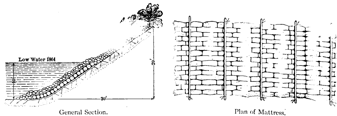
FIG. 110.—Protection Used on the Upper Mississippi River.
