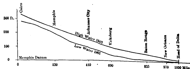
FIG. 1.—High and Low Water Profile of the Lower Mississippi River.
