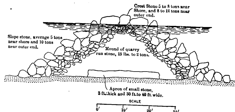
FIG. 128a.—Section of South Jetty, Aransas Pass, Texas (1911).
