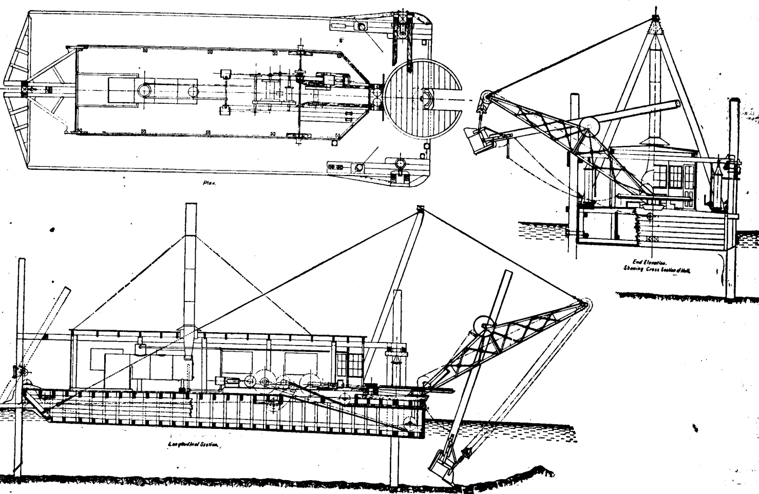
FIG. 44.—General Plan, etc., of a Two-yard Dipper Dredge.
