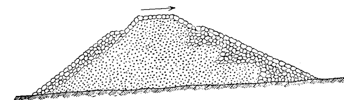
FIG. 73.—Cross-section of Spur-dikes as Built in 1885.
