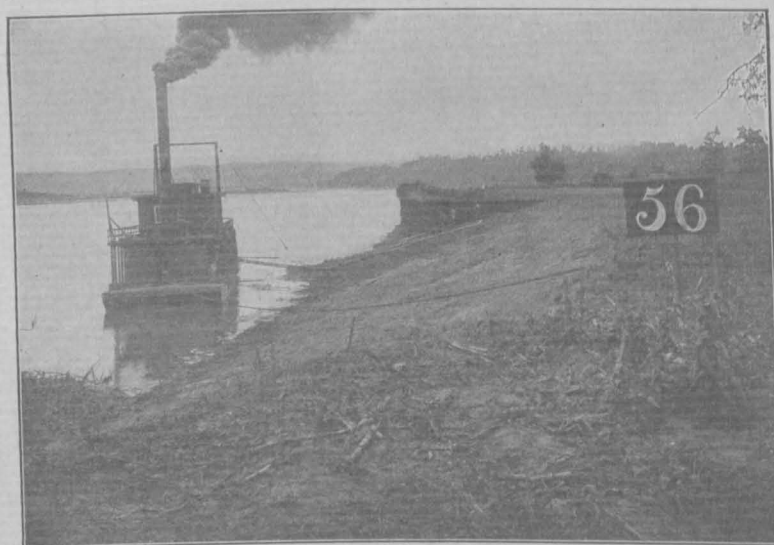
FIG. 112.—Hydraulic Grader and Party, Grading Bank for Revetment.
