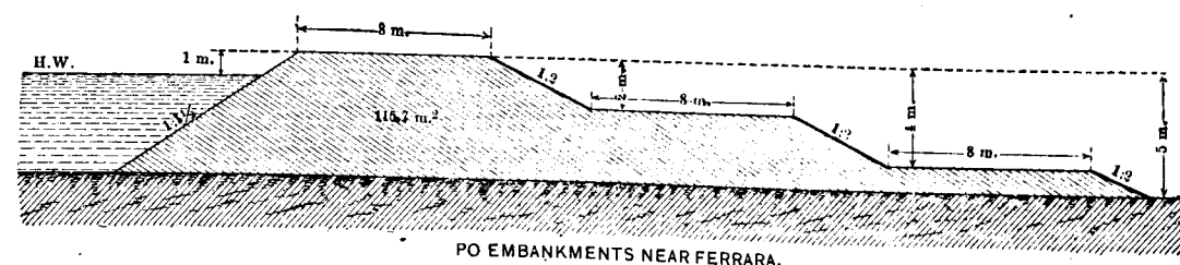
FIG. 124a.—Sections of Levees on the Loire, Rhine, and Po.
