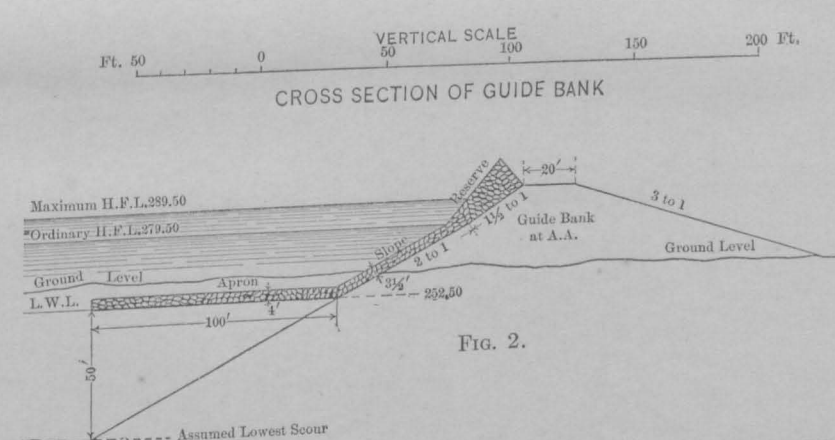
FIG. 2. BRIDGE OVER THE GANGES RIVER AT ALLAHABAD, AS ORIGINALLY PROPOSED
