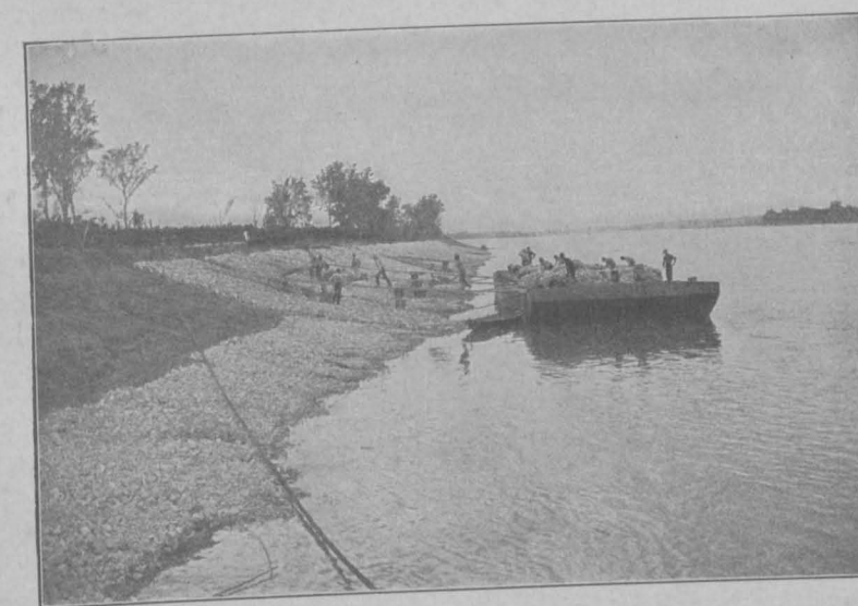
FIG. 114.—Bank Revetment, Missouri River. Party Paving Upper Bank.
