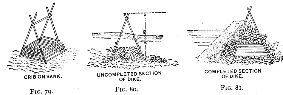
HURDLE DIKE AS USED IN INDIA.
