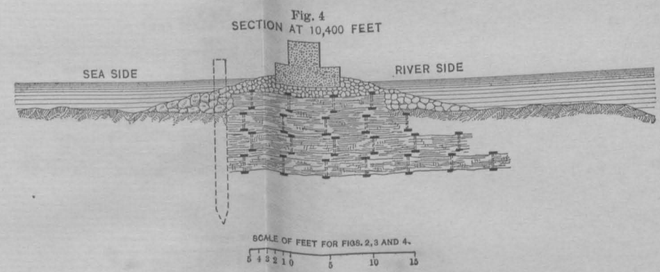
IMPROVEMENT OF SOUTH PASS, MISSISSIPPI RIVER
