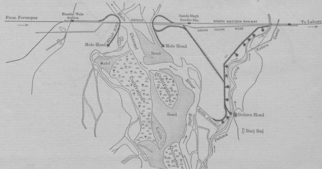
Fig. 3.-WORKS AS REMODELED AFTER FLOOD OF 1889.
