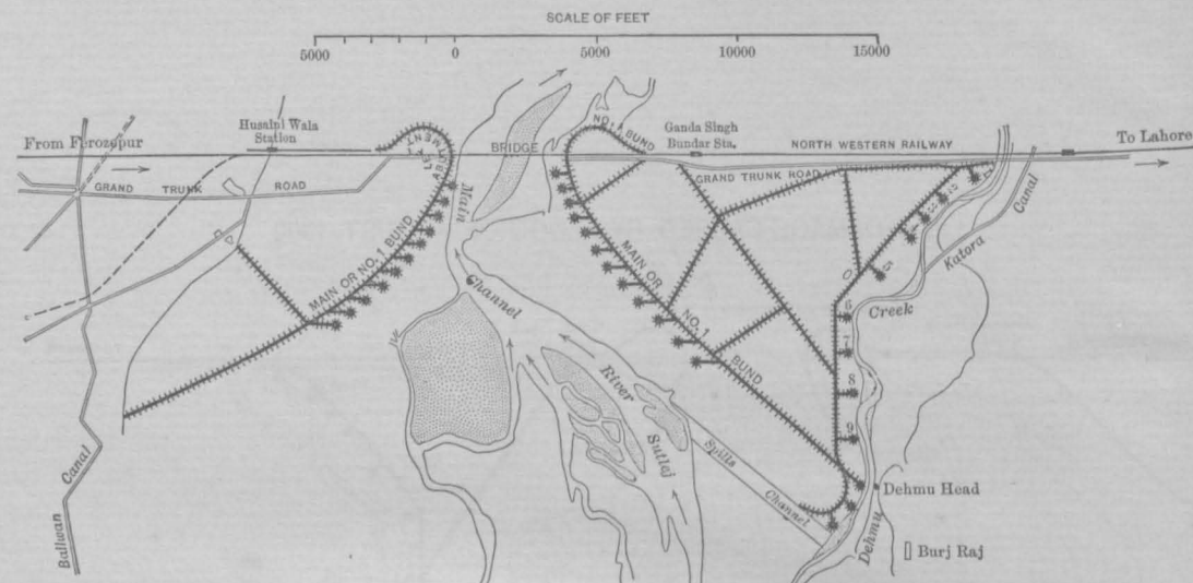
Fig.1-ORIGINAL SYSTEM OF WORKS.
