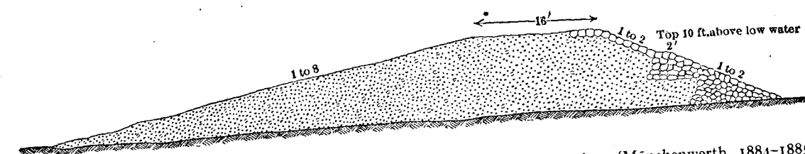
FIG. 76.—Cross-section of Training Dike Exposed to a Current on One Side only. (Mönchenwerth, 1884-1885.)
