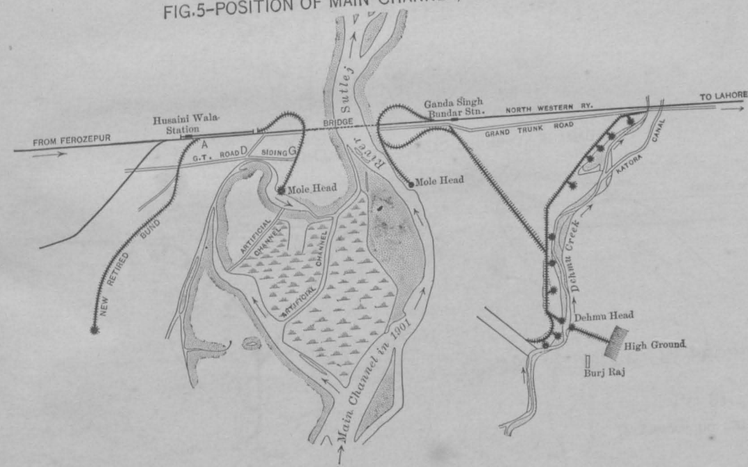
FIG.5-POSITION OF MAIN CHANNEL, DECEMBER 1901
