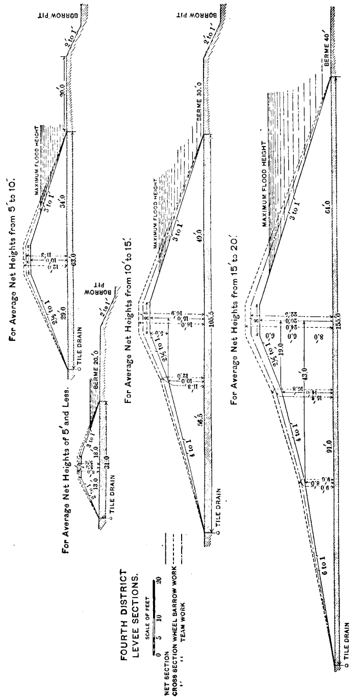
FIG. 122.—Sections of Mississippi River Levees for Various Heights.
