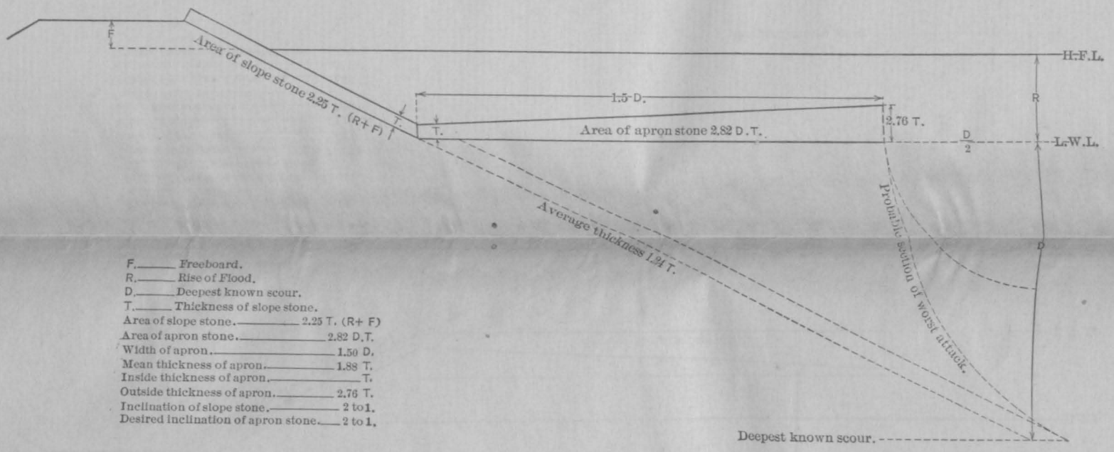
FIG. 4-DIMENSIONS OF GUIDE BANK APRONS.
