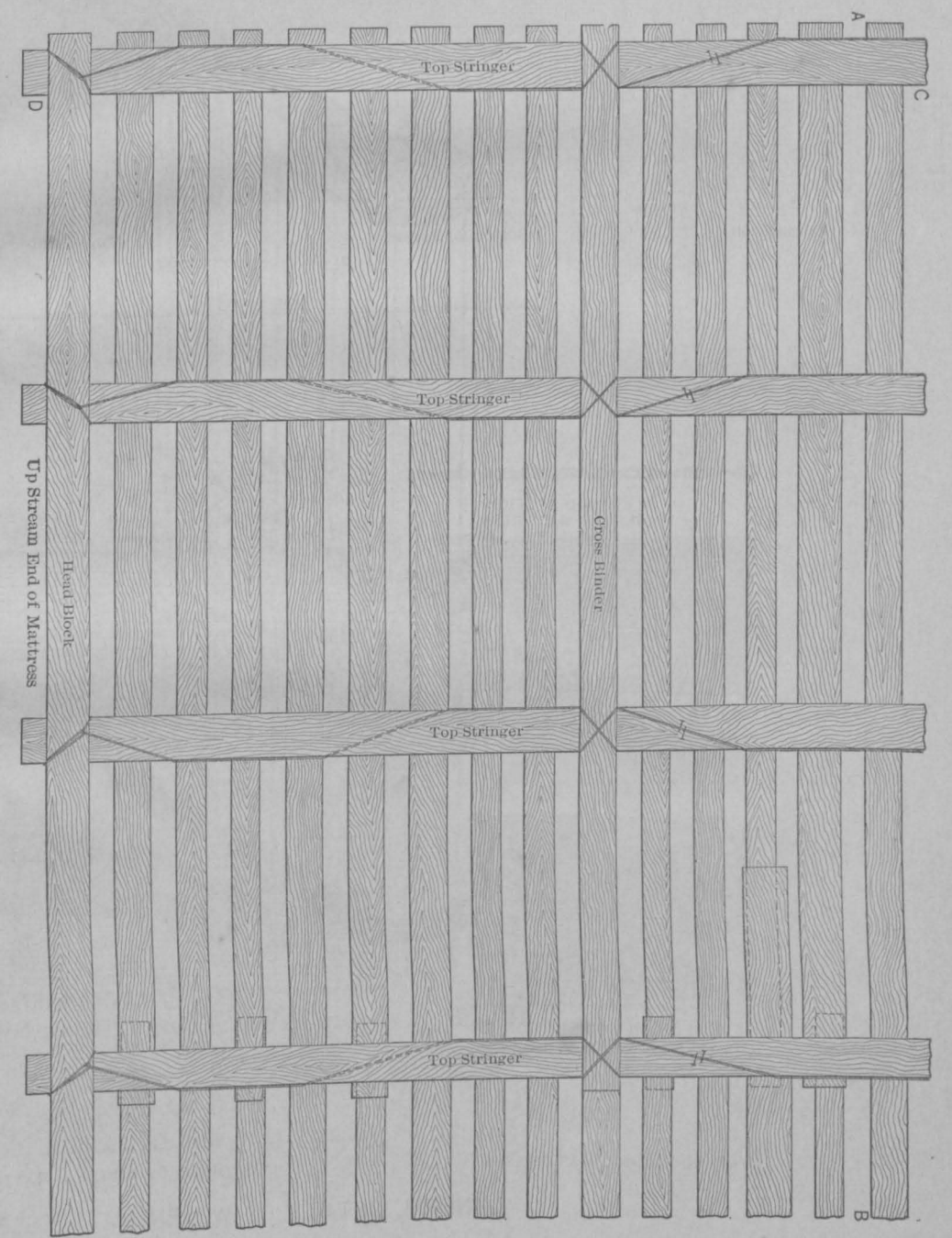
GENERAL DETAILS OF LUMBER MATTRESS.
