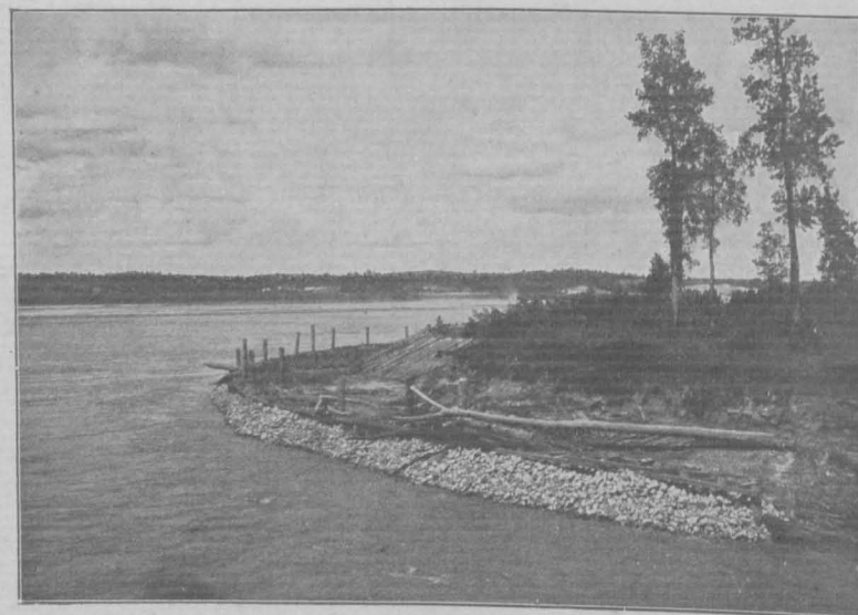
FIG. 117.—Bank-head Near Chamois, Mo., Looking Downstream, after Structure had been Exposed to the Floods Two Seasons.
