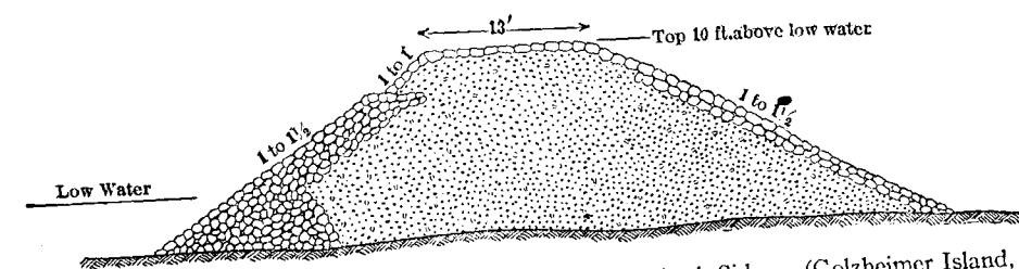
FIG. 74.—Cross-section of Gravel Spur-dikes as Built in 1882.
