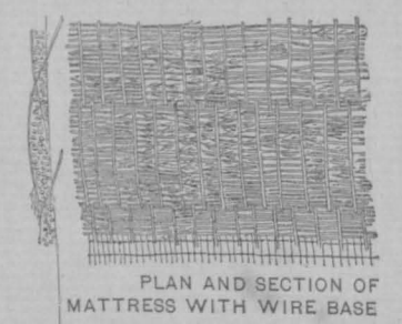
POLE AND WIRE MATTRESSES.
