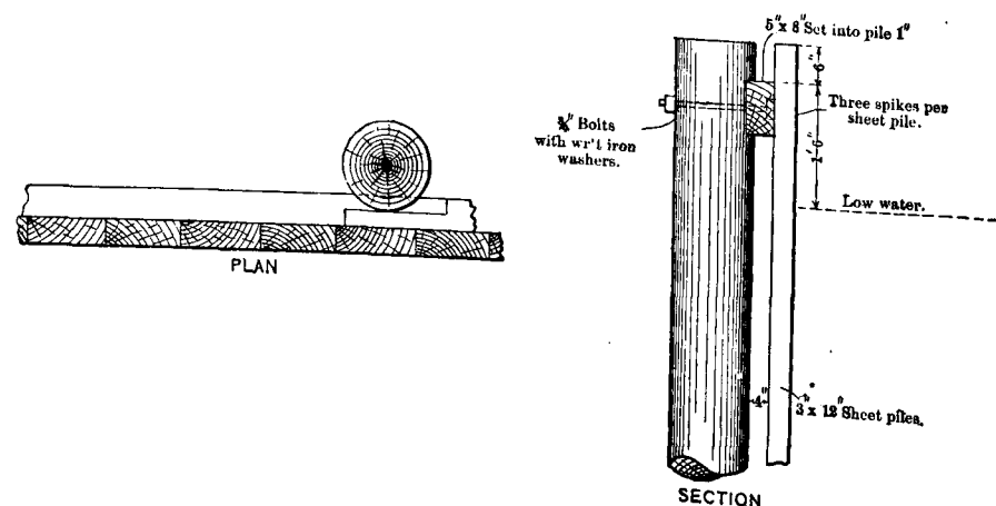
FIG. 77.—Sheet-pile Dike.
