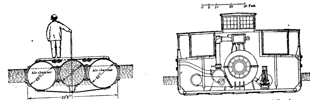
FIG. 51.—Cross-section of Pipe Line.
