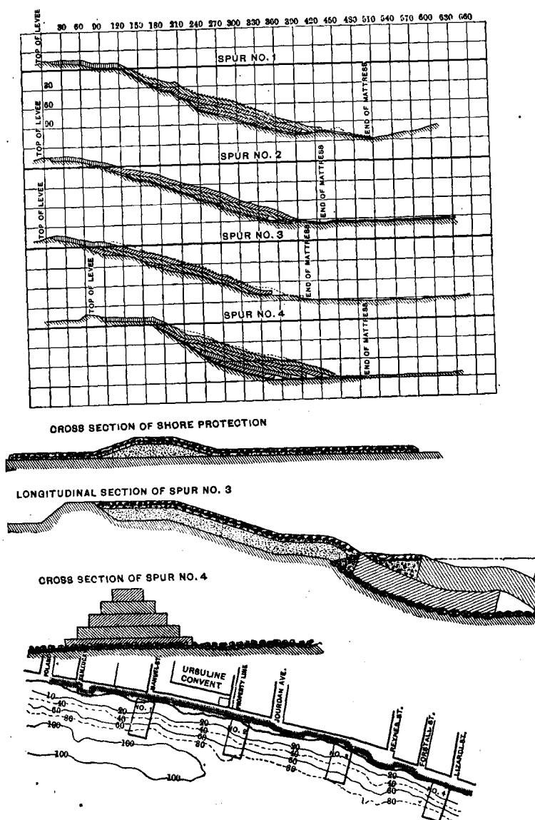
FIG. 109.—New Orleans Spur Revetments. (For Bank Protection.)
