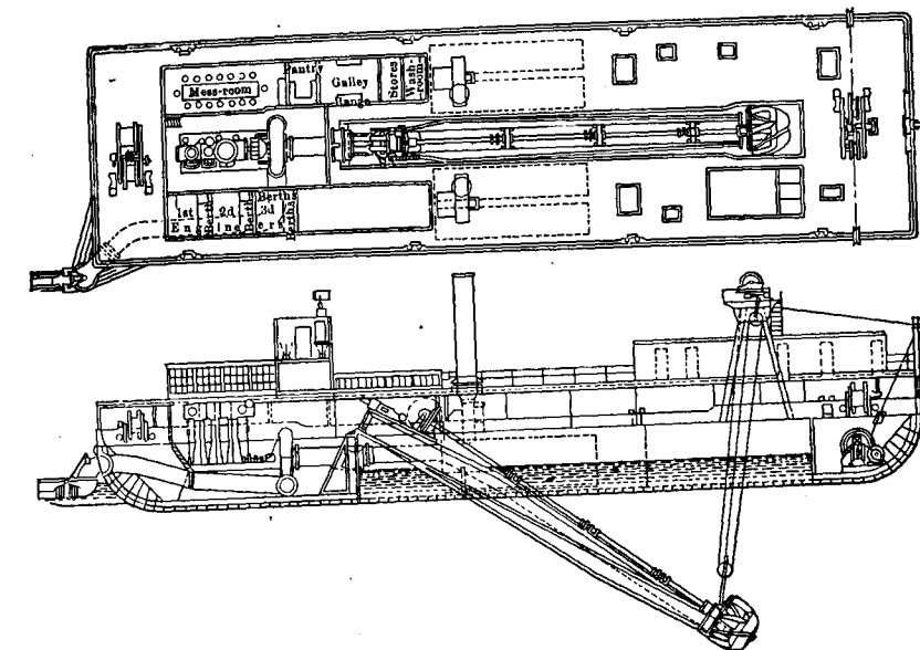
FIG. 50.—Plan and Sectional Elevation of Dredge.
