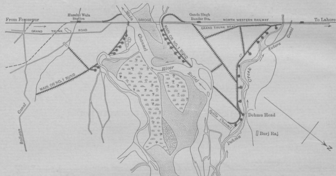
Fig.2-DAMAGE TO BUNDS CAUSED BY FLOOD OF JULY 1889.
