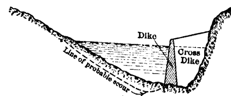
SECTION THROUGH A BEND WITH LONGITUDINAL & CROSS DIKES
