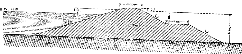
Section above Csongrad in 1888.
