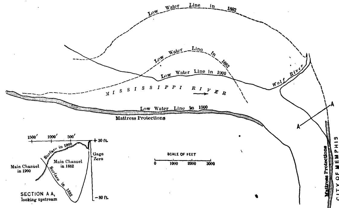
FIG. 5a.—Changes in the Mississippi River at Memphis, Tenn.
