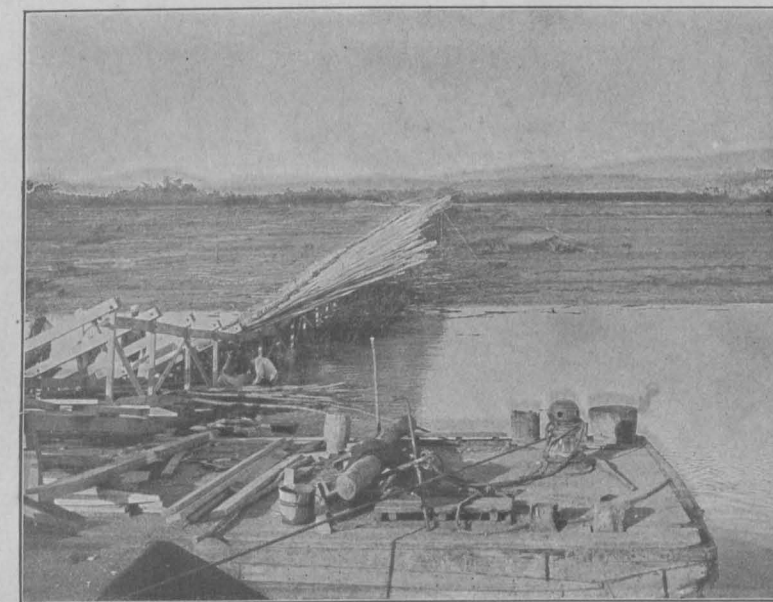
FIG. 89.—Method Used in Building a Continuous Abattis Over Water. Looking Inshore.
