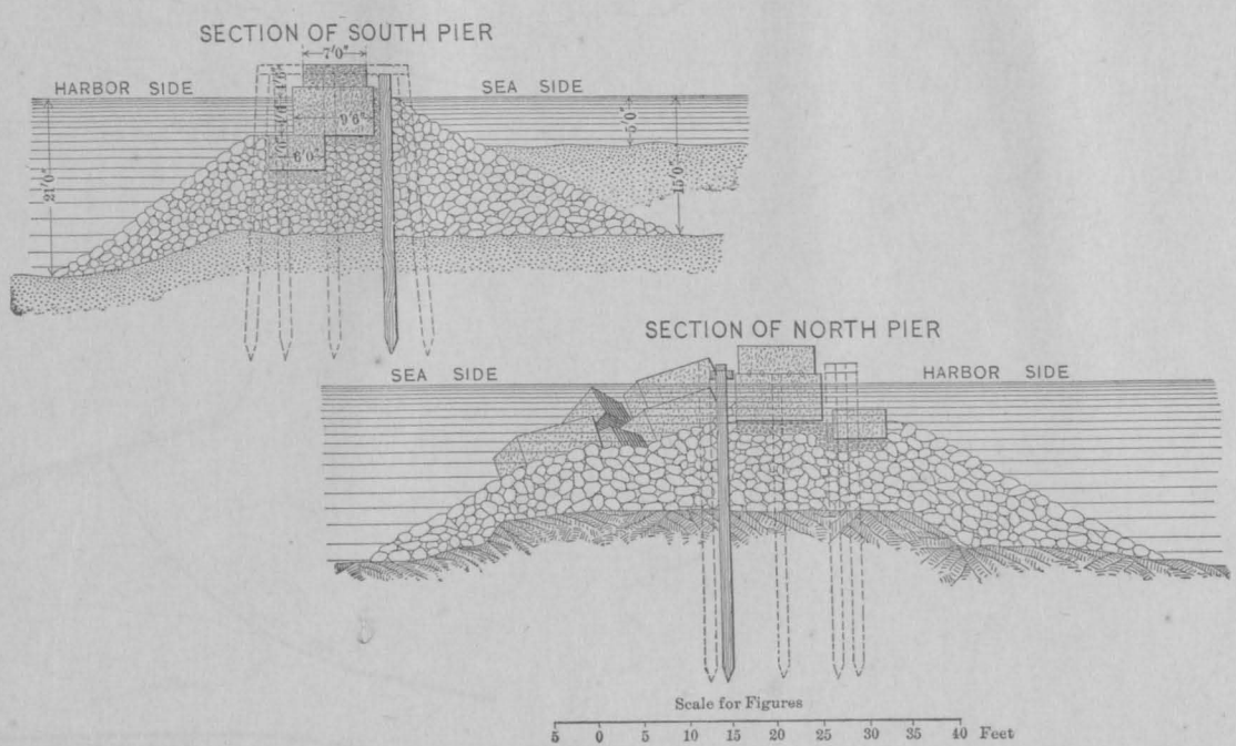
IMPROVEMENT OF THE SULINA MOUTH OF THE DANUBE.
