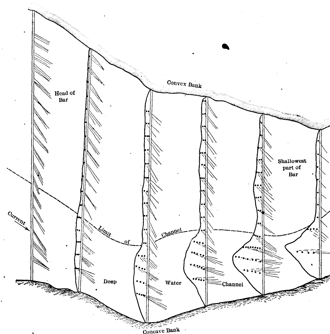
FIG. 3a.—Illustrating the Movements of Threads of Flowing Water. From a photograph of a model by M. N. de Lelavski, based on observations by floats on the Dniéper River in 1902. The movements were represented by pins placed in pieces of glass which were shaped to conform to the water surface and to the contours of the bed.
