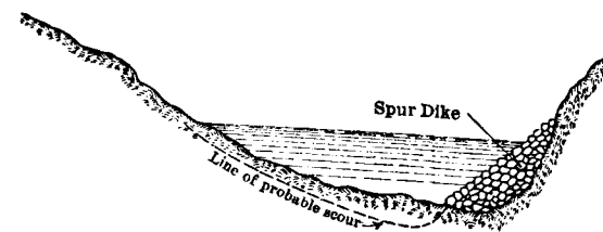
SECTION THROUGH A BEND WITH SPUR DIKES
