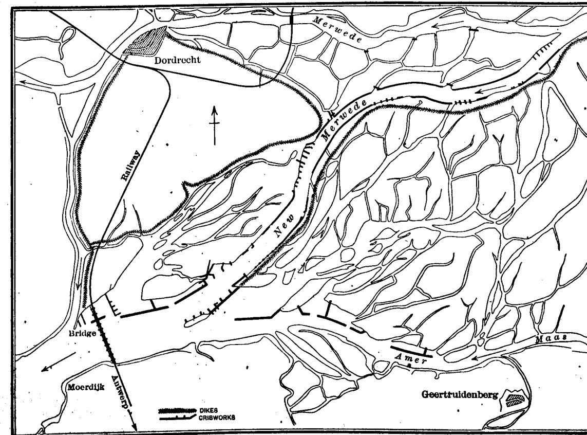
FIG. 28.—Comparative Plans Showing the Improvements of the Merwede Outlet of the Rhine.
