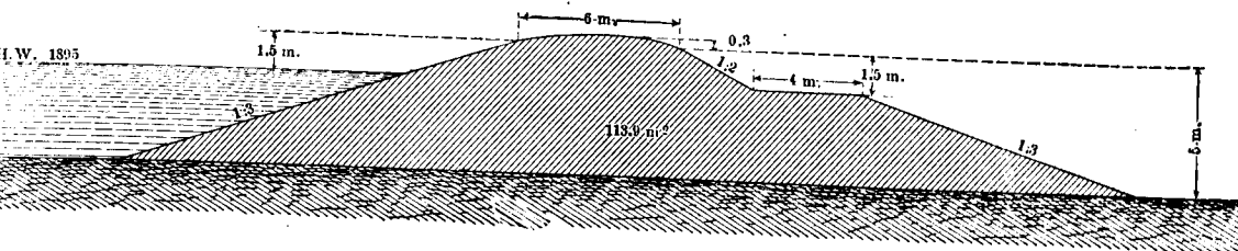
Maximum Section in 1895.
