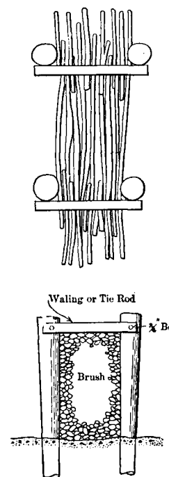
FIG. 78.—Plan and Section of Brush and Pile Dike.
