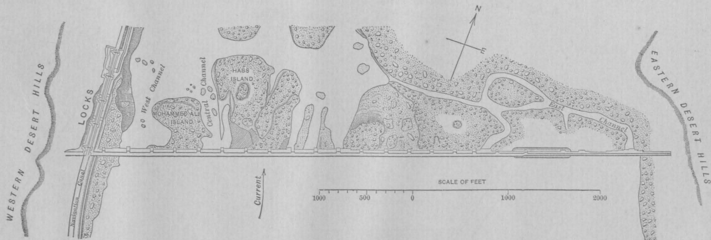
FIG. b-GENERAL PLAN OF THE ASSUAN DAM, WITH RESERVOIR FILLED
