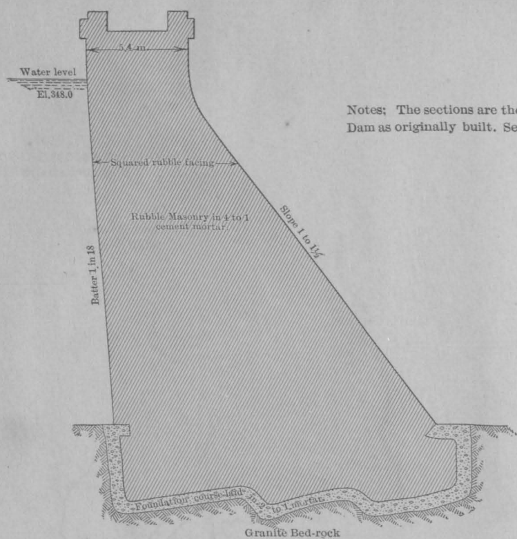
Fig. c-SECTION OF SOLID DAM
