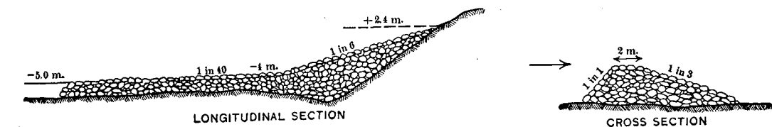
FIG. 82—Submerged Sill.
