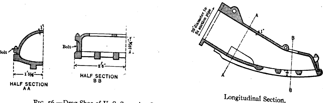
FIG. 56.—Drag Shoe of U. S. Sea-going Suction Dredges, New York Harbor Entrance.
