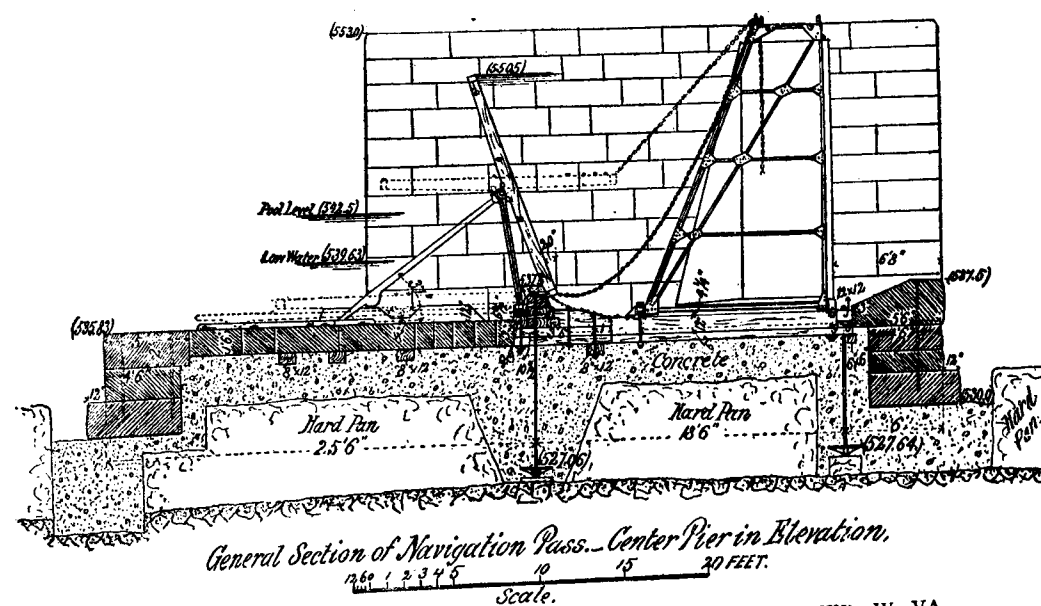
SECTIONS, ETC., OF PASS AND WEIR, DAM NO. 7, KANAWHA RIVER, W. VA.
