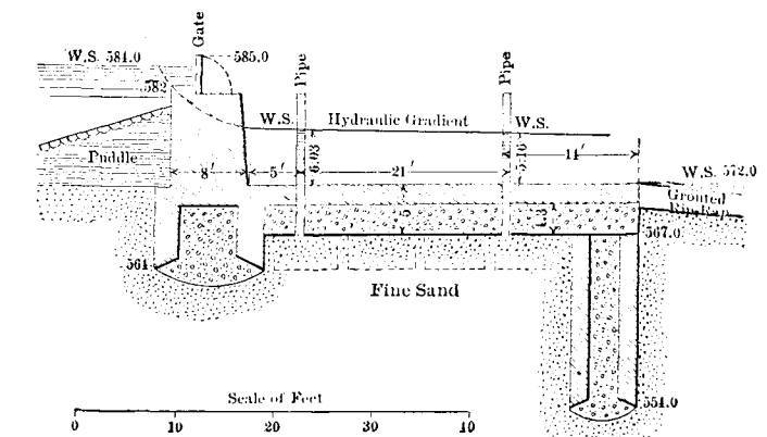
FIG. 197.—Cross-section of the Narora Weir, River Ganges. Head, 12 Feet.
