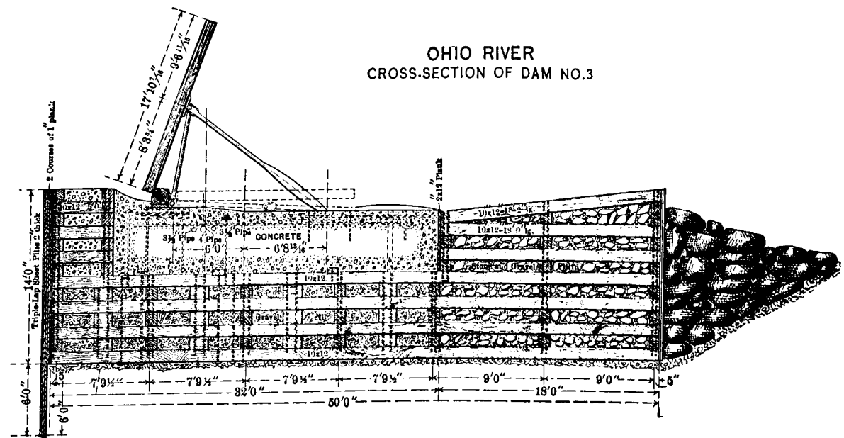
FOUNDATIONS OF OHIO RIVER DAMS (See also Pl. 54.)
