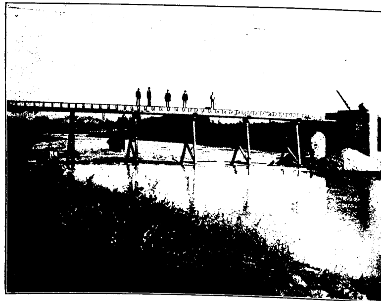
Pass Trestles from Above, Showing Escape-bars and Footway.
