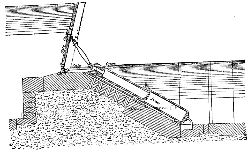
FIG. 229.—Section of a Girard Shutter.
