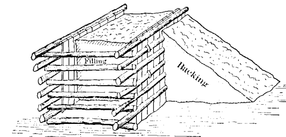
FIG. 134.—Crib Cofferdam Built of Logs.
