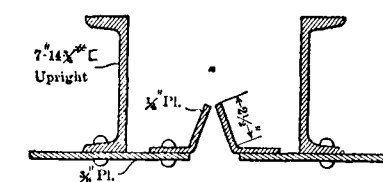
FIG. 209a.—Horizontal Section through Two Adjoining Wickets.
