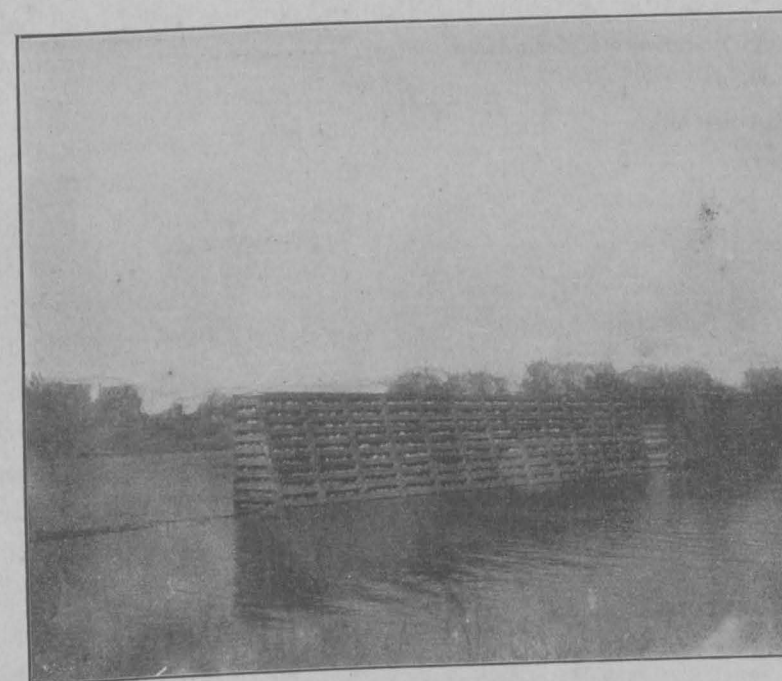
Rear View of a Lower Land Guide Crib of Timber
