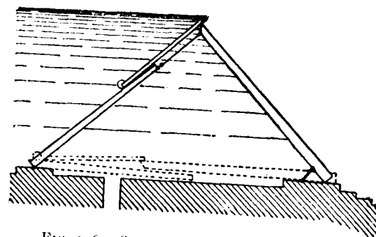
FIG. 236.—Section of Lang Bear-trap Dam.
