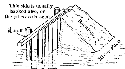
FIG. 132.—Pile Cofferdam, Single Row.
