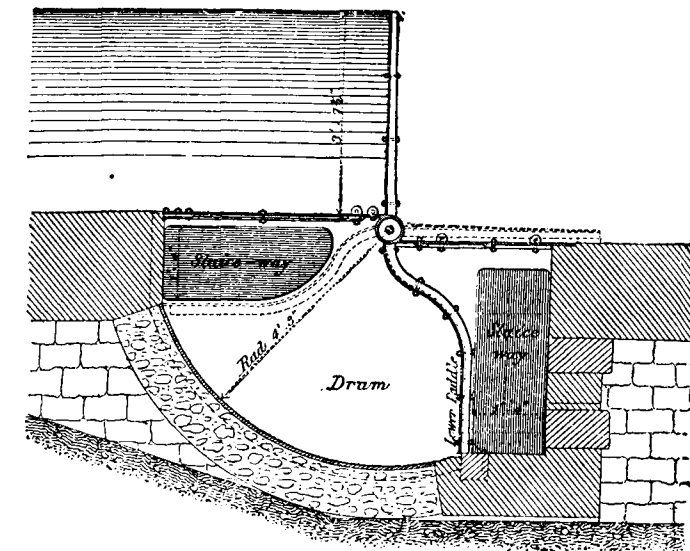
FIG. 231.—Section of Desfontaines Drum Dam, River Marne. (1867.)
