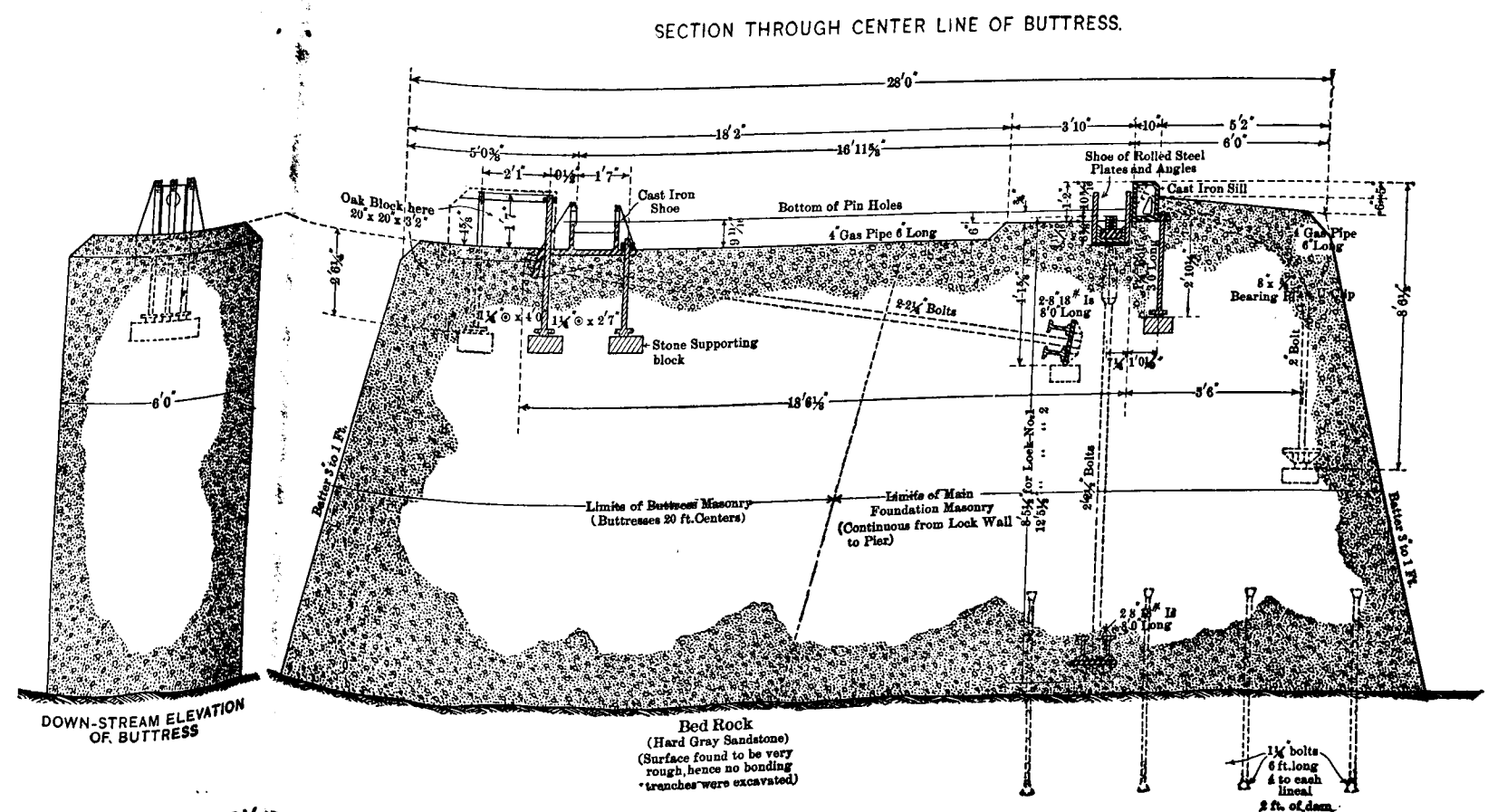
DAM NO. 1, BIG SANDY RIVER, W. VA. AND KY. DETAILS OF FOUNDATIONS AND SUPERSTRUCTURE.
