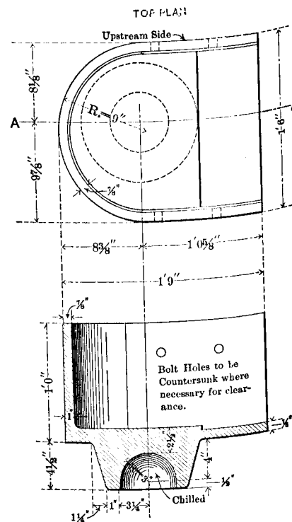
CAST SHOE FOR AN 18-INCH GATE.
