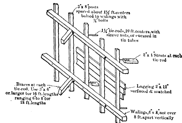
FIG. 167.—General Framing of Form with Outside Braces.
