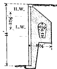
FIG. 161.—Section of Lock Wall, Harbor of St. Nazaire, France. (1906.)
