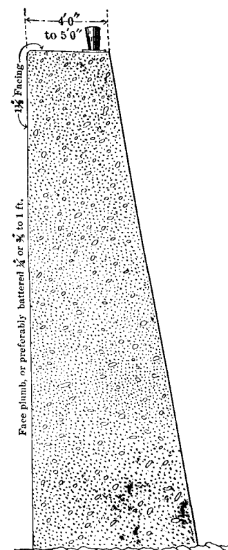
SECTION OF CONCRETE GUARD CRIB (FOR RIVER SIDE) For Guide Cribs wider bases are used if there is earth behind.
