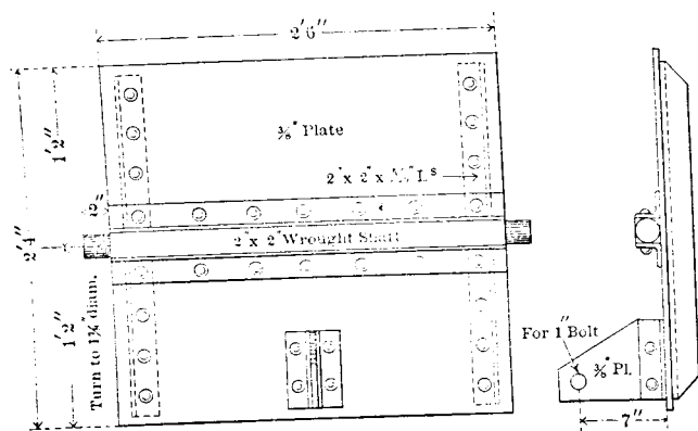
ELEVATIONS OF STEEL VALVE. (of size for high lifts.)
