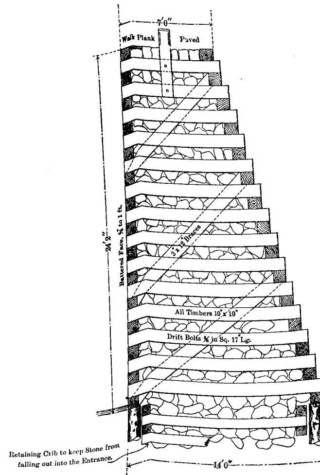
ELEVATION AND SECTION OF ORDINARY CRIB.
