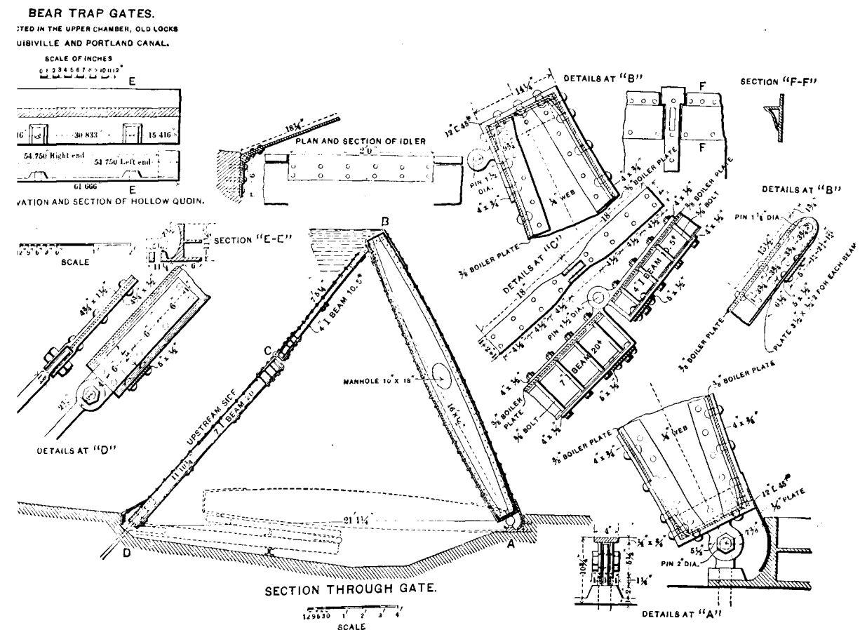
FIG. 237.—Bear-trap at Louisville, Ky., 1896. (Direct Parker Type. Depth about 15 Feet on the Sill.)
