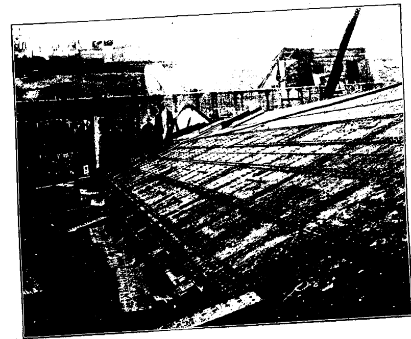
Bear-trap Dam with Steel Sheathing.
