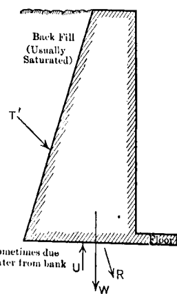
FIG. 152.—Conditions for Land Wall during Construction.
