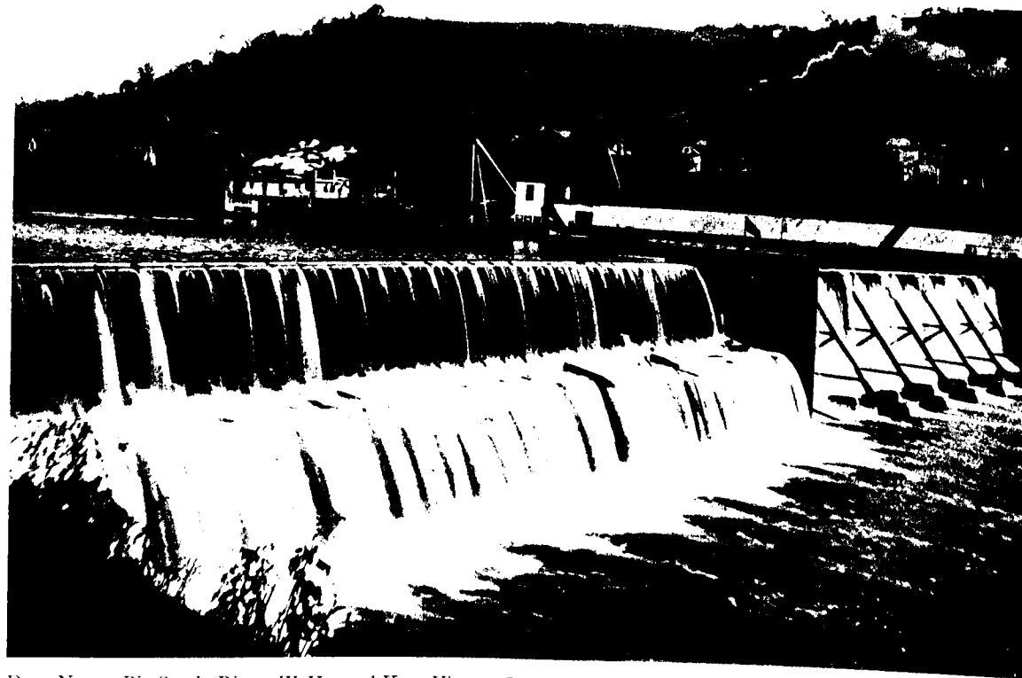
Dam No. 1, Big Sandy River, W. Va. and Ky. View at Low Water. Total Head above Sill of Needle Pass 18 Feet (this dam sustains at low water the greatest head of any needle dam yet built); against lock gates, 22½ feet. There is practically no leakage.
