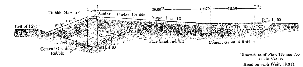
FIG. 199.—Damietta Weir, River Nile, 418 Meters Long. (1901.)
