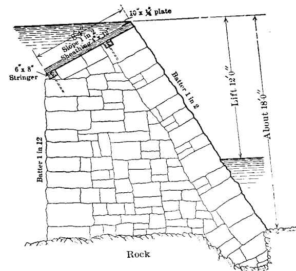
RUBBLE MASONRY DAM. (No. 4, Black Warrior River, Alabama. 1902.) Length 640 ft. laid in Portland Cement mortar.
