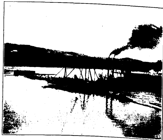
View of Weir of Dam No. 6, Kanawha River, W. Va., Illustrating the Effect of Drift on Trestles of Movable Dams.
