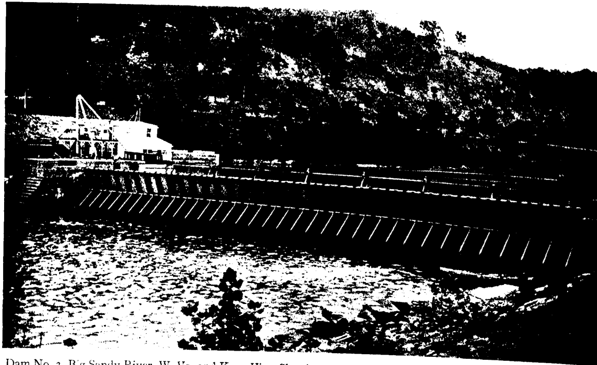
Dam No. 3, Big Sandy River, W. Va. and Ky. View Showing the Weir Reconstructed with Steel Chanoine Wickets, (1908). (See also p. 567.)
