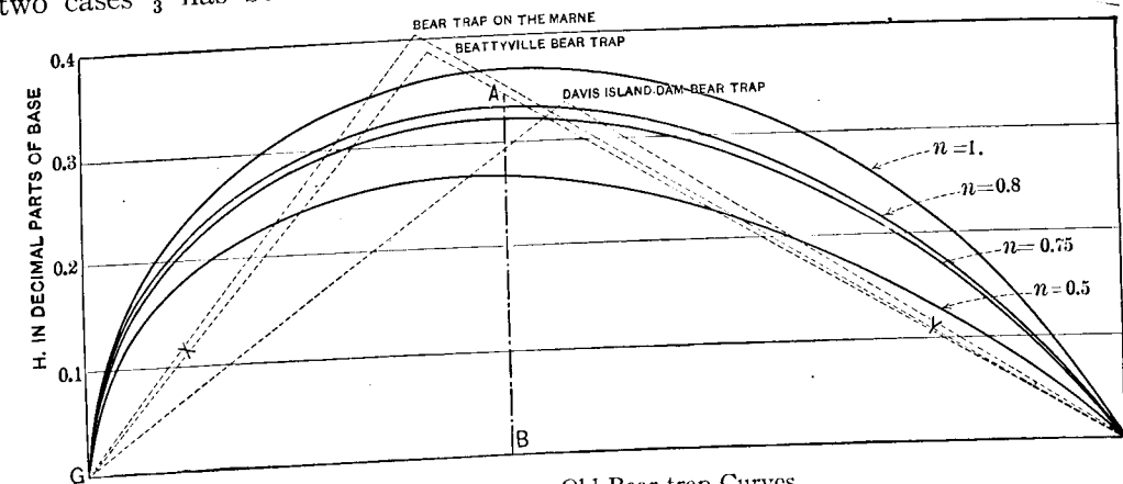
FIG. 241.—Old Bear-trap Curves.
