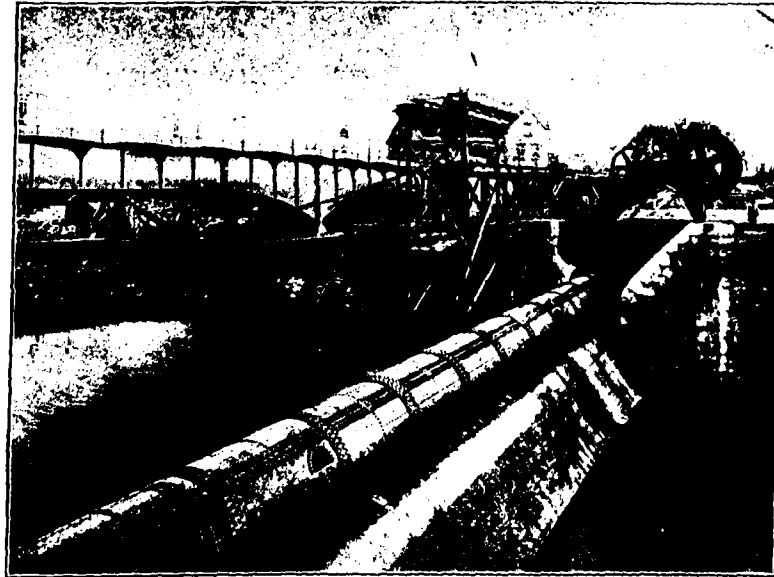
The Larger Schweinfurt Dam, Lowered in Place.
