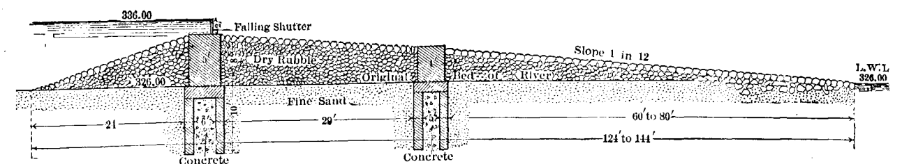
FIG. 201.—Dehri Weir, River Sone (India). Lift, 10.0 feet. Length, 12,500 feet. Flood discharge, 830,000 Second-feet.
