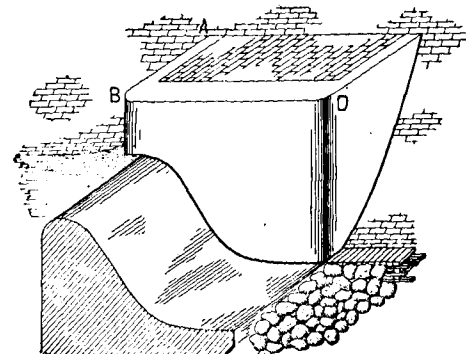
FIG. 204.—U Abutment.
