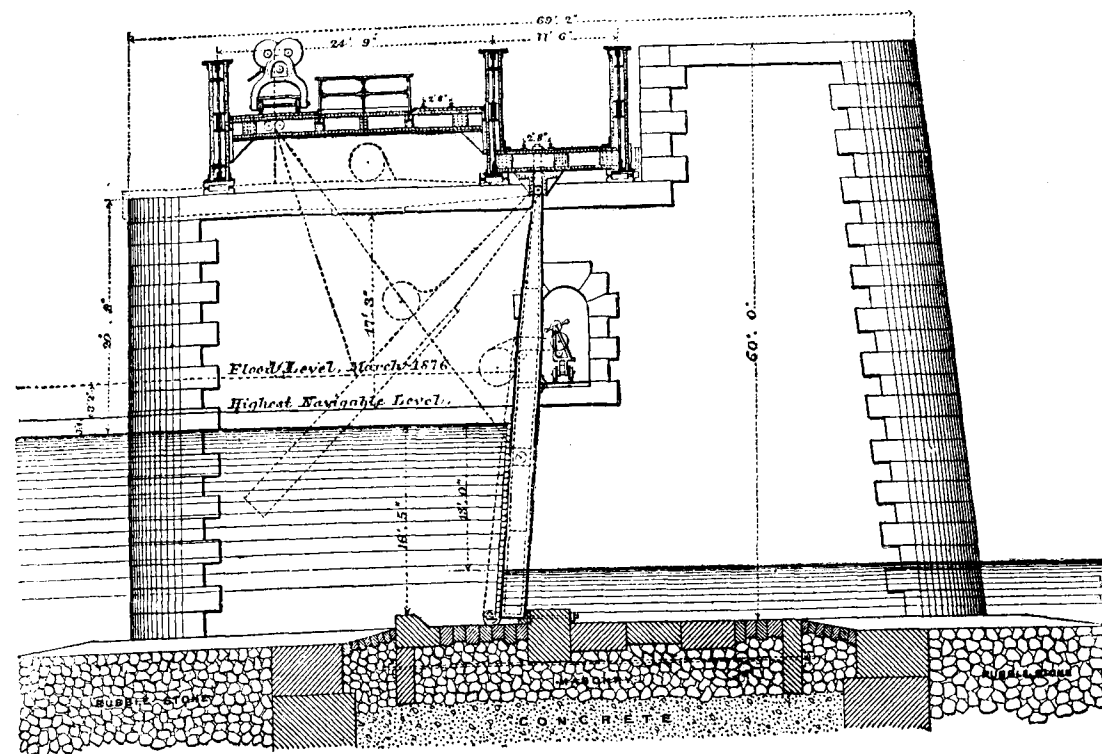
FIG. 224.—General Section of the Poses Dam. (Built on a chalk foundation.)
