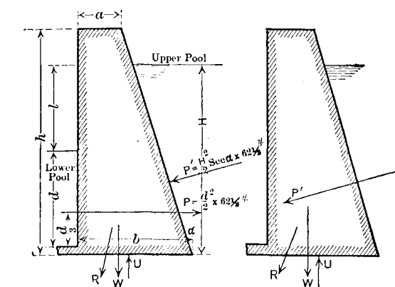
FIG. 148.—Normal Conditions. FIG. 149.—Conditions with Lock Unwatered.
