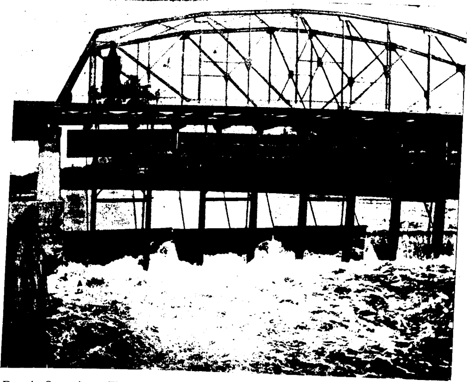
Placing a Dam in Operation. The gates of the lower tier are resting on the masonry sill, with the exception of the three shown, which are about to be lowered the final 2 feet. The upper gates have not yet been lowered.
