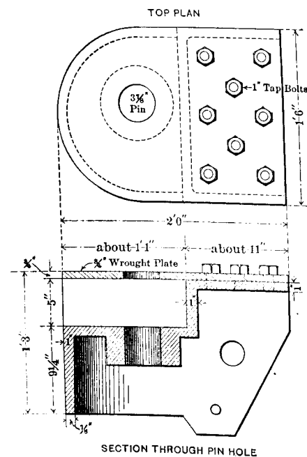
CAST BONNET WITH BOLTED CAP-PLATE.
