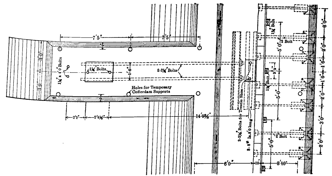
PLAN OF SILL AND TREESTLE ANCHORAGES
