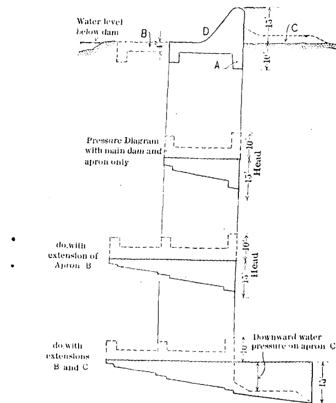
FIG. 140.—The hatched portion below the horizontal line represents the up-pressure on the base of the dam due to the head from the upper pool; the portion enclosed in broken lines represents the up-pressure due to immersion. The total up-pressure is their algebraic sum. The diagrams neglect the weight of the masonry and of the aprons.
