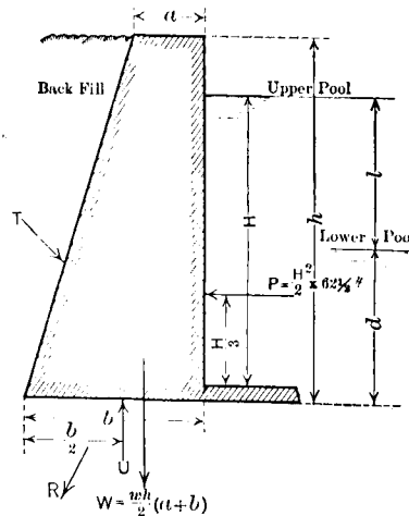
FIG. 150.—Normal Conditions.
