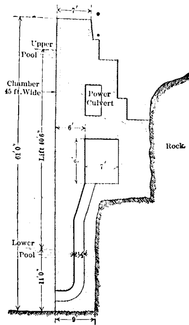
FIG. 160.—Section of North Wall of Lock at Little Falls, N. Y. (Mohawk River, 1911.)
