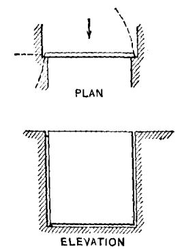
SINGLE SWINGING GATE
