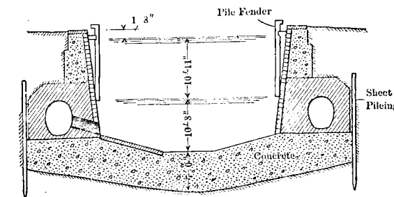
FIG. 162.—Section of Lock Chamber with Battered Masonry Walls and Pile Fenders. (At Teglingen on the Dortmund-Ems Canal. Built about 1896.)
