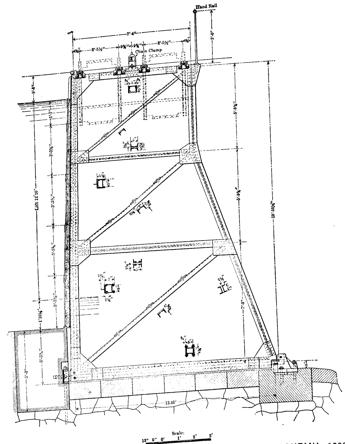
GENERAL SECTION OF THE BOULÉ DAM AT LIBSCHITZ, BOHEMIA, 1900.
