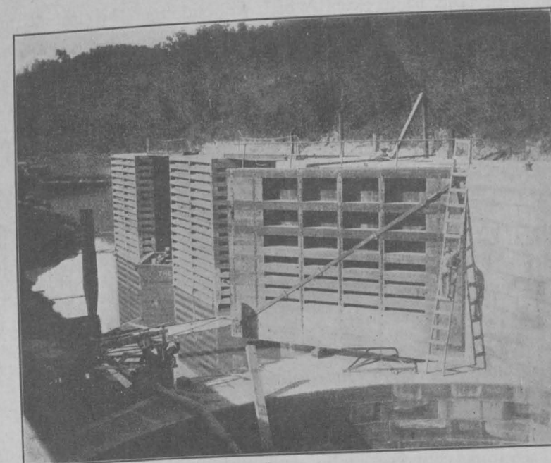
View of an Upper Lock-gate of Timber, with Triangular Guard Cribs.
