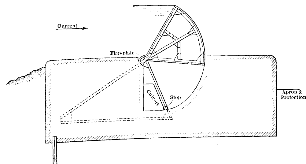
FIG. 232.—Typical Section of a Chittenden Drum Wicket.
