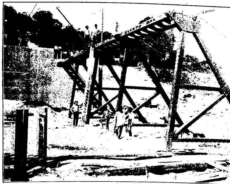
Pass Trestles, Escape-bars and One Needle. Trestles are 20 Feet Centers, and the Needles are 12"×12" and a little more than 18 Feet in Length. (See Pl. 59.)
