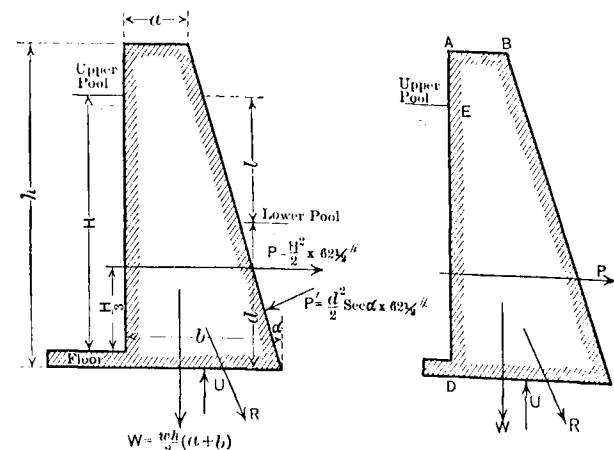
FIG. 146.—Normal Conditions. FIG. 147.—Conditions with Lower Pool drawn off.
