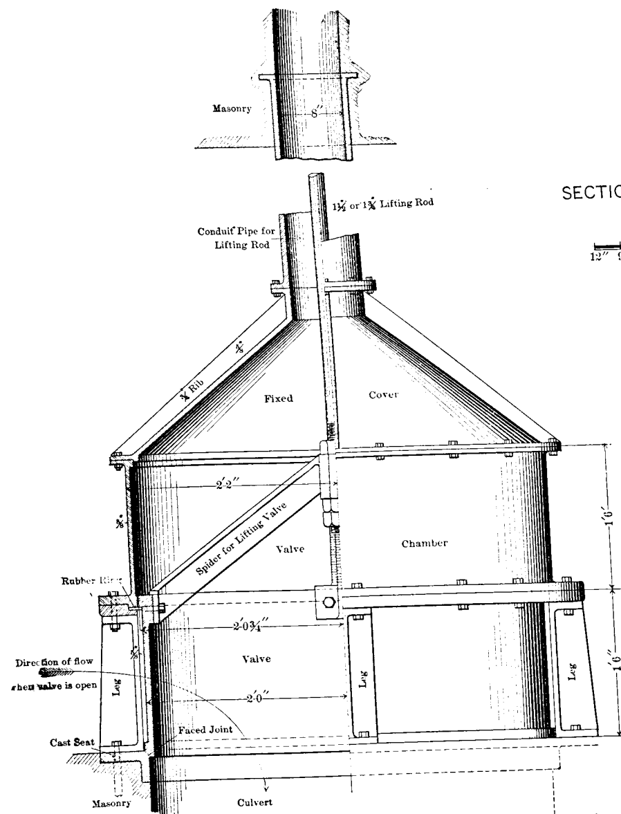
SECTIONAL ELEVATION OF DRUM OR CYLINDRICAL VALVE (FONTAINES VALVE) AS USUALLY MADE, WITH VALVE MOVING IN WATERTIGHT CHAMBER.
