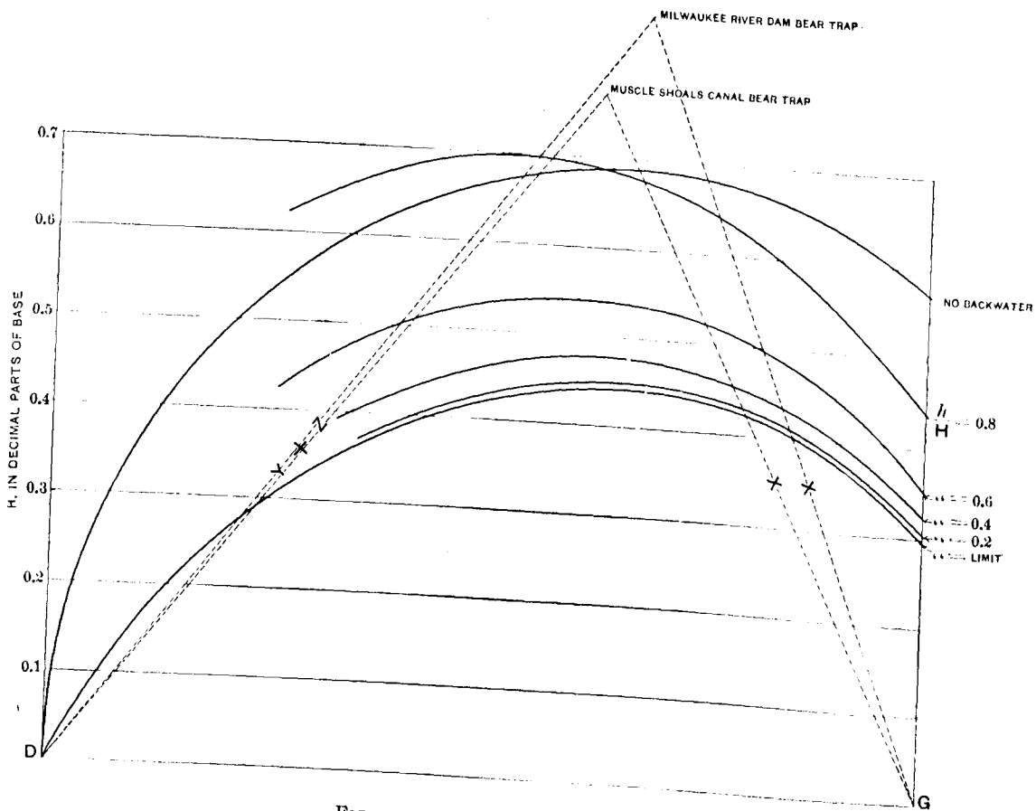
FIG. 243.—Parker Bear-trap Curves.
