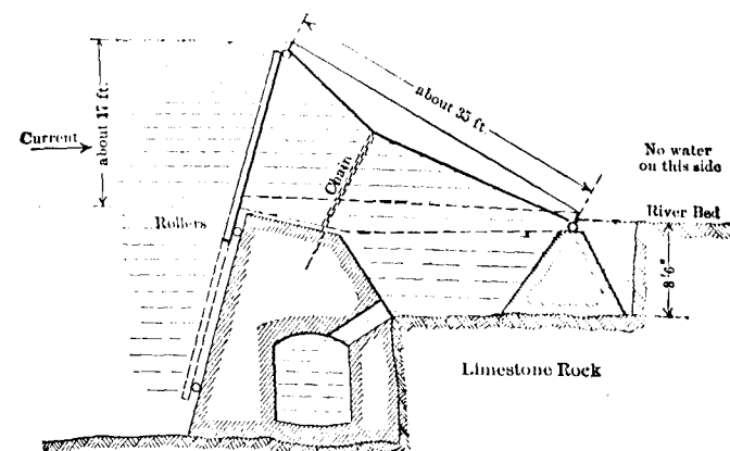
FIG. 238. —Sketch Illustrating the Design of the Chicago Drainage Canal Bear-trap
