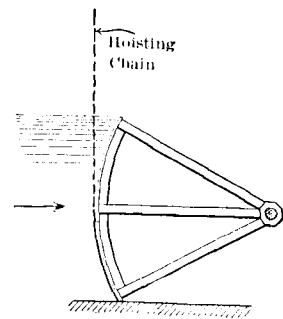
FIG. 202.—Taintor Gate.
