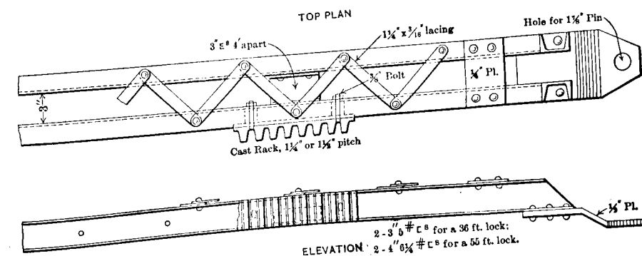
STEEL SPAR FOR OPERATING GATES.
