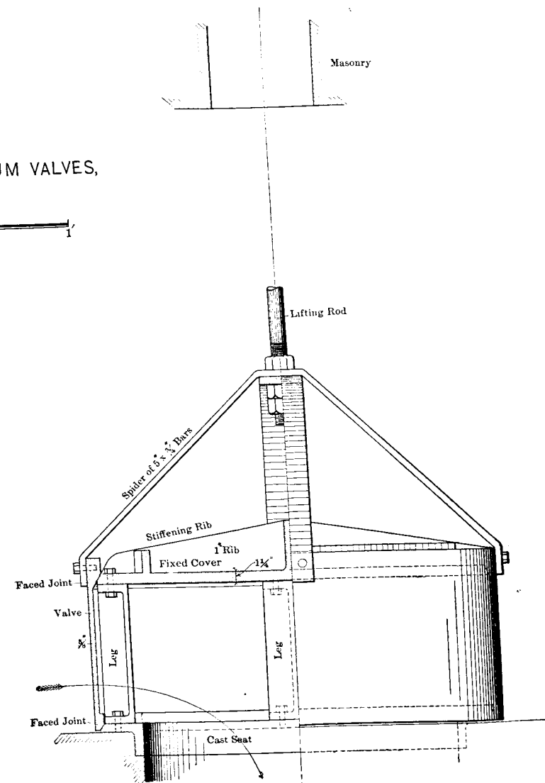
SECTIONAL ELEVATION OF PROPOSED DRUM VALVE WITHOUT WATERTIGHT CHAMBER.
