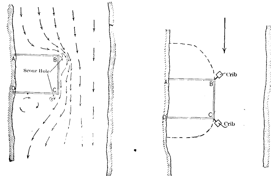
FIG. 129.—Directions of Currents around a Cofferdam.
