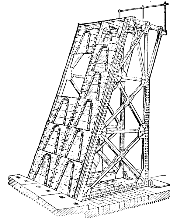
FIG. 218.—Perspective View of Boulé Gates and Trestles, as Used at the Suresnes Dam.
