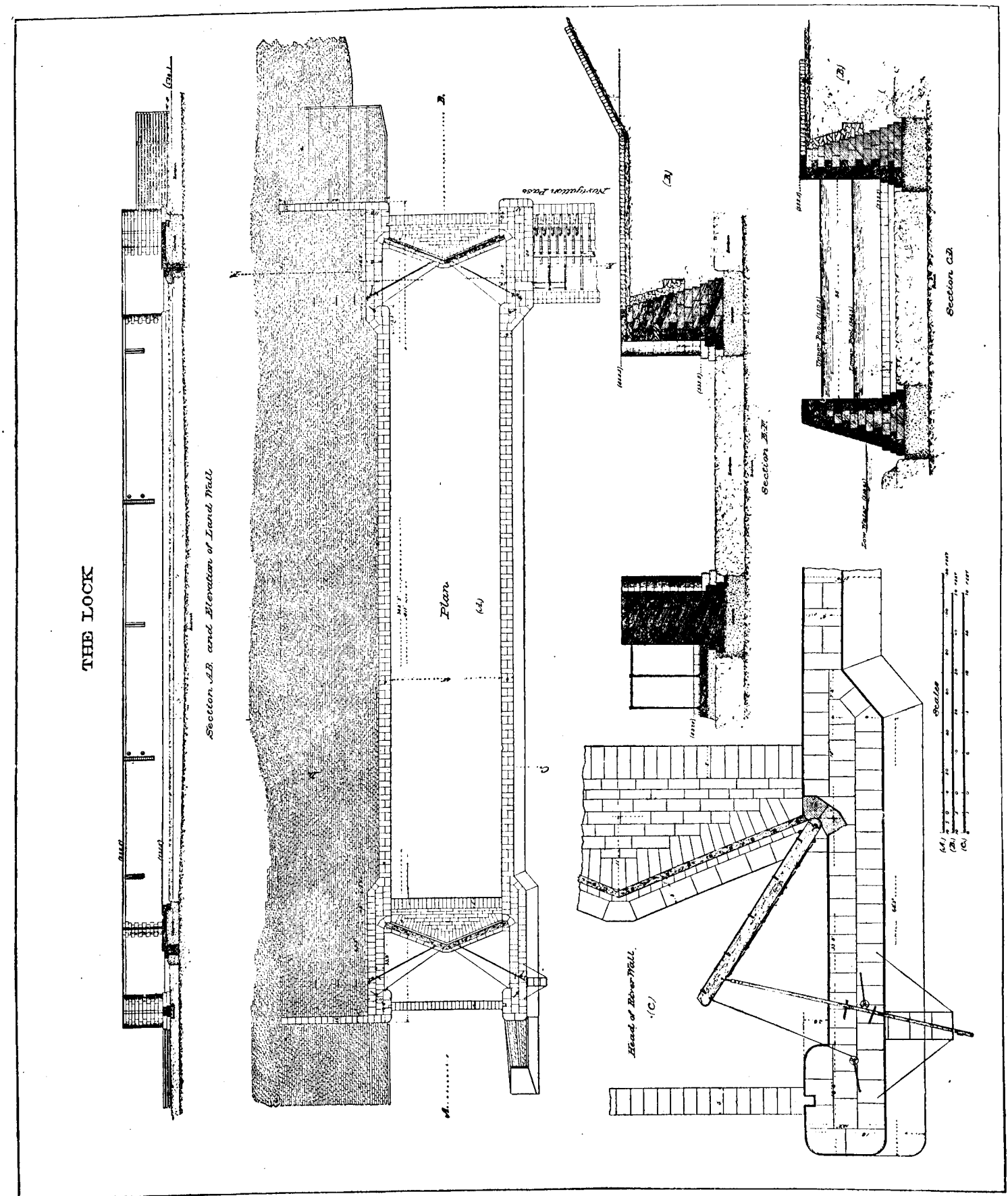
GENERAL PLAN, ETC., OF LOCK NO. 7, KANAWHA RIVER, W. VA. (Built on rock.)
