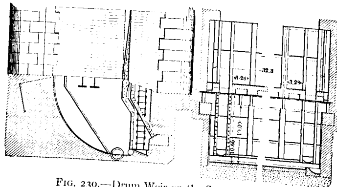
FIG. 230.—Drum Weir on the Spree, Germany.
