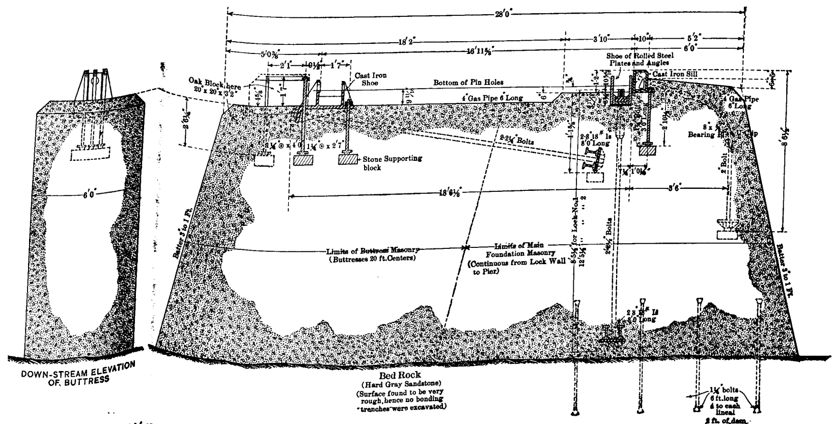
DAM NO. 1, BIG SANDY RIVER, W. VA. AND KY. DETAILS OF FOUNDATIONS AND SUPERSTRUCTURE.
