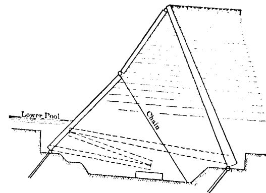
FIG. 235.—Section of a Reversed Parker Bear-trap Dam.
