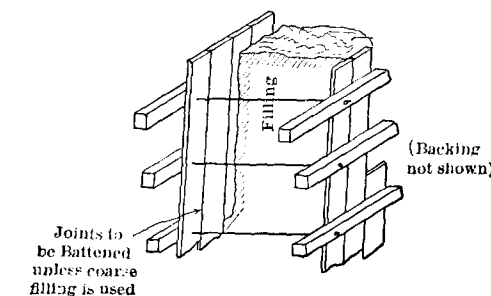
FIG. 135.—Box Cofferdam.
