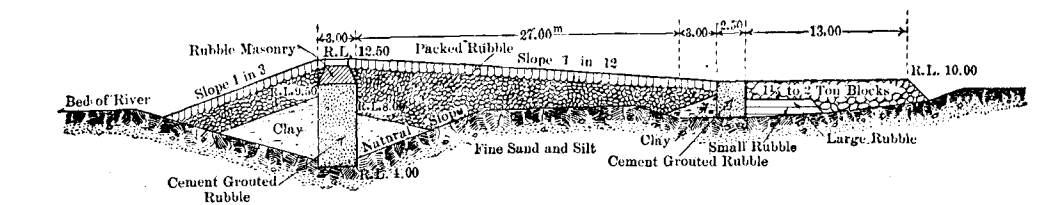
FIG. 200.—Rosetta Weir, River Nile, 500 Meters Long. (1901.)
