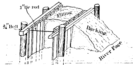
FIG. 133.—Pile Cofferdam, Double Row.
