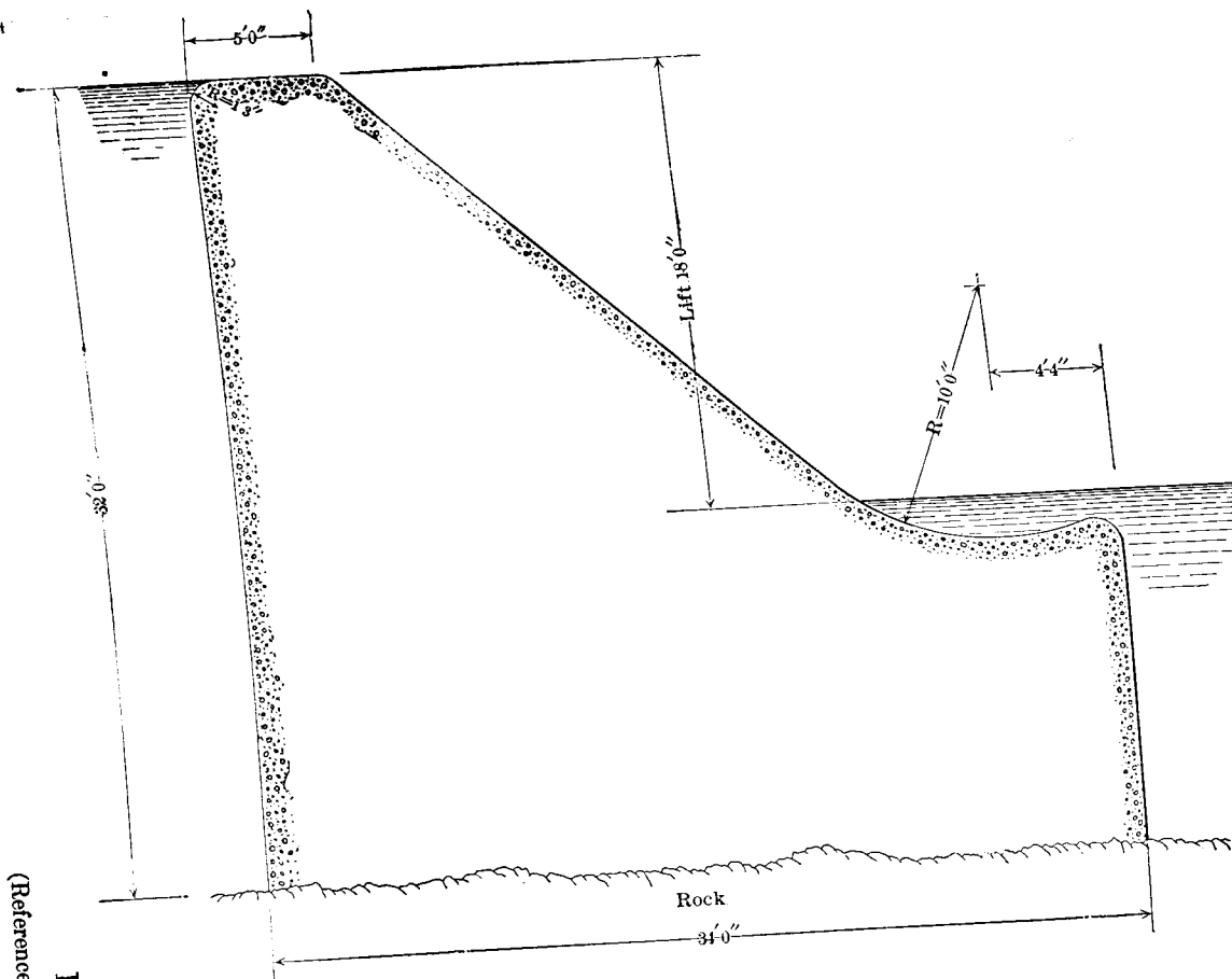
CONCRETE DAM. No. 9, Kentucky River, Ky. 1902 Length 250 ft. Proportions about 1 of Portland Cement to 12 of sand and limestone. Facing 1 to 2, 1½ inches thick.
