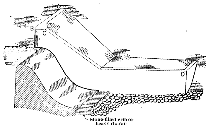
FIG. 205.—L Abutment.
