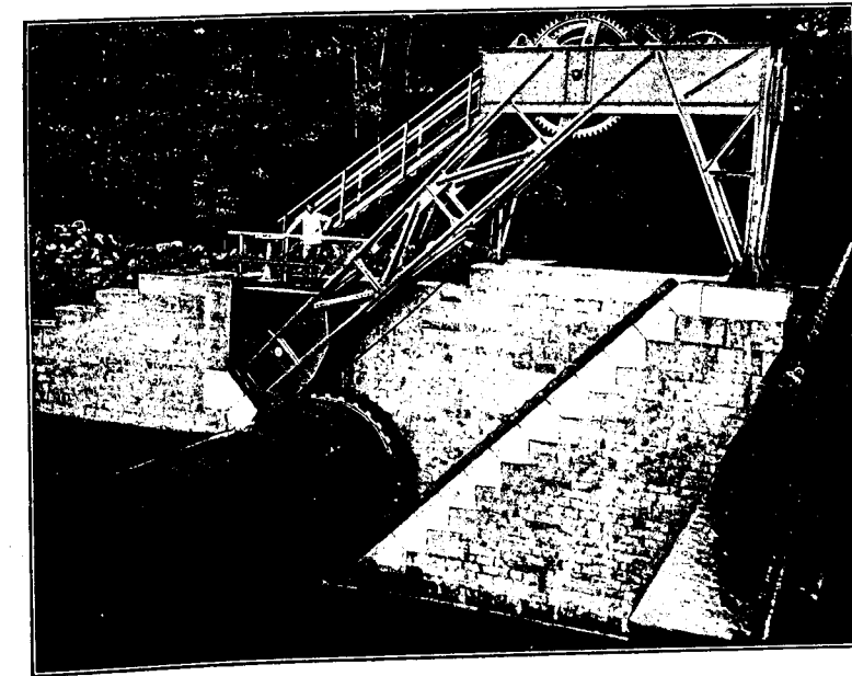
Rolling Dam at Schweinfurt, Showing Rack and Operating Machinery.
