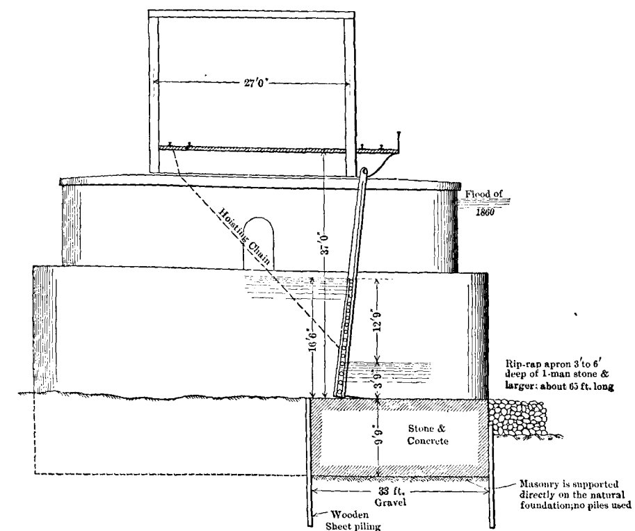
FIG. 225.—Section of the Pass of the Mirowitz Bridge Dam, Moldau River, Bohemia.
