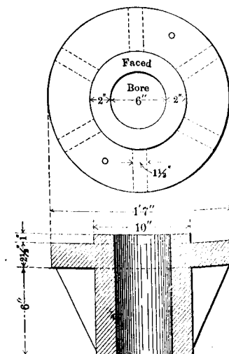
PINTLE WITH STEEL PIN AND CAST IRON SOCKET.
