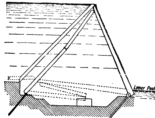
FIG. 234.—Section of Direct Parker Bear-trap Dam with Idler Leaf.
