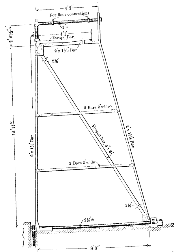
PASS TRESTLE OF THE KLECAN NEEDLE DAM ON THE RIVER MOLDAU, BOHEMIA, 1899. (Trestles are spaced 1\frac{1}{4} meters apart.)
