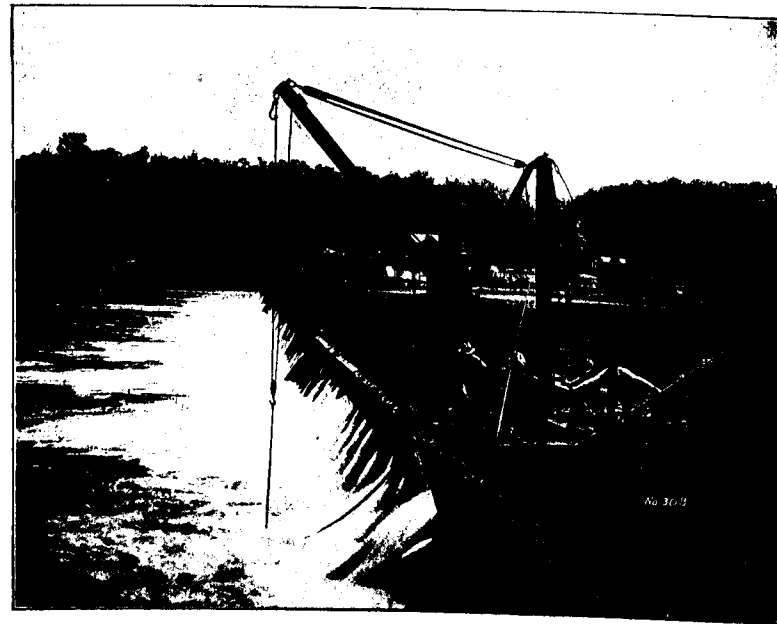
Maneuvering Boat at Dam No. 2, Ohio River, raising a fallen wicket. (The dam has just been raised and the pool is filling.)
