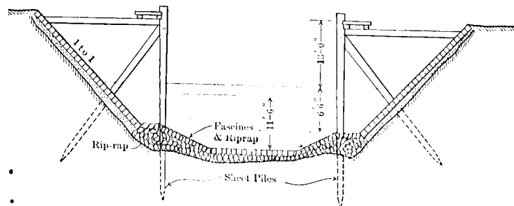
FIG. 163.—Section of a Lock Chamber with Paved Earth Slopes and Pile Fenders. (At Bollingerfähr, on the Dortmund-Ems Canal.)
