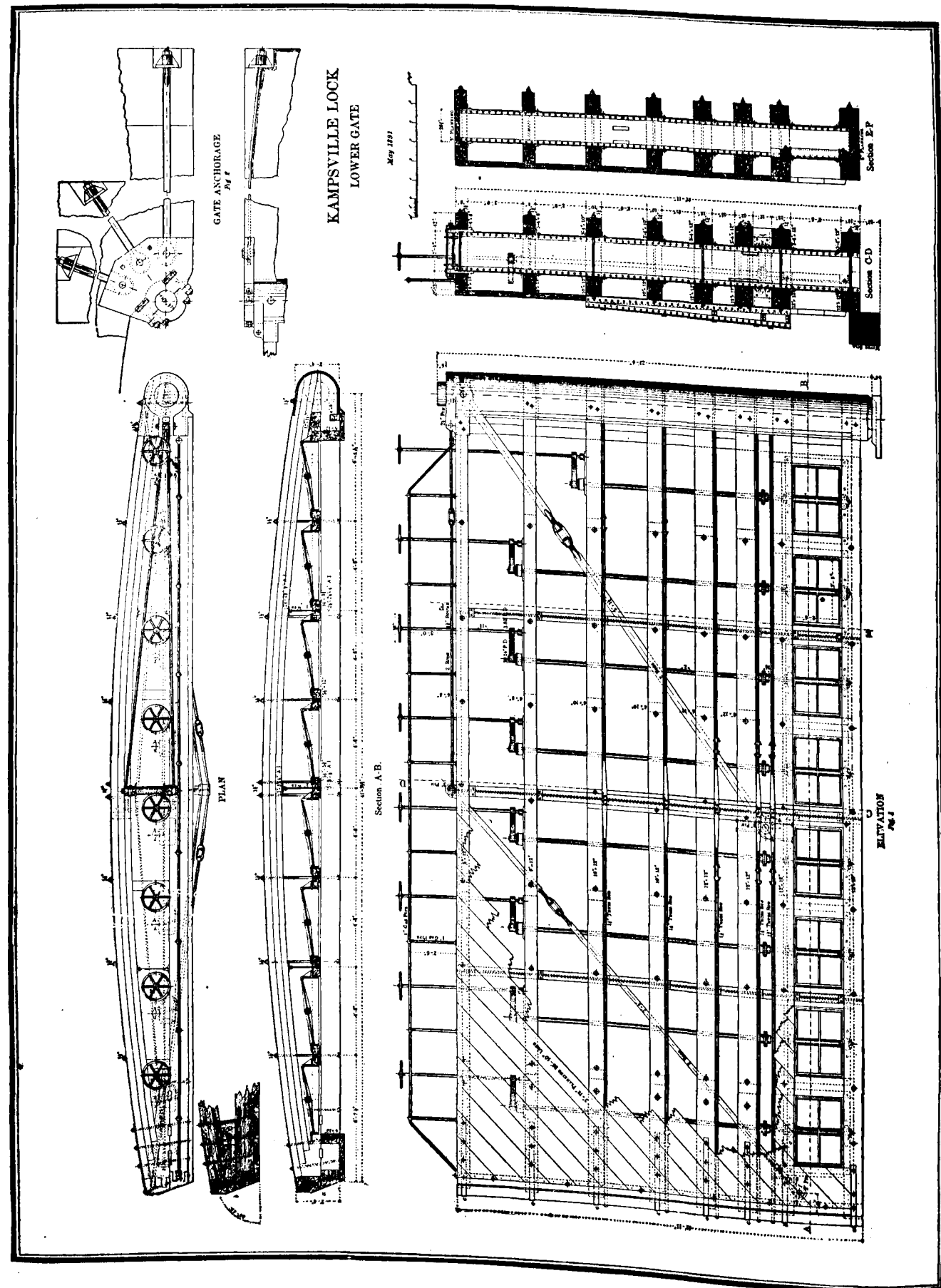
GATE OF THE KAMPSVILLE LOCK, ILLINOIS RIVER, ILLINOIS. (Trussed Bowstring Type.)
