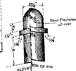
PINTLE WITH STEEL PIN AND CAST IRON SOCKET.
