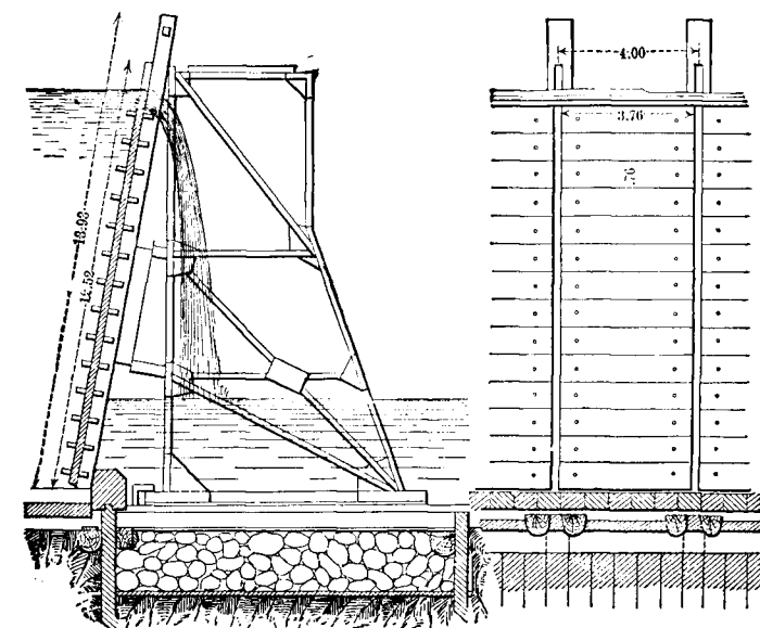
Dam Composed of Needles and Boulé Gates, on the River Moskva, Russia.
