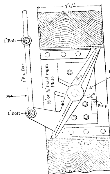
SECTION OF WOODEN GATE, SHOWING VALVE AND GIRDER IN PLACE.
