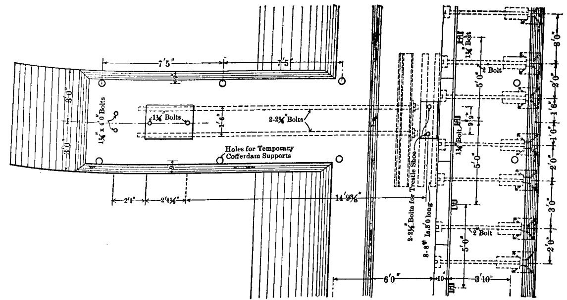
PLAN OF SILL AND TRESTLE ANGHORAGES
