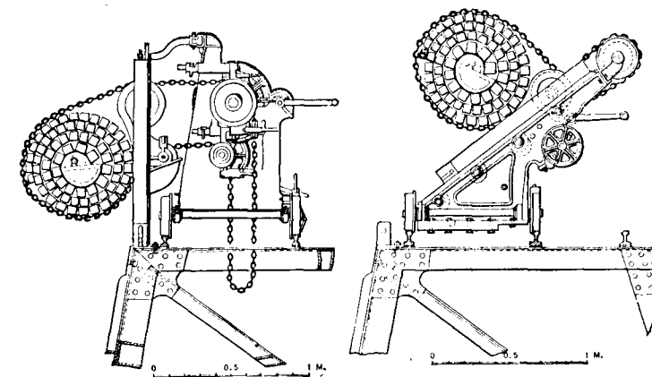
FIG. 221.—Method of Handling Curtains with a Service Truck and Crab.
