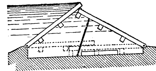
FIG. 233.—Section of Old Bear-trap Dam.
