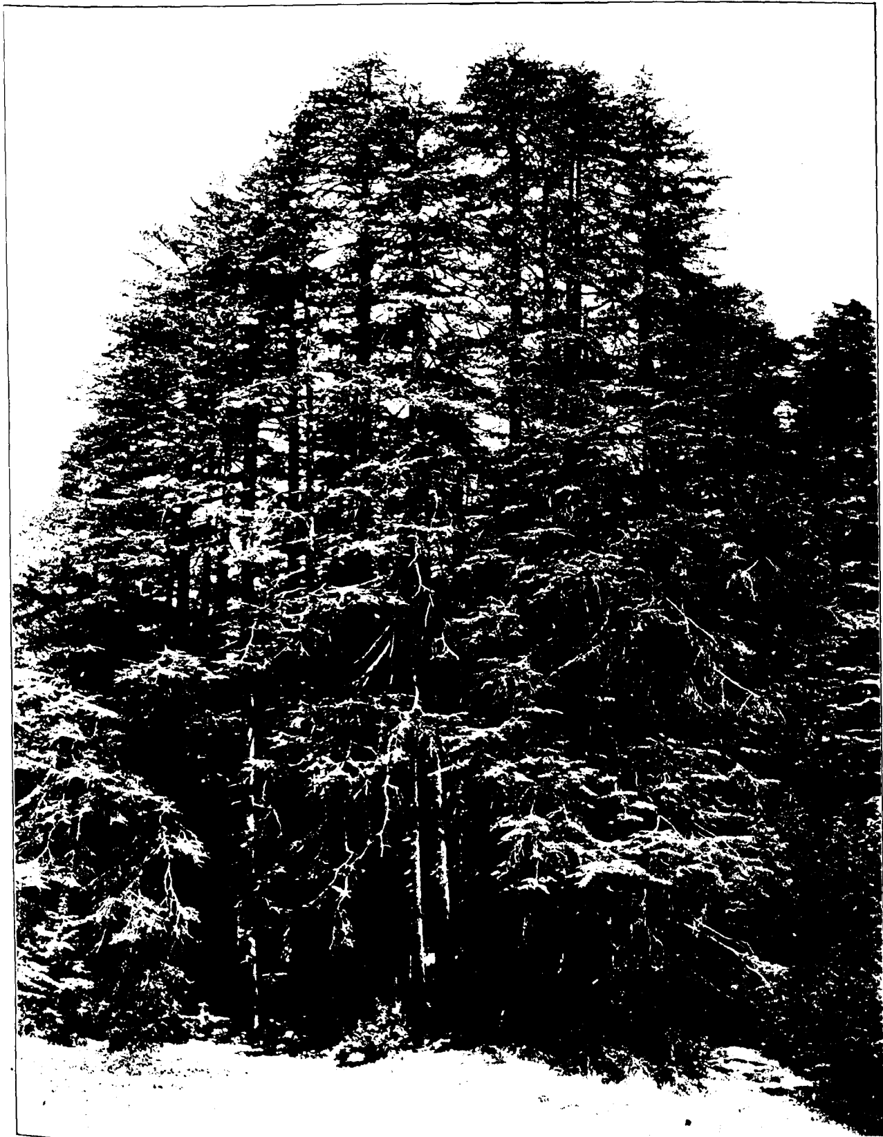
A Group of Deodar trees. Girth 10 ft., height 150 ft., Jaunsar Division, U. P.
