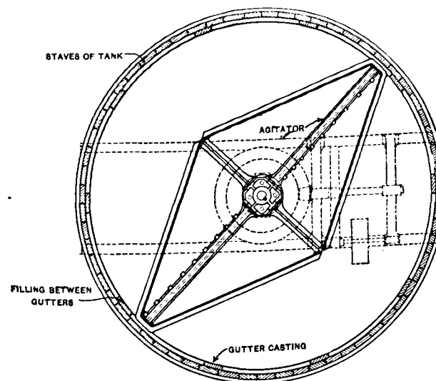
PLAN OF AGITATOR, GUTTER CASTINGS, ETC.
