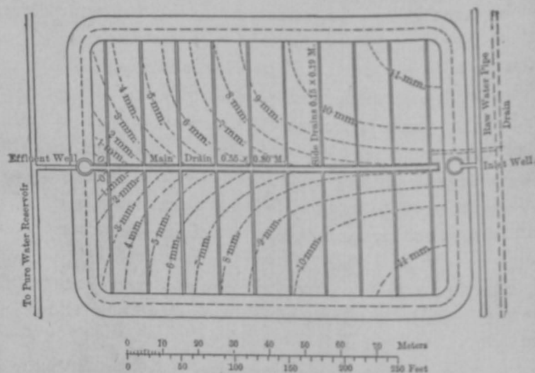
FIG. 4.—PLAN OF ONE OF THE HAMBURG FILTERS, SHOWING FRICTIONAL RESISTANCE OF THE UNDERDRAINS.
