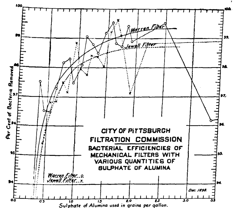
FIG. 21.—BACTERIAL EFFICIENCIES OF MECHANICAL FILTERS.
