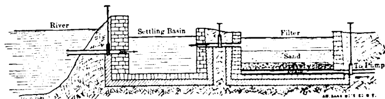
FIG. 1.—SKETCH SHOWING GENERAL ARRANGEMENT OF FILTER PLANTS.
