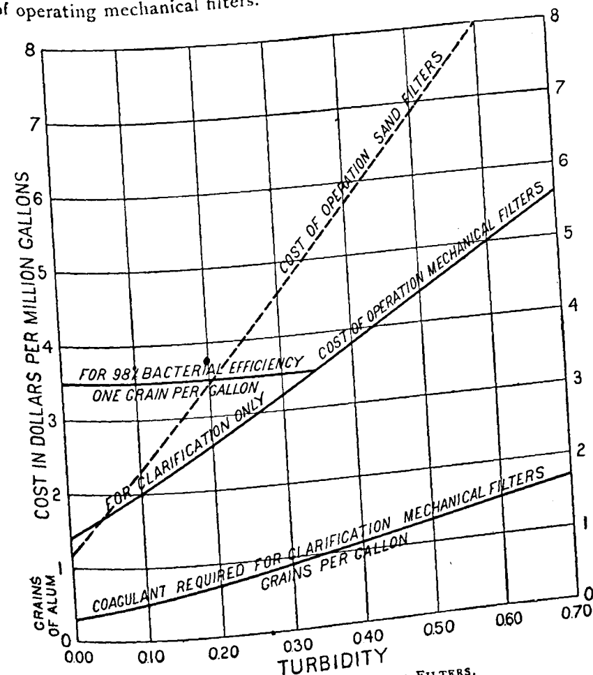
FIG. 26.—COST OF OPERATION OF FILTERS.
