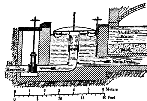
FIG. 9.—LINDLEY'S REGULATION APPARATUS AT WARSAW, RUSSIA.
