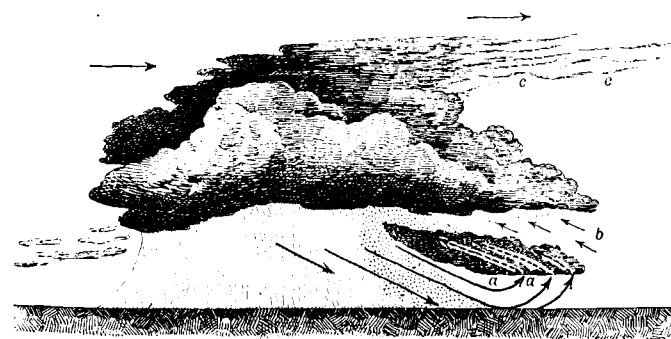
FIG. 7.—SECTIONAL DIAGRAM OF A SQUALL. AFTER MÖLLER.
