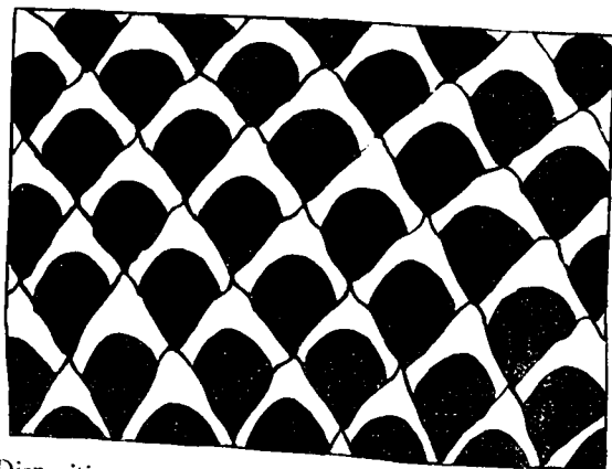
FIG. 3.—Disposition of equatorial chambers and canals in Orbitoides cf. minor .
