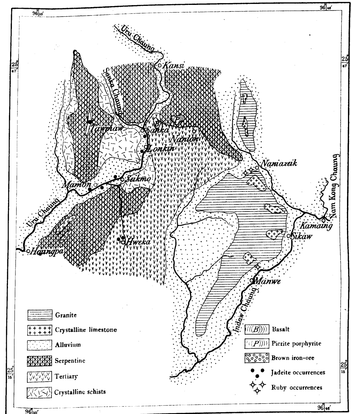
JADEITE IN UPPER BURMA.
