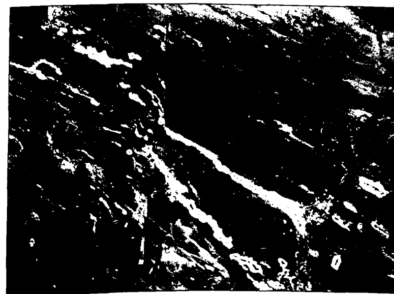
EFFLORESCENCE OF ALUM AT MORMUGAO.
