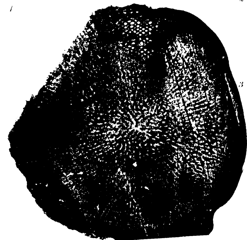
Orbitoides media d'Archiac 1, megaspheric; 2, microspheric 3, lateral layers.
