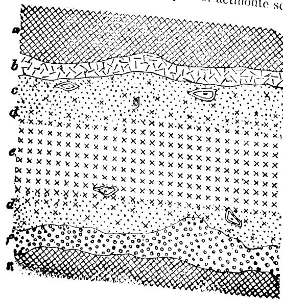
Fig. 3. Section through the jadeite-albite dyke at Tawmaw. a. Serpentine. b. Earthy chlorite. c. Albite rock with inclusions of schistose amphibolite. d. Zone of mixed albite and jadeite. e. Jadeite. f. Amphibolite.
