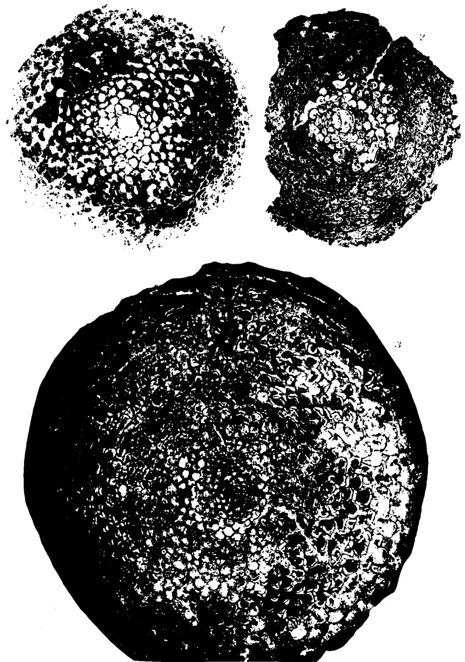
Omphalocyclus macrostoma , Lamarck. 1, 2, megaspheric. 3, microspheric.
