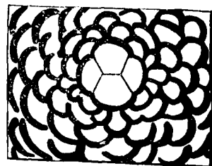
FIG. 5.—Innermost chambers of a megaspheric individual of Omphalocyclus macropora from the Maestrichtian of Maestricht, magnified 22 times, after A. Silvestri.
