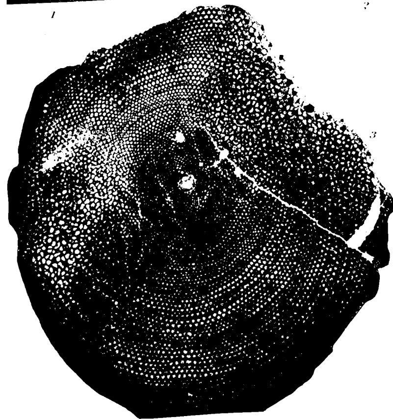
Orbitoides socialis . Leymerie. 1. lat. rat. layers. 2. Equatorial layer. 3. Specimen from the Pyrenees.
