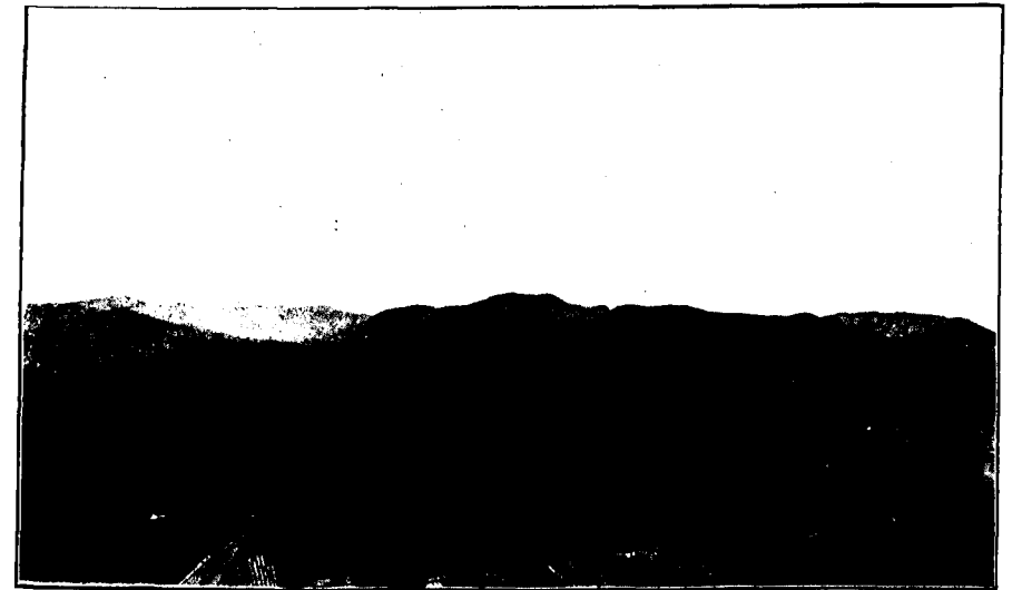
FIG. 2. THE LESSER HIMALAYA, AS SEEN FROM SIMLA,
