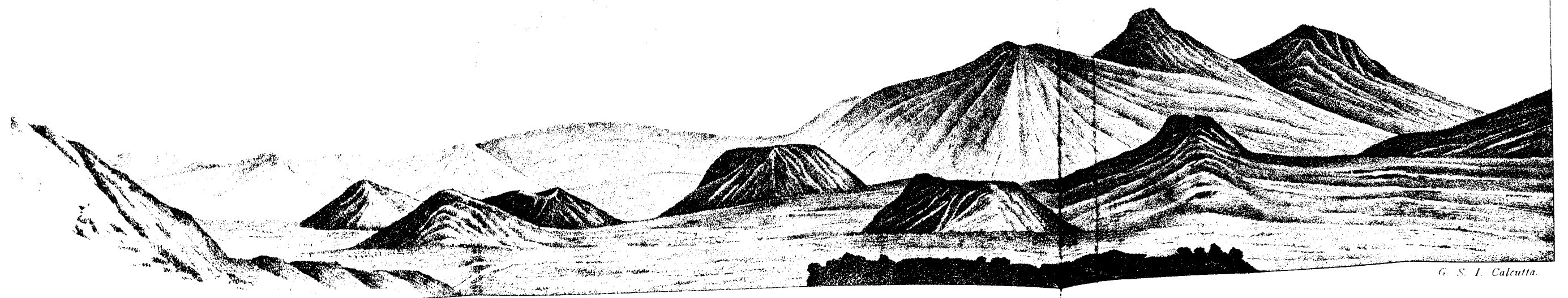
THE KUNG-PO GROUP OF GRATERLETS LOOKING SOUTH FROM YAO-WU-SHAN.
