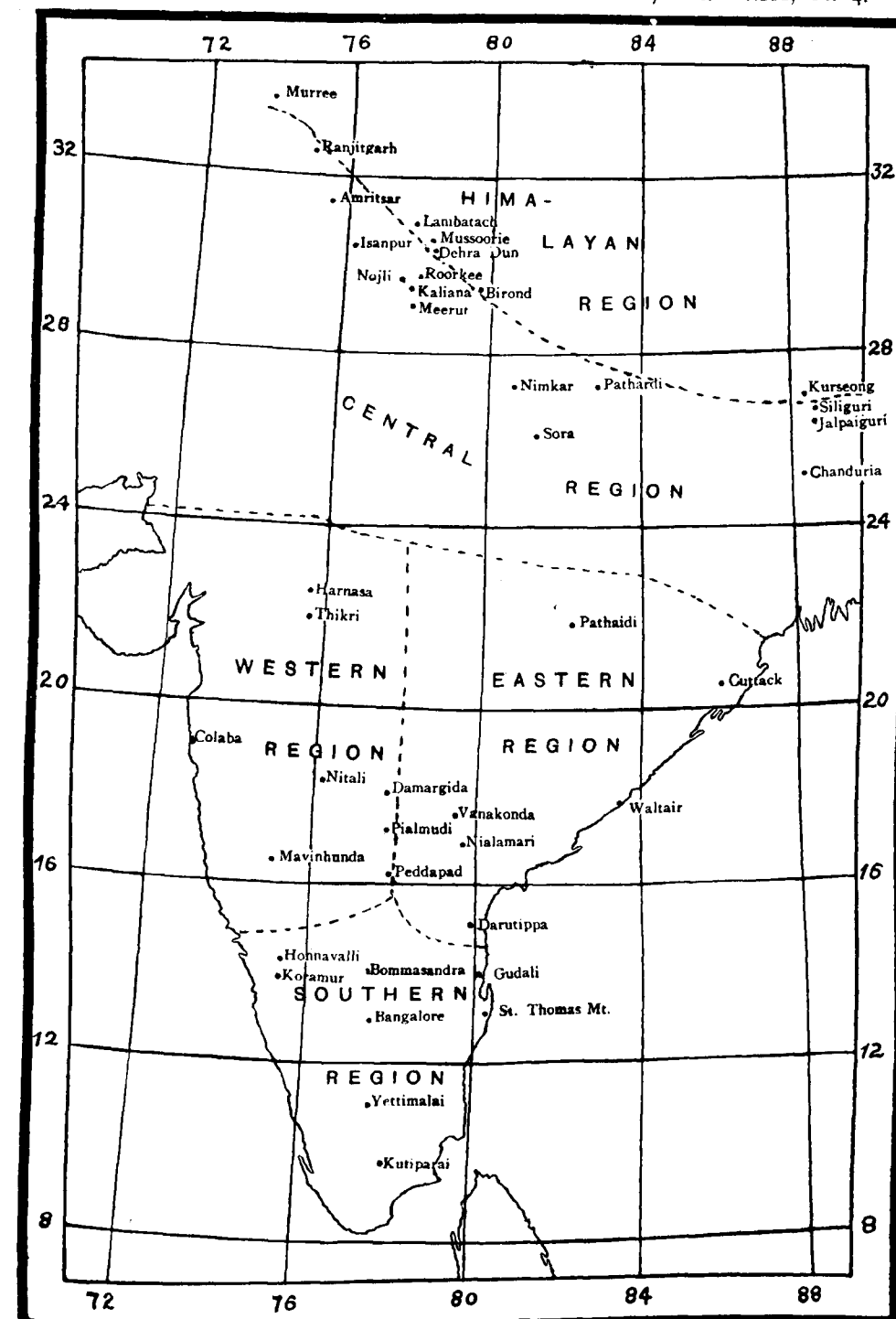
INDEX MAP SHOWING REGIONS AND PLUMB-LINE STATIONS INCLUDED IN TABLES 1-6.
