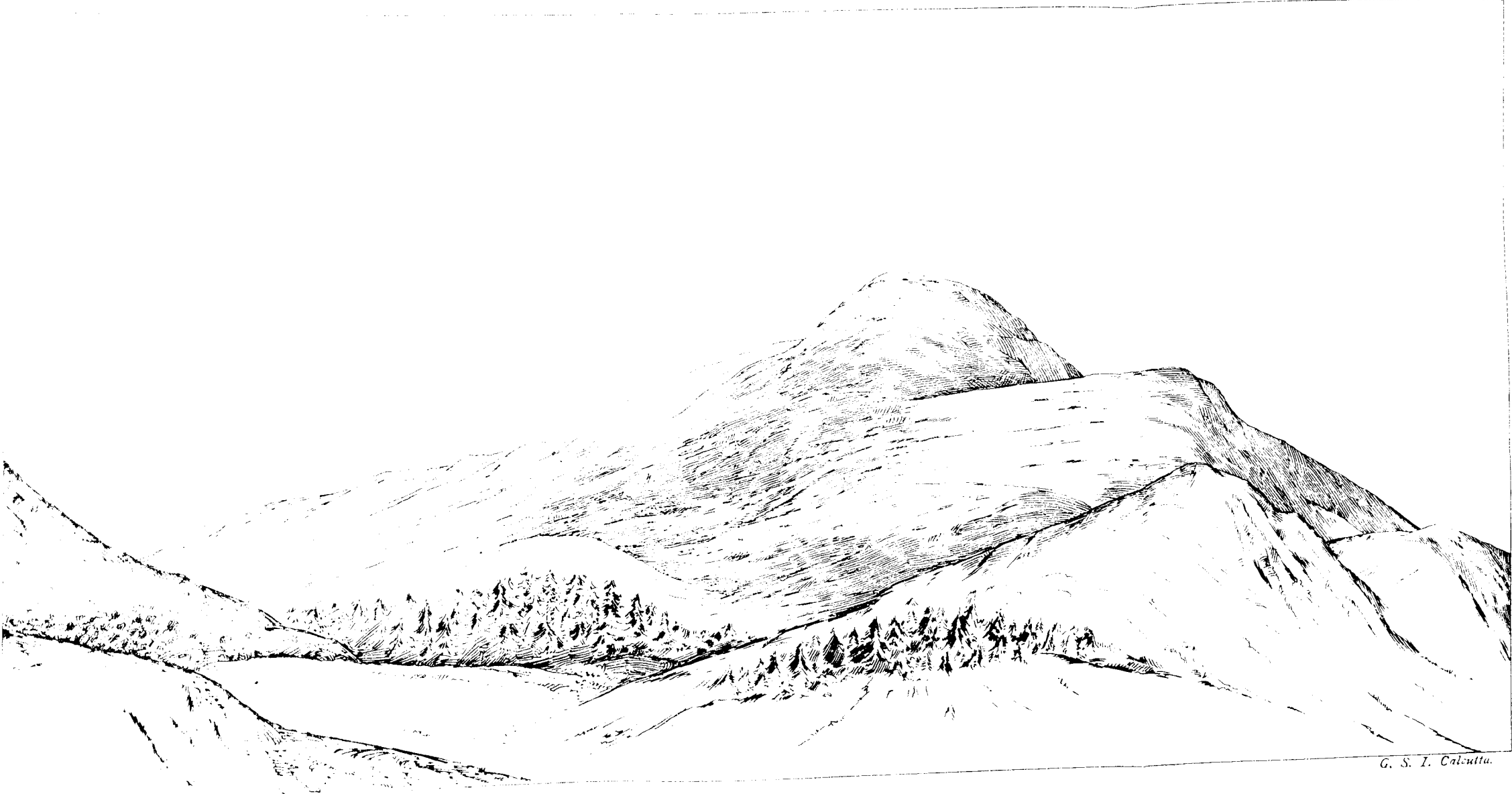
TAY-IN-SHAN. From the North.
