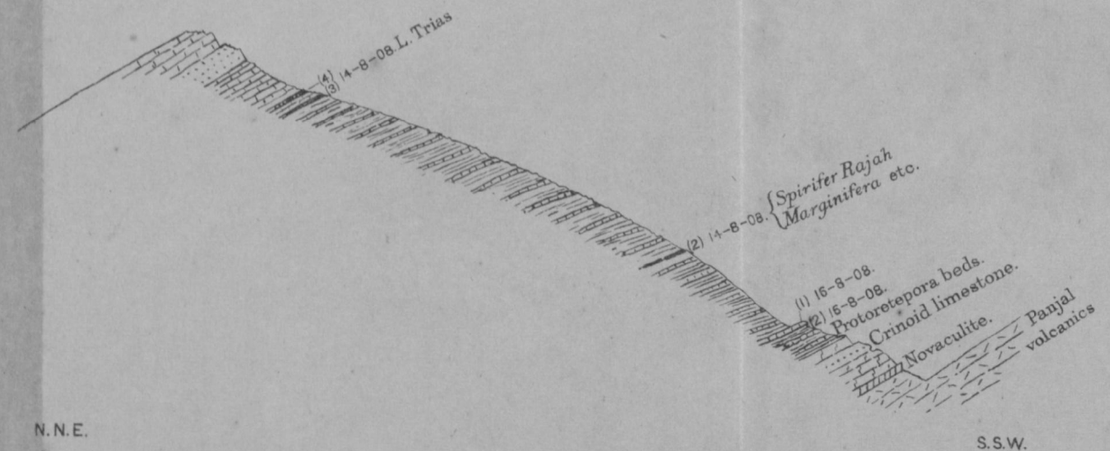
FIG. 2. SECTION OF ABOVE.
