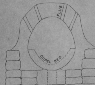
c. Section
