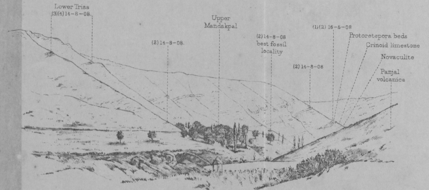
FIG. 1. OUTCROPS NEAR UPPER MANDAKPAL, LOOKING E.
