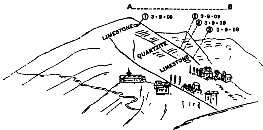
FIG. 4.—Profile view of Eishmakam Hill.
