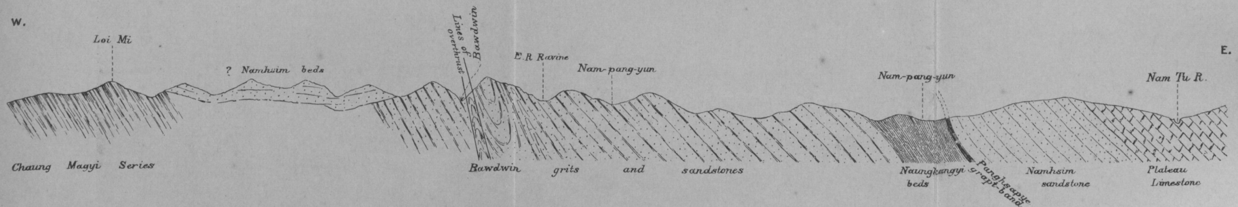
FIG.-2. SECTION THROUGH BAWDWIN Scale, 1 inch = 1 mile
