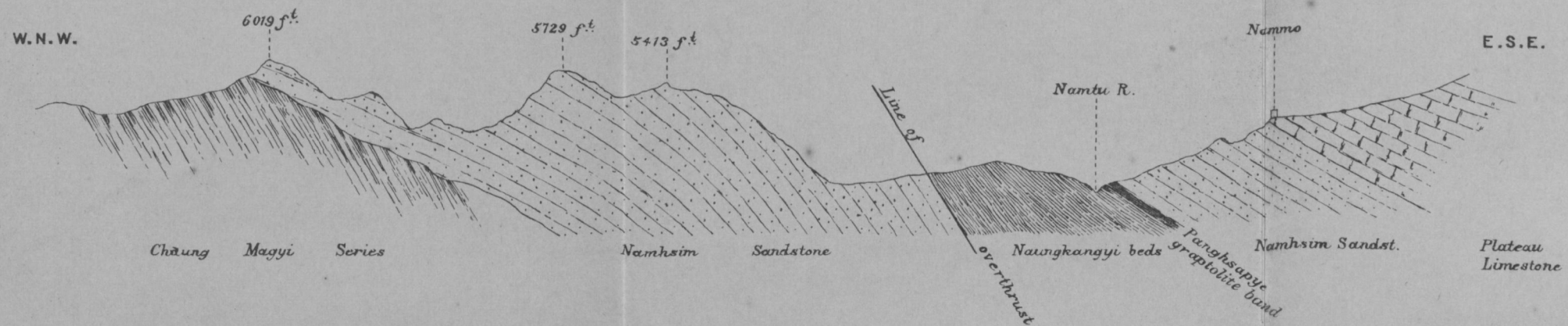
FIG.-1. SECTION ACROSS THE NAM TU VALLEY, NEAR LILU Scale, 1 inch = 1 mile
