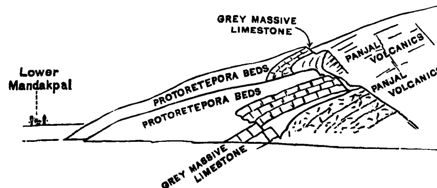
FIG. 2.—Spur S.W. of Lower Mandakpal.
