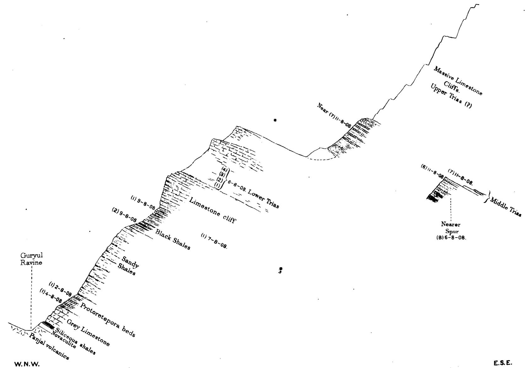
SECTION, GURYUL RAVINE AND E. OF 'IT.
