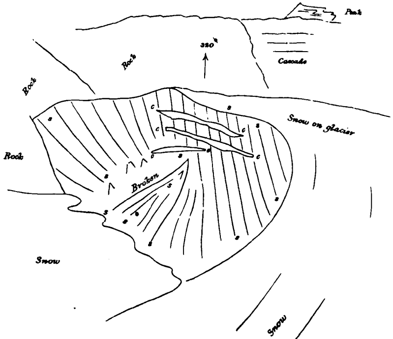
Fig. 16.— STRUCTURE ILLUSTRATING FORMATION OF AN AUXILIARY "ICE-CLIFF." O.O. crevasses. S.S. structure.
