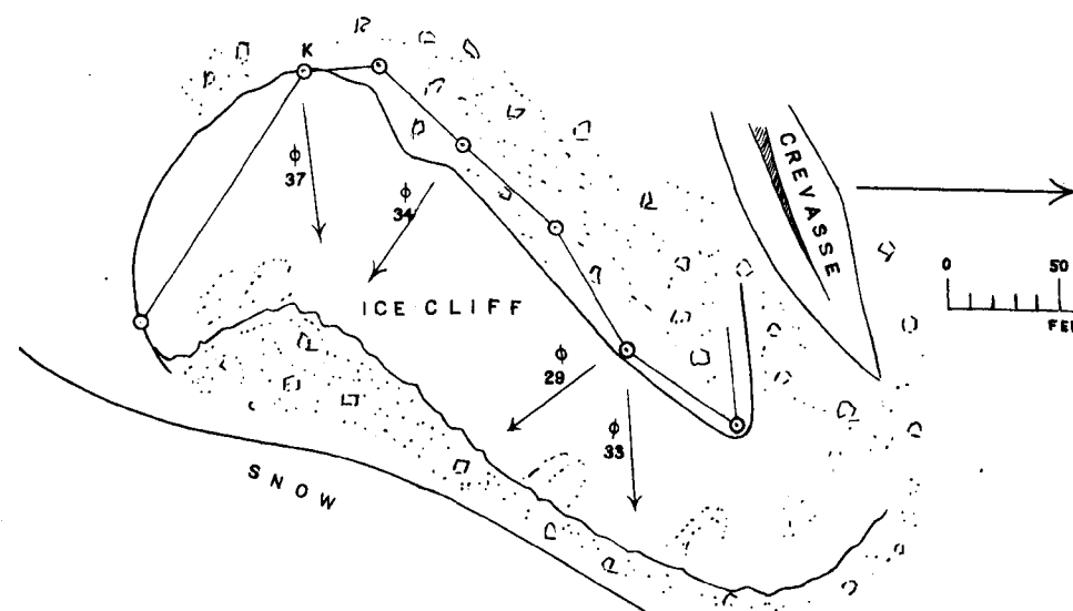
Fig. 5.— SHAPE OF ICE-CLIFF, JUNE 1911. K is the "Cairn"
