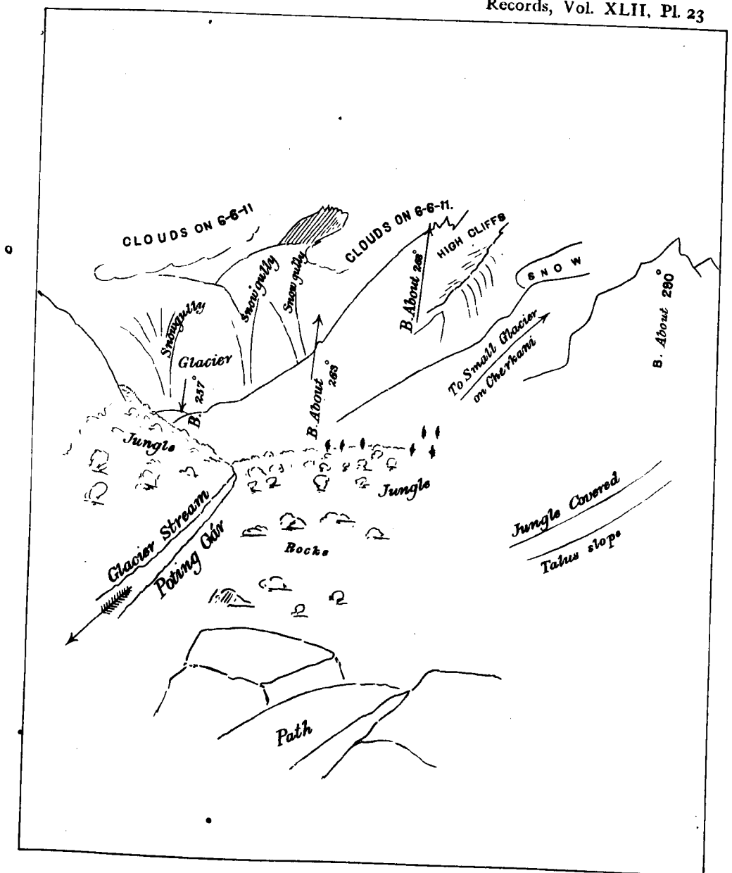
Fig. 11.— SKETCH SHOWING BEARINGS OF CERTAIN PROMINENT FEATURES FROM POINT WHERE THE VALLEY COMMENCES TO OPEN OUT. at 2nd. mile from Bugdhar.
