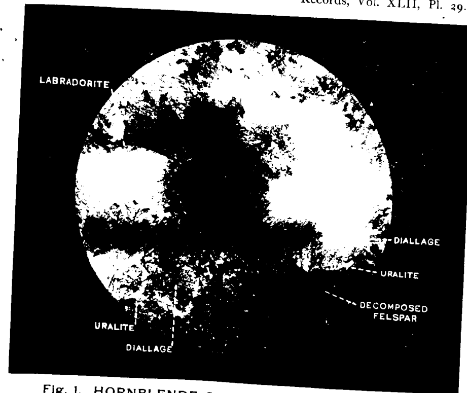
Fig. 1. HORNBLENDE-GABBRO. ( \times 12 diam. cross nicols).
