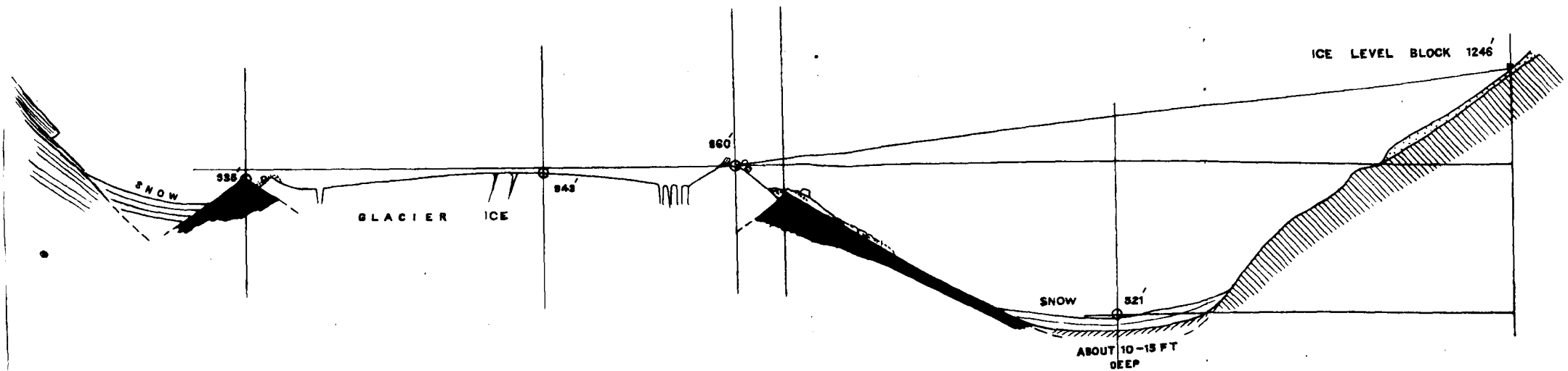
Fig. 6.—SECTION ACROSS THE POTING GLACIER, 7th. June 1911.
