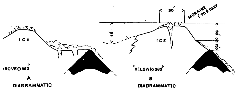
Fig. 3.— TYPE CROSS SECTIONS RIDGE OF LEFT LATERAL MORaine. Above and below 980'
