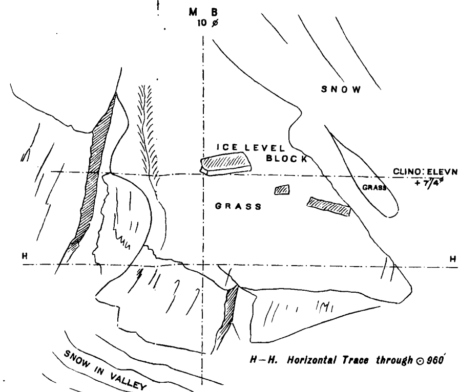
Fig. 4.— ROUGH SKETCH SHOWING ICE LEVEL BLOCK as seen from Point 980, 8th. June 1911.
