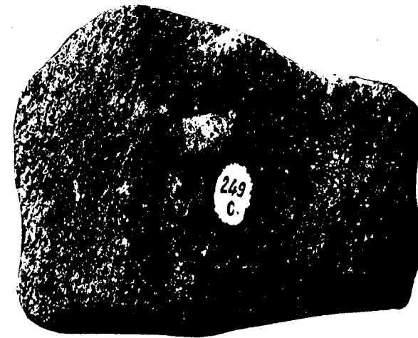
CHAINPUR METEORITE SHOWING GRANULAR STRUCTURE.
