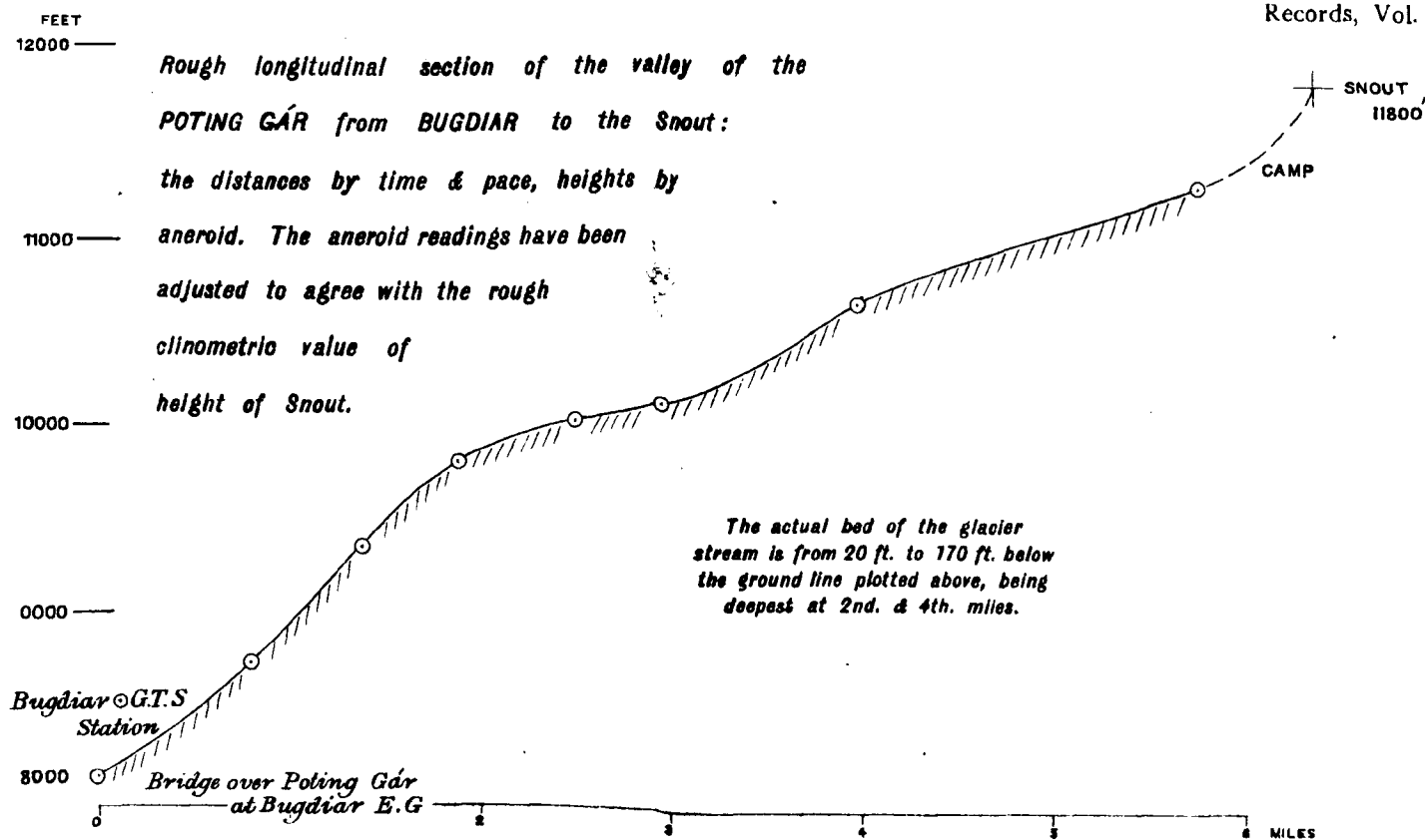
Fig. 8.—ROUGH LONGITUDINAL SECTION FROM BUGDIAR TO THE GLACIER SNOUT.
