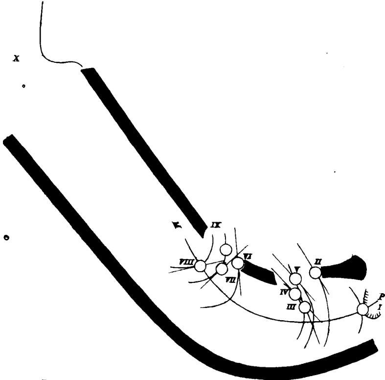
Fig. 12.— RETARDATION OF THE ICE IN LEFT LATERAL MORaine.
