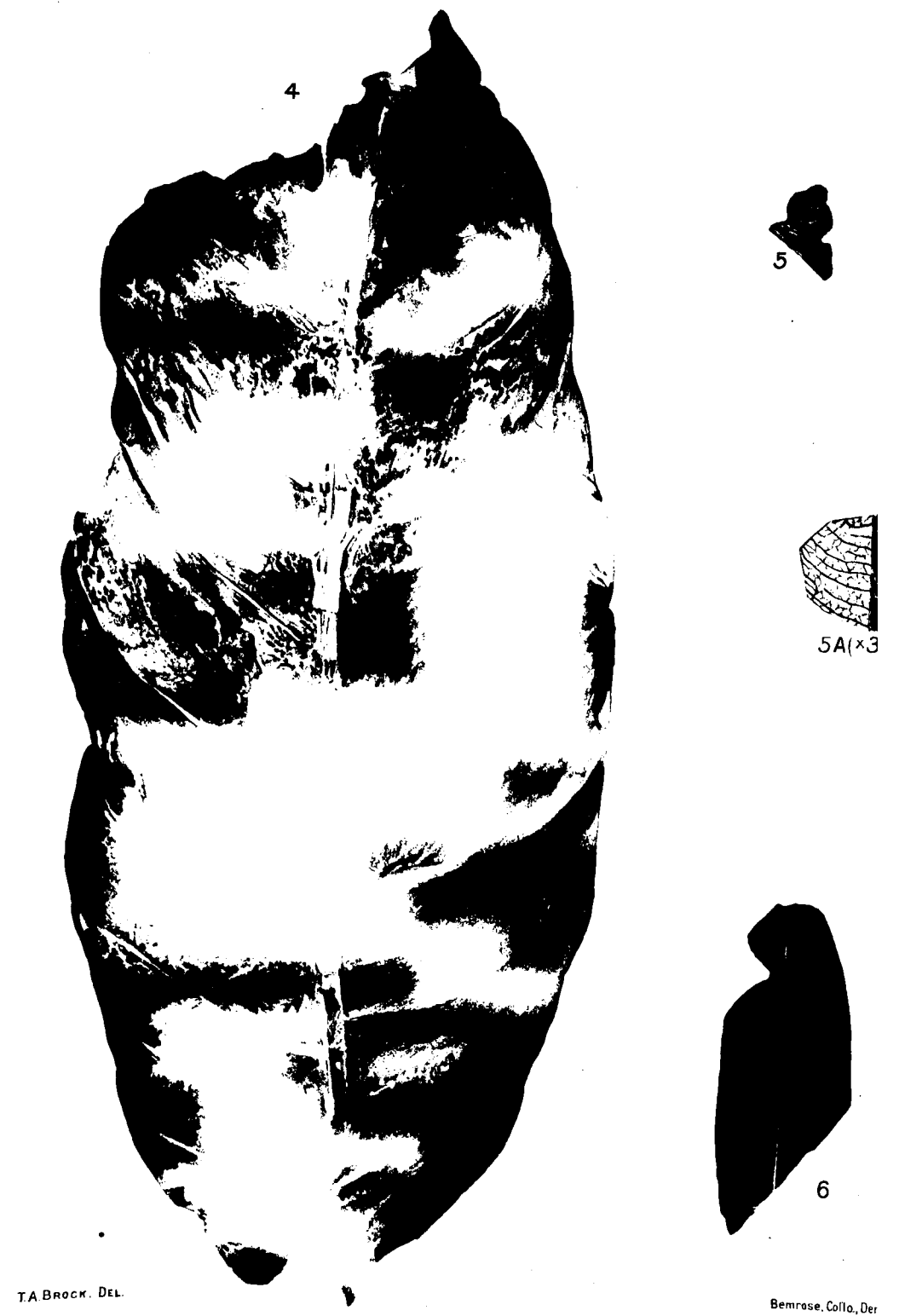
Phyllites kamarupensis , sp. nov. Fig. 4.
