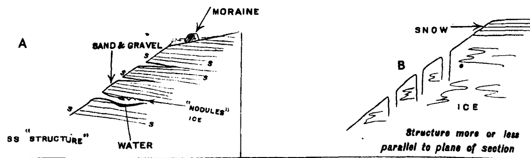
Fig. 9.—TYPES OF CREVASSING.
