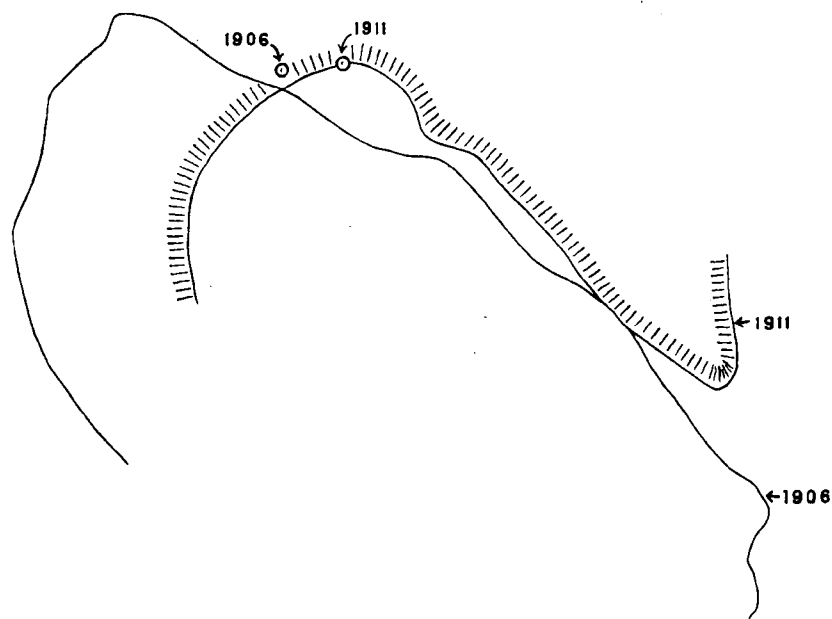
Fig. 2.— HORIZONTAL TRACE OF THE LIP OF THE ICE-CLIFF OF 1911. Superimposed on that of 1906.
