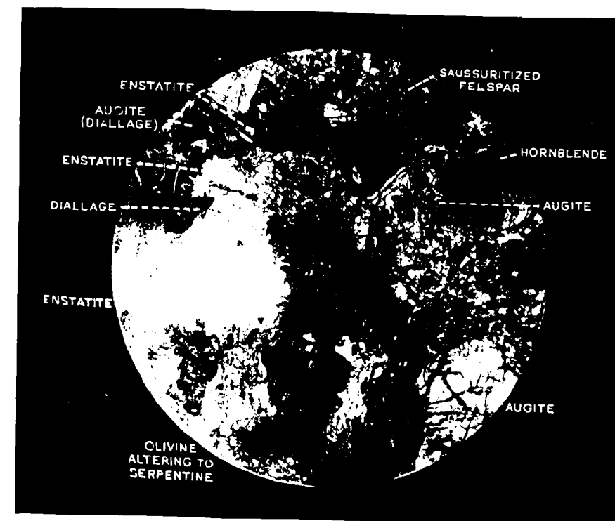
Fig. 2. SAME GABBRO ( \times 10\frac{1}{2} diam. crossed nicols)
