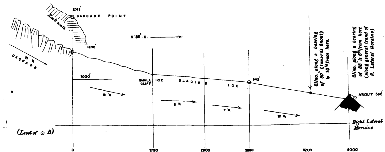
Fig. 7.—POTING GLACIER, 7th. June 1911.
