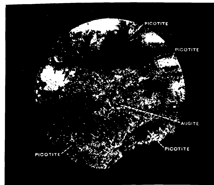
Fig. 2. SERPENTINE ( \times 10\frac{1}{2} diam., crossed nicols.)
