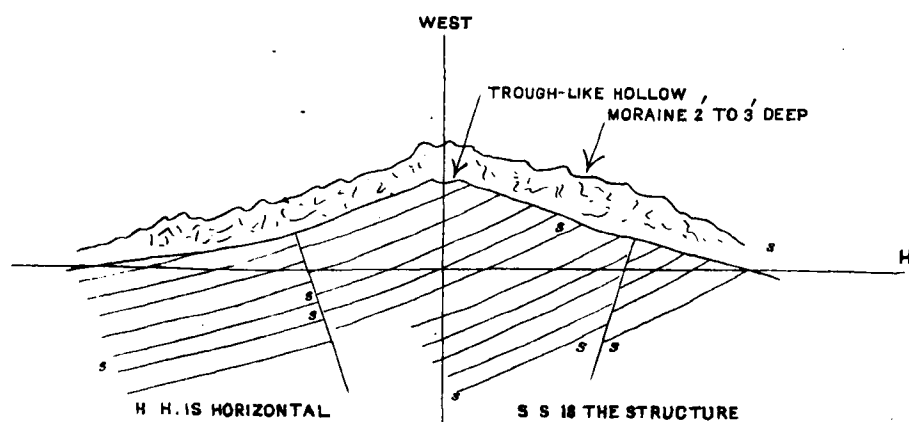
Fig. 10.—TROUGH FAULT IN THE ICE.
