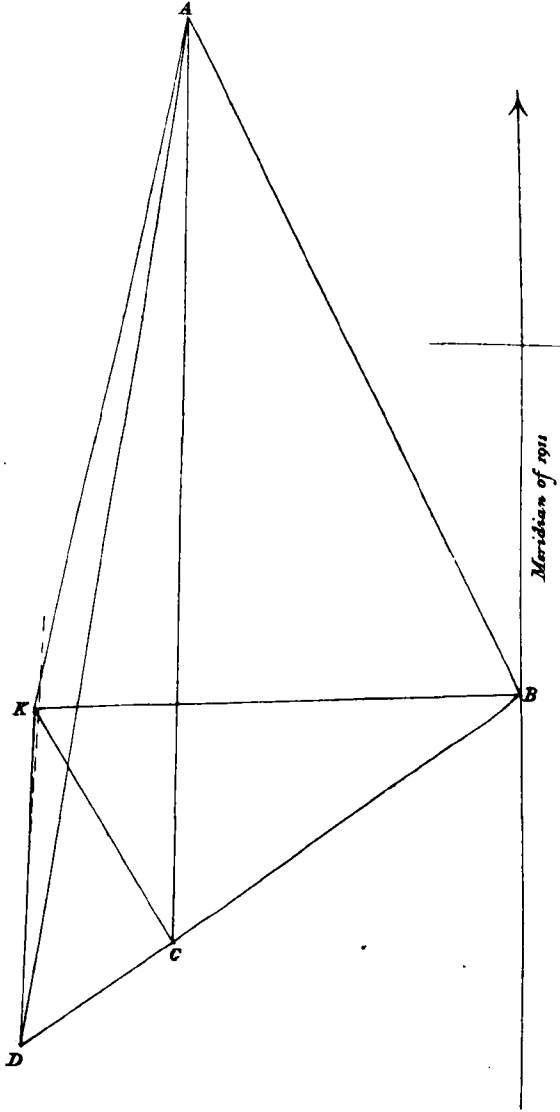
Fig. 13.— DIAGRAM SHEWING THE EXACT PORTION OF K; the Cairn of 1911.
