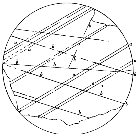
Fig. 1—16'964—Nicols crossed— \times 38 (See p. 201) Calcite showing twinning planes ( a ) and cleavage planes ( b ) both marked out by manganese-ore dust. Where ( a ) shows white there is no manganese-ore.
