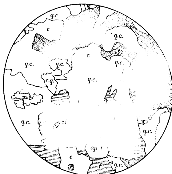
Fig. 2—16 946—Nicols crossed—x 68 (See p. 206) (ap) Apatite. (c) Calcite. (e) Epidote (stippled). (f) Felspar (shaded). (q) Quartz. (q.c.) & (c.q.) Quartz-calcite, & calcite-quartz micropegmatite.
