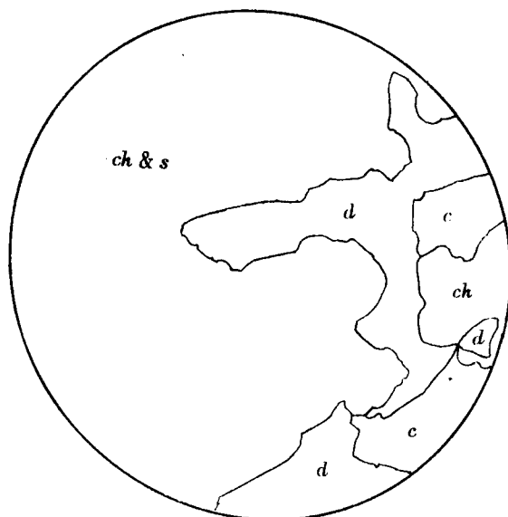
Fig. 1—16 958—Nicols crossed—x 38 (See p. 205) (c) Calcite. (ch) & (s) Chondrodite (ch) veined with serpentine (s). (ch) Chondrodite. (d) Dolomite.
