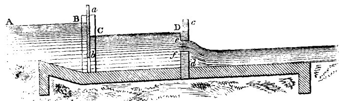
SECTIONAL DIAGRAM OF A PIEDMONTESE OUTLET.
