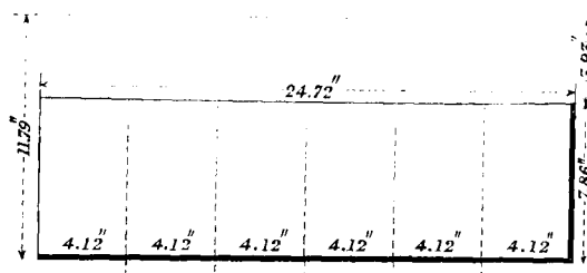
OUTLET FOR 6 WATER-INCHES.
