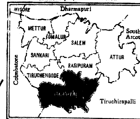
Index Map of Salem District.
