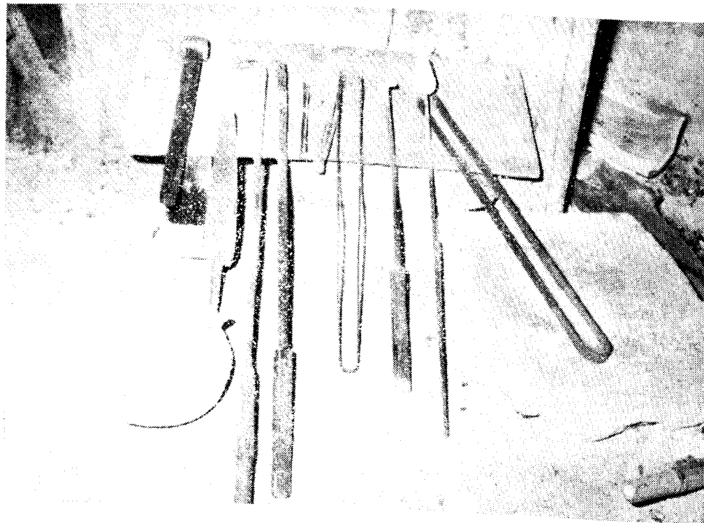
Photograph No. 19 Tools and implements used at Tarapur in manufacturing glass bangles
