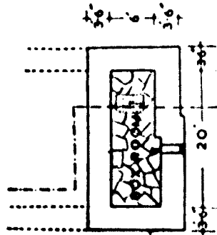
BASEMENT PLAN
