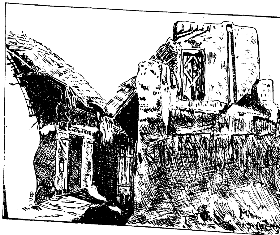
A semi-pucca house in village Barauli, Tahsil Atrauli District Aligarh (West Plain) The front walls of the house are built of burnt bricks and the remaining wall of sun-dried clay bricks. The roofs are built of mango beams covered with burnt bricks and thin mud layer. A portion has a thatch of moonj Grass
