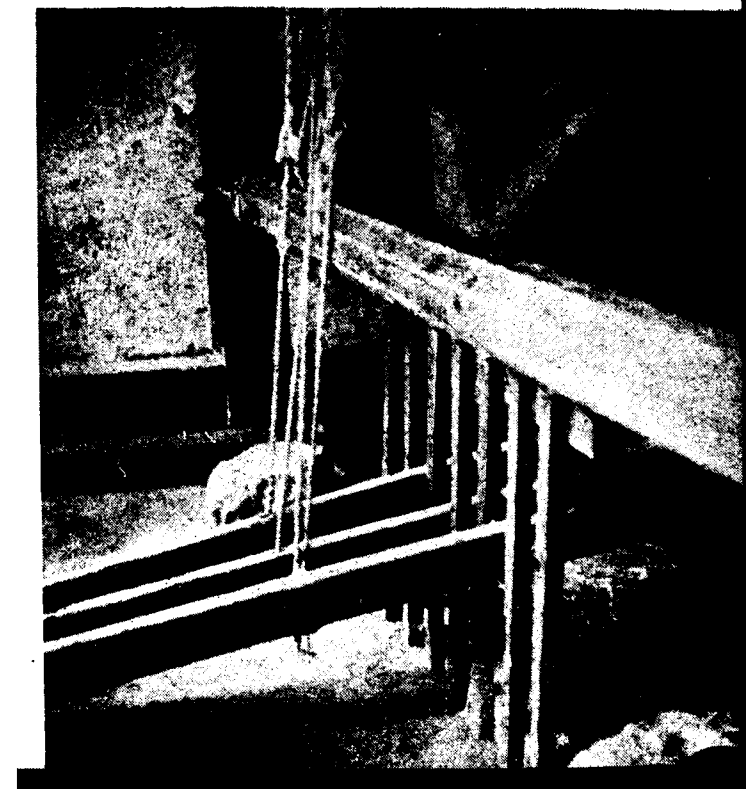
Portions of the loom showing treadles
