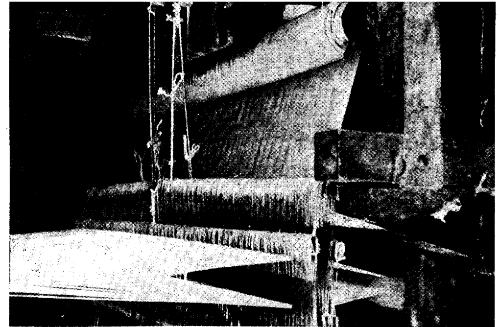
Loom showing the tie-up position of treadles to shafts
