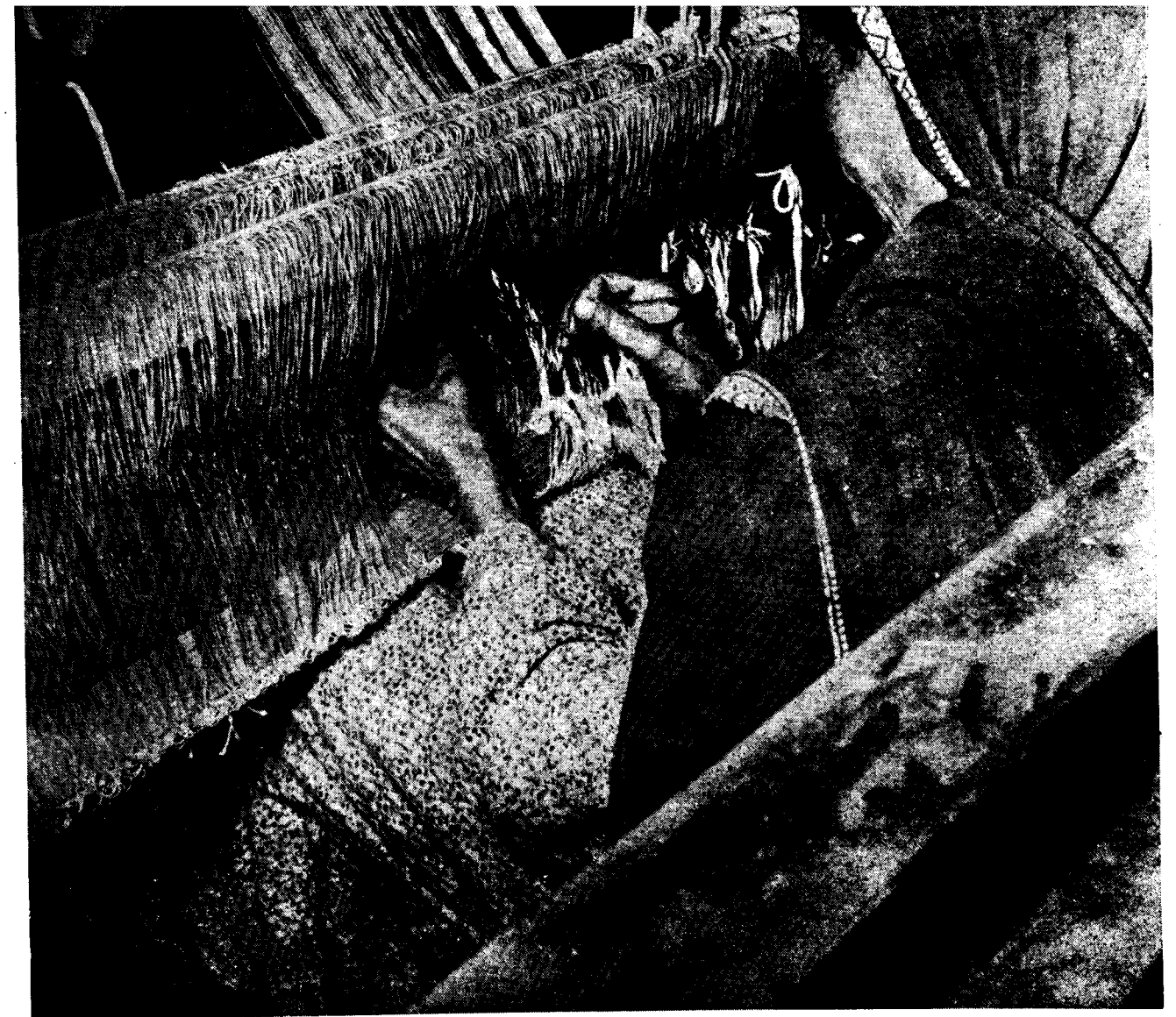
Threading the healds
