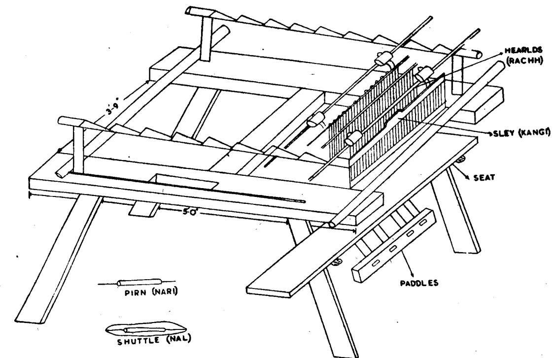
Throw shuttle frame loom
