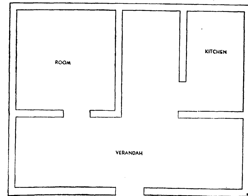
Ground plan of Pallar house (Thanipulinaickenpatti)
