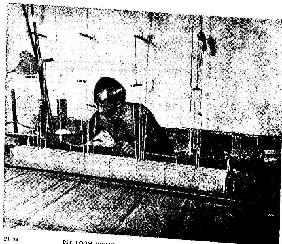
PIT LOOM WEAVING WITH THE THROW SHUTTLE
