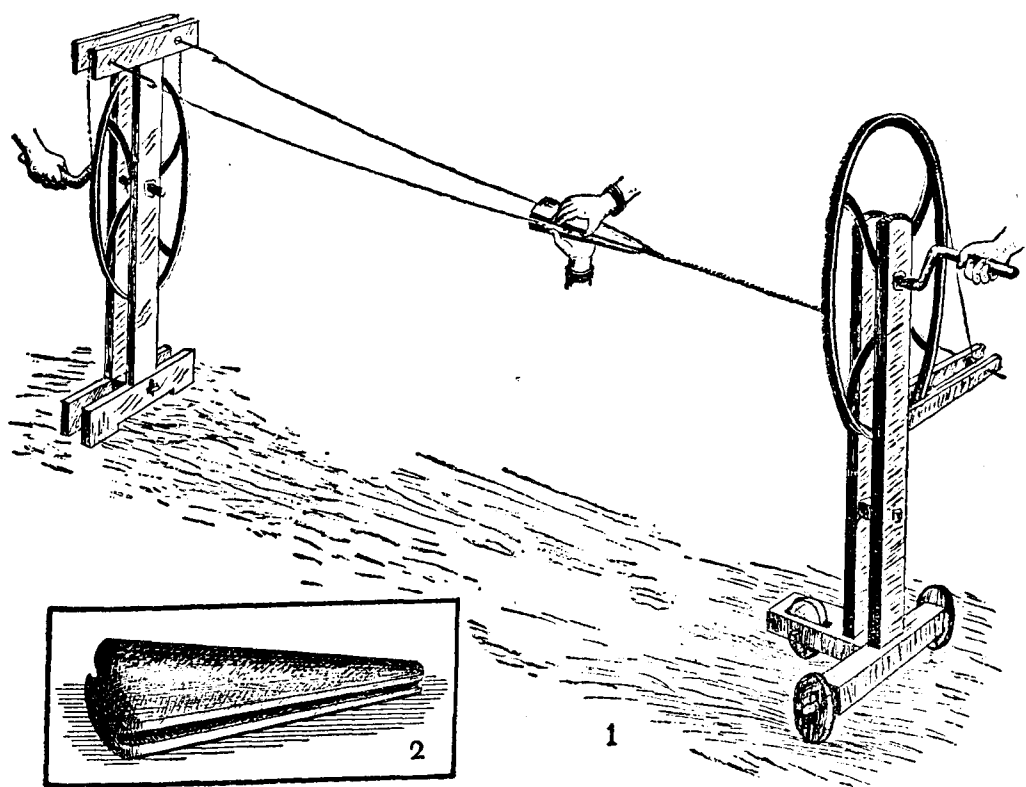
1. DOUBLING THE STRANDS 2. TRIANGULAR PIECE OF WOOD WITH GROOVES
