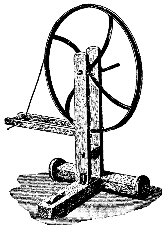
MOVABLE WHEEL FOR DOUBLING THE STRANDS
