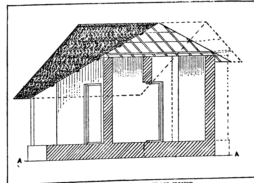
SECTIONAL VIEW OF A POOR CLASS HOUSE
