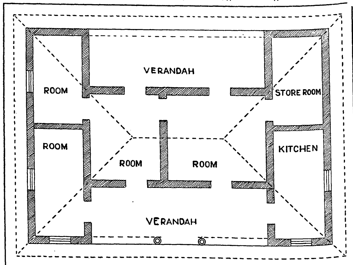
GROUND-PLAN OF A HIGH CLASS HOUSE
