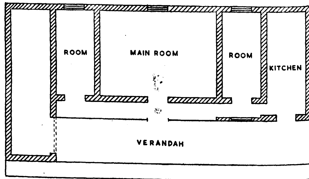
GROUND-PLAN OF A MIDDLE CLASS HOUSE
