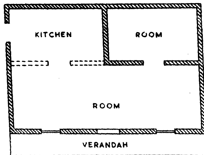
GROUND-PLAN OF A CHALIYAN POOR CLASS HOUSE
