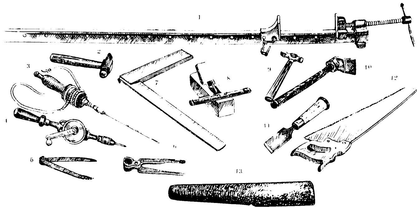
Tools :- 1. Vice; 2 & 9. Hathodi (hammer). 3 & 4. Shardi (drill). 5. Compass; 6. Jambur (nail puller). 7. Katkhuno (right angle); 8. Randho (plane); 10. Vanslo (adze); 11. Farsi (chisel). 12. Karvat (saw); 13. Gotilo (mallet).
