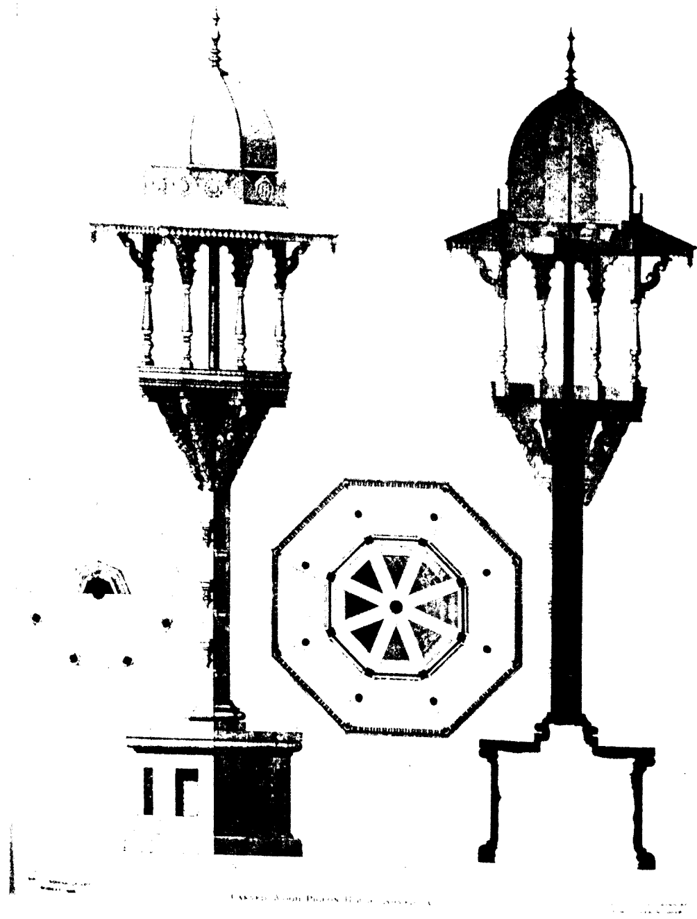
Plan, section and elevation of a pigeon house at Ahmedabad (Reproduced from 'The Journal of Indian Art', 1896.)
