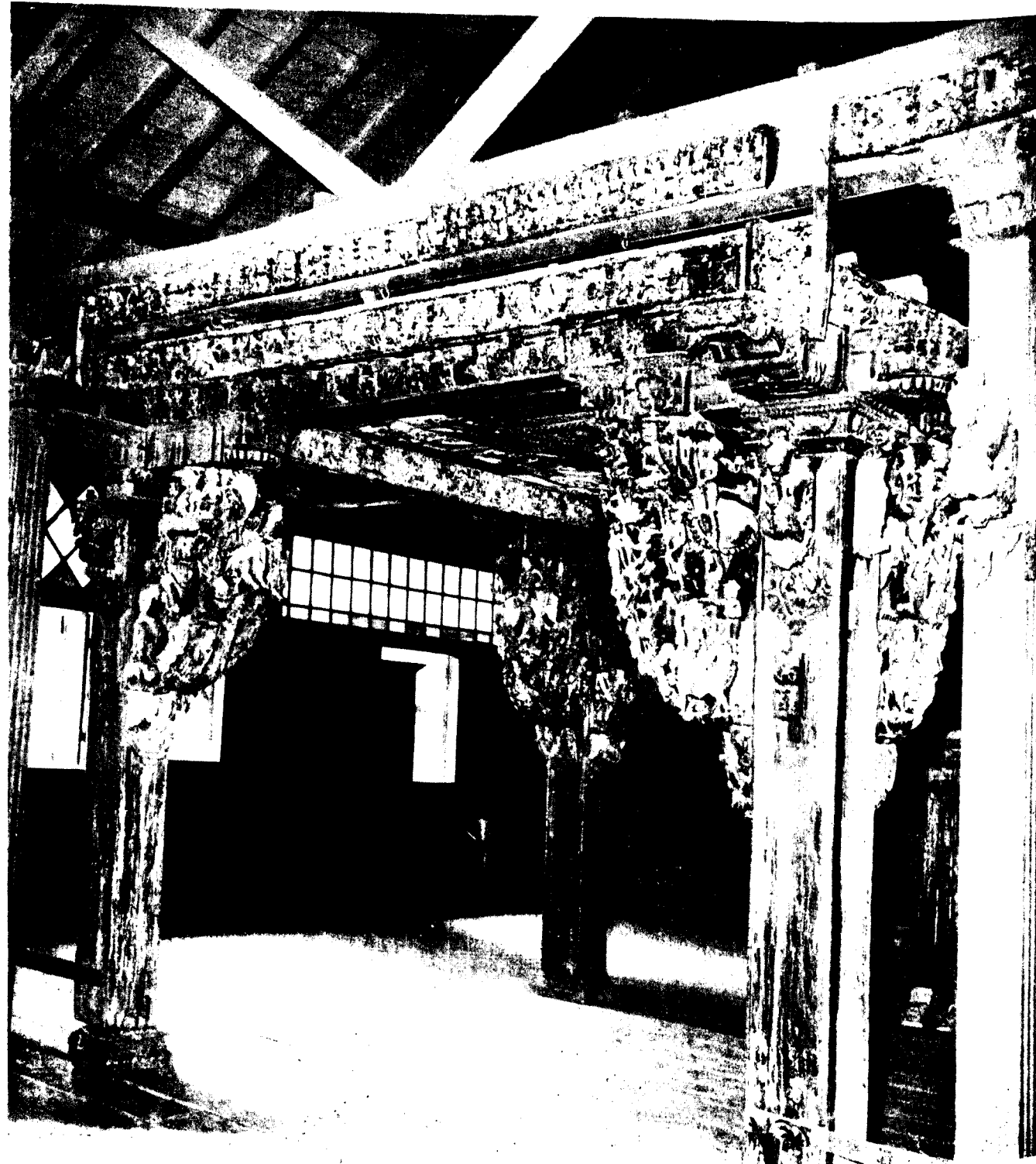
Wooden Mandap of Suparshvanath Temple, reassembled and preserved at Shanttsagar Upashraya, Ahmedabad, after the Temple was rebuilt in stone Mandap 8'-5" square : Height of pillars 7'-2½"
