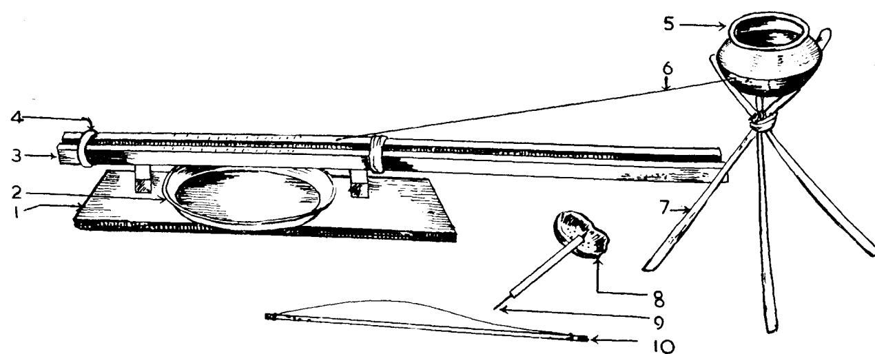
2. Tools in use for drilling
