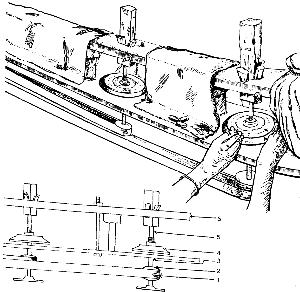
Grinding and smoothing on electrically operated emery wheel
