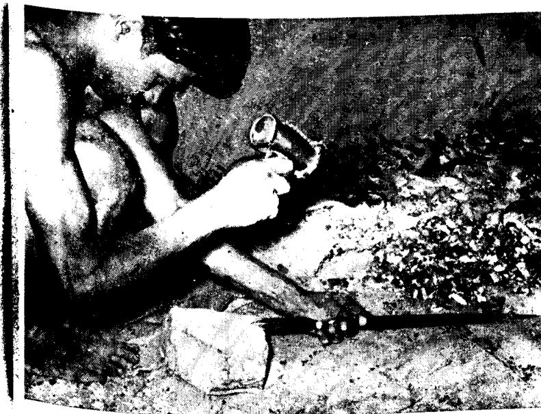
1. Hammering the edge of iron spike
