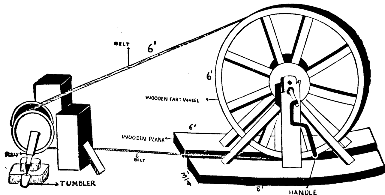
Hand-turning lathe
