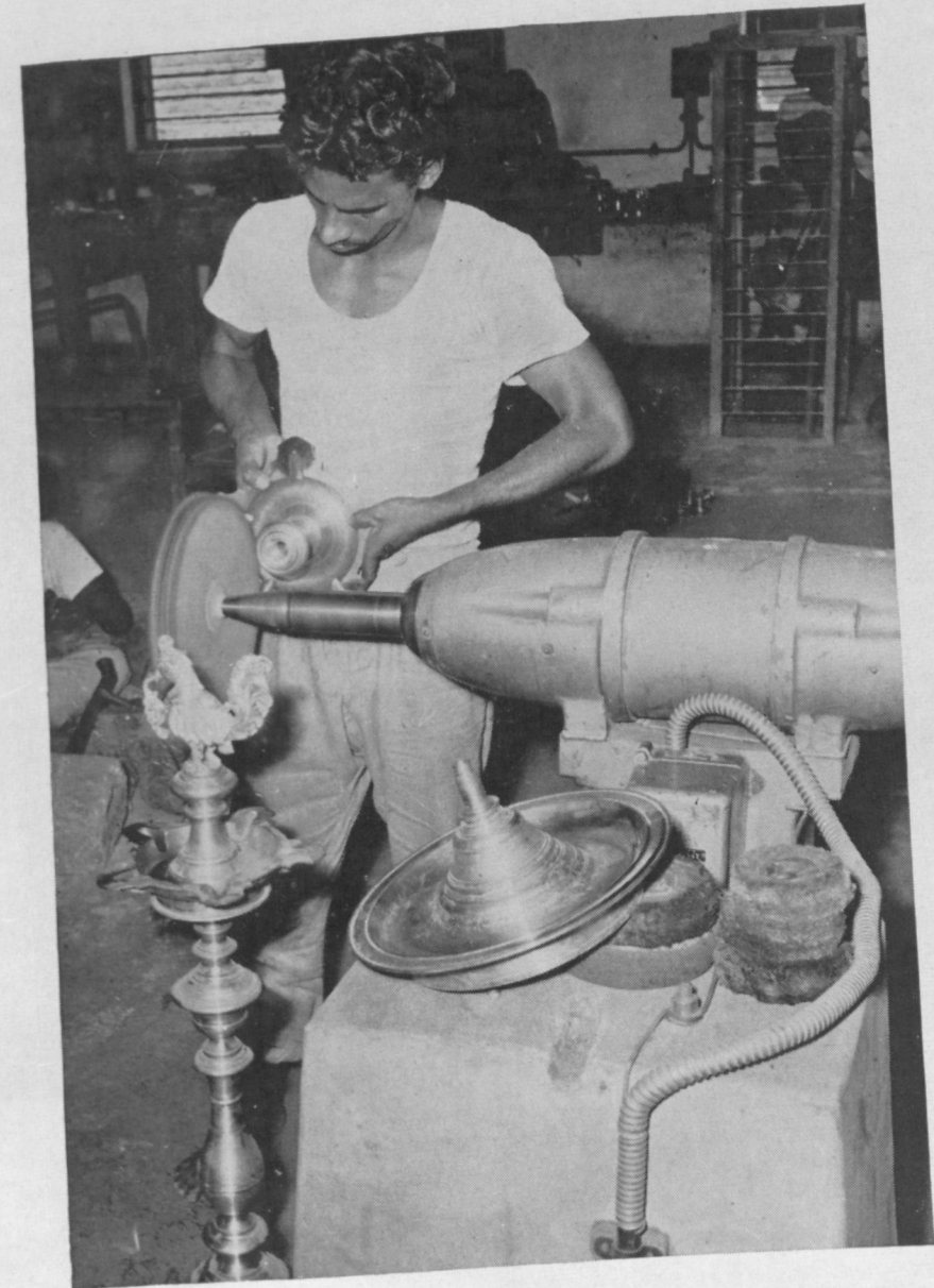
For polishing the various parts of the Kuthuvilakku (Pedestal oil lamp) a lustre soap is put on a buff which is attached to a polishing machine run by an electric motor. The parts under polishing are held firmly with both the craftsman's hands against the buff as the spindle rotates at the high speed of 3,000 R. P. M.
