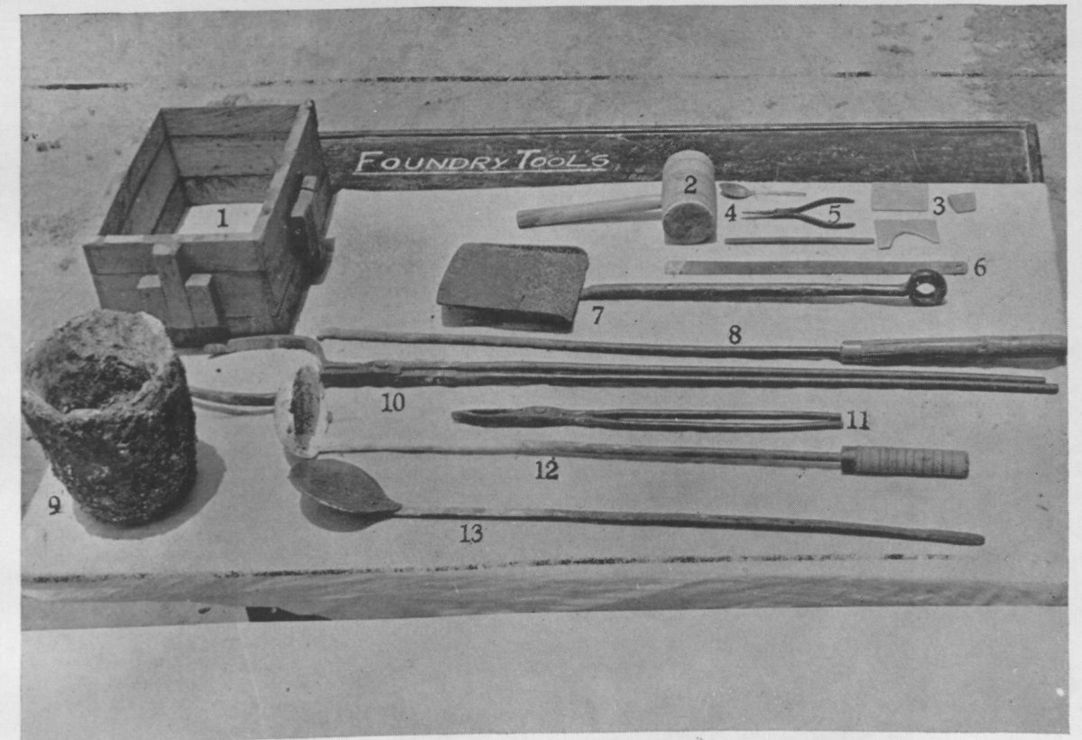
Foundry tools which are essential for moulding and casting
