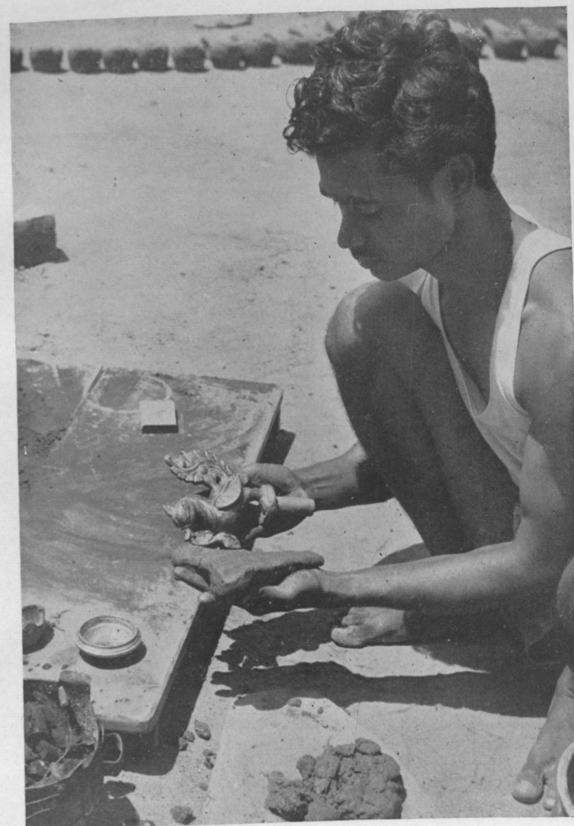
One side of the Hamsa paper weight pattern which has been rubbed with the oil is being plastered with the loam sand.
