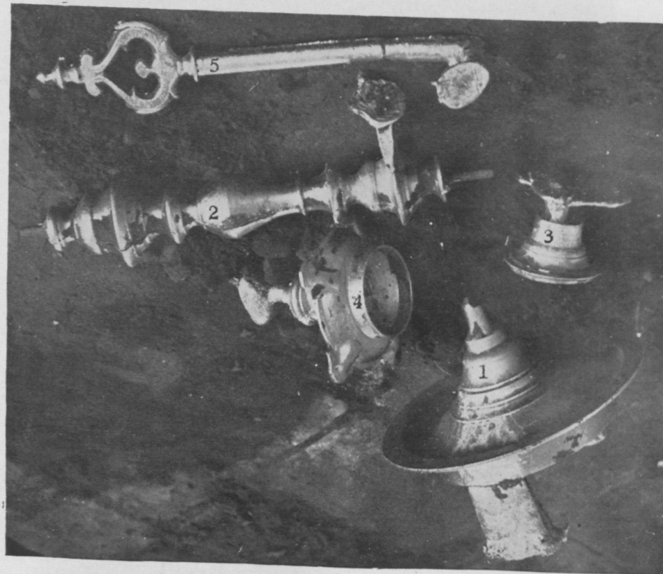
A few minutes after casting the moulds are broken open and the cast pieces of the Kuthuvilakku are taken out wrapped in vandal sand along with the runners attached to them.
