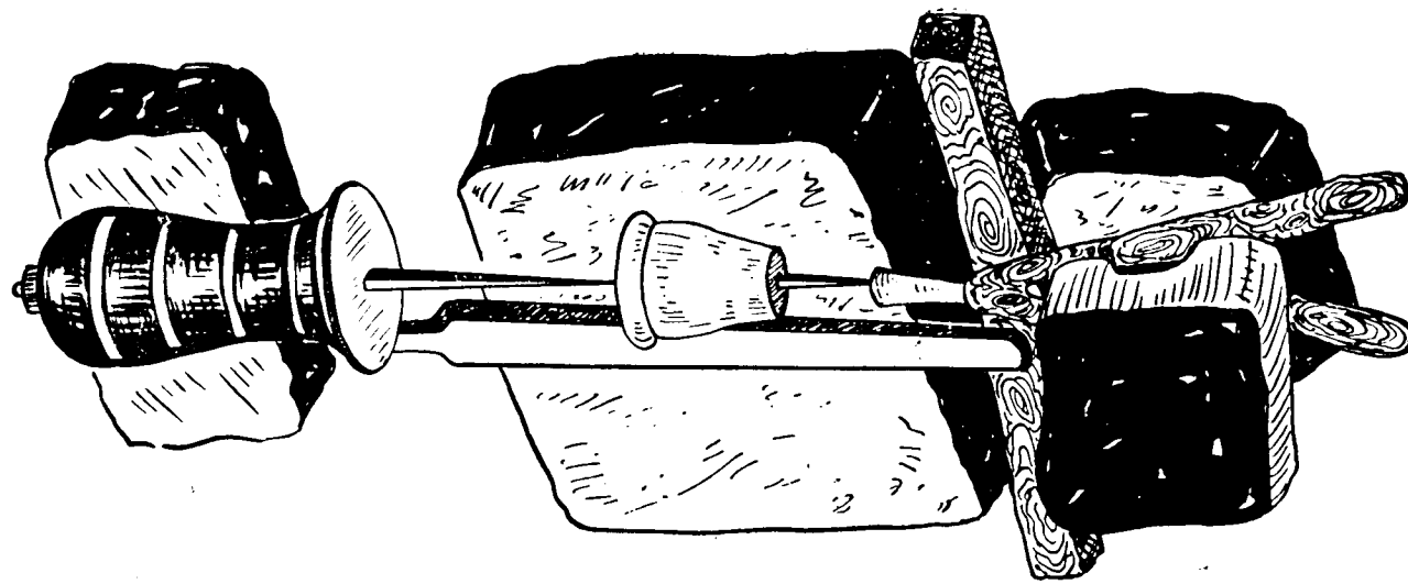
Wax moulding of Mundhiri Kooja on core mandal
