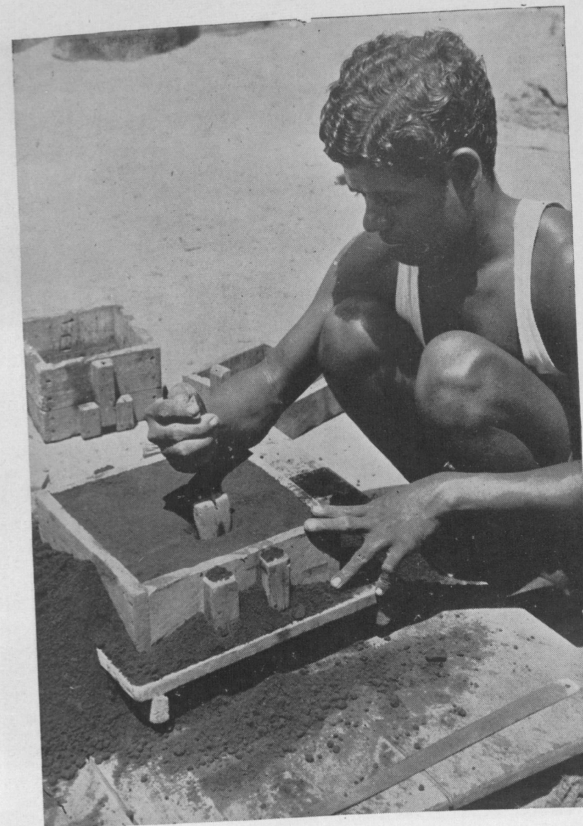
Runner is being pulled out from the hard-packed sand by means of pliers which will form a hollow passage way for an easy flow of the molten metal at the time of casting the base of the Kuthuvilakku.
