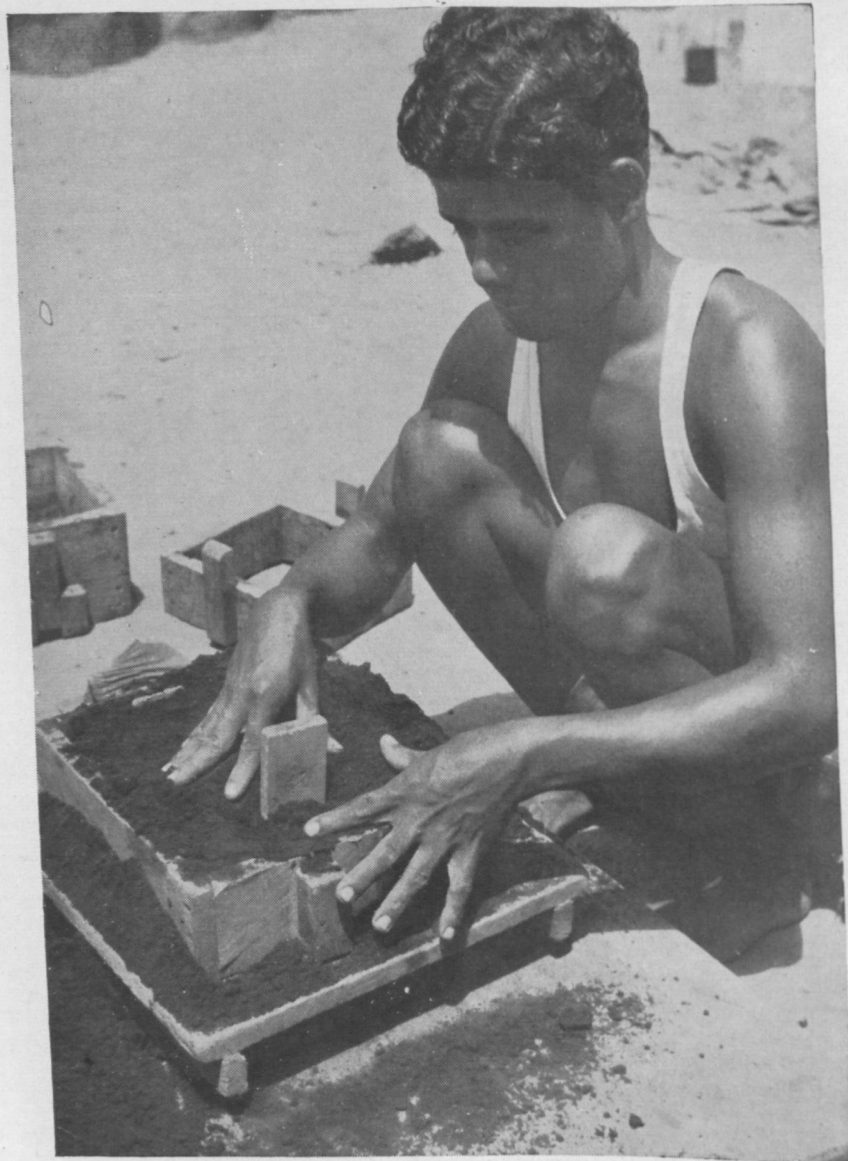
The moulder having placed the metal pattern mould of the base of the Kuthuvilakku (pedestal oil lamp) upside down over a centrally bored hole on a wooden plank and over that laid the bottom moulding box, and having dusted parting sand over the pattern mould, with his left hand he places the runner about an inch away from where the pattern mould of the oil lamp's base lies on wooden plank, what is referred to as the mouth and cavity (that will assist in forming a smooth ingress for the molten metal when casting takes place). With his right hand he will then fill the interior of the box with vandal sand to hold the mouth and cavity in place.
