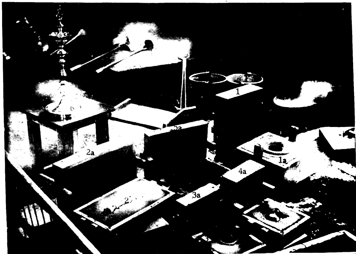
Different moulds of the Kuthuvilakku (pedestal oil lamp) in moulding boxes of various sizes grouped together to indicate the number of boxes required for producing a single Kuthuvilakku.
