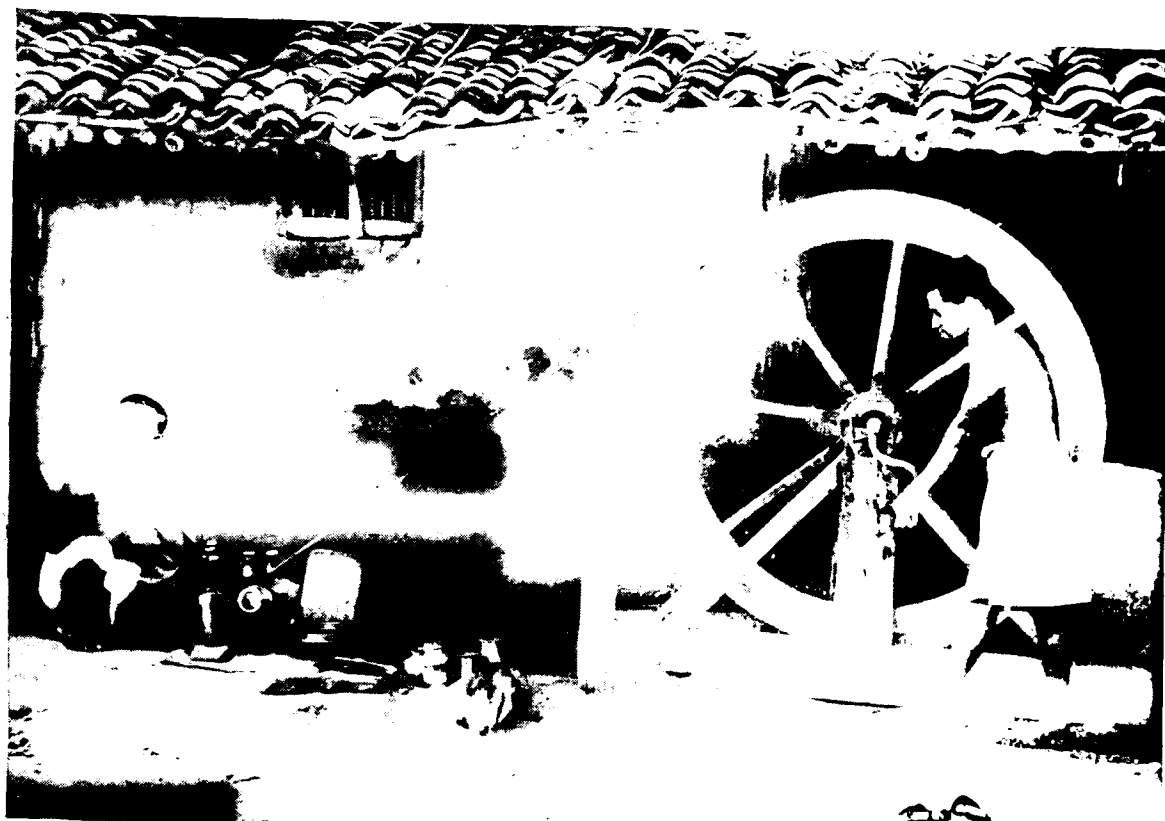
In some of the factories two artisans are at work operating a wooden cart wheel type of turning lathe in order to burnish newly cast milk chembus and other articles, some of which are already burnished and awaiting polishing.
